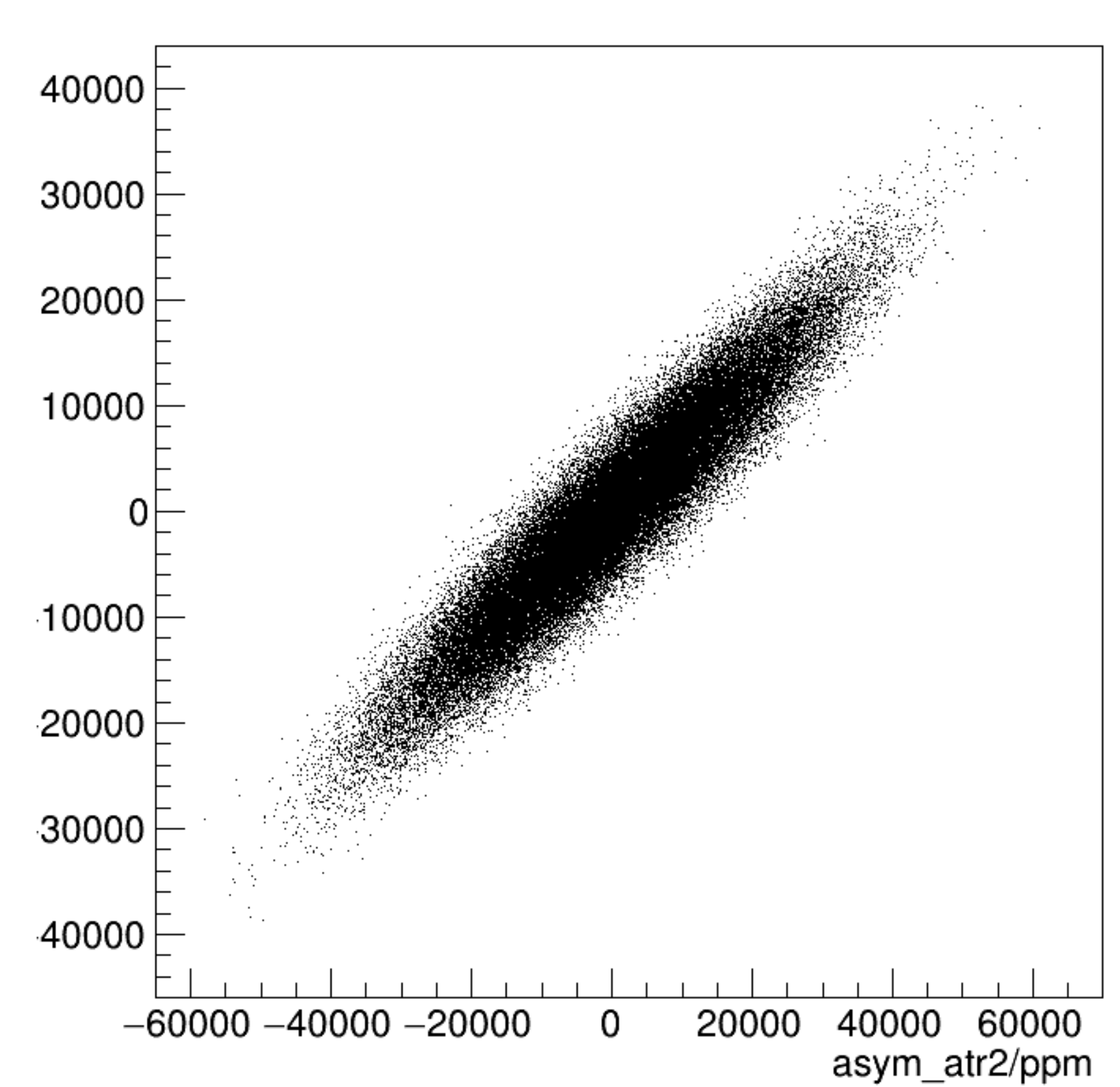
asym_atl2/ppm:asym_atr2/ppm {ok_cut}
