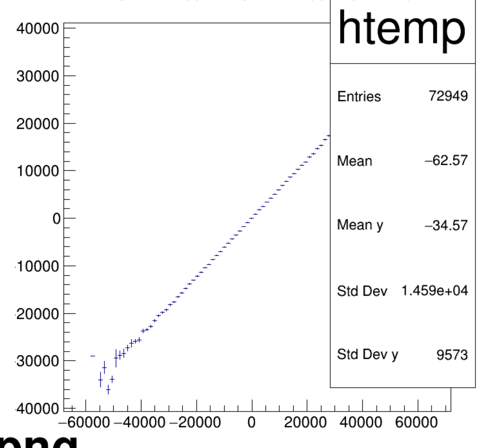
asym_atl2/ppm:asym_atr2/ppm {ok_cut}
