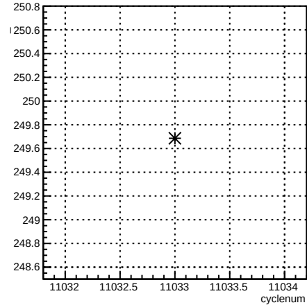
4eX_coil7:cyclenum {run == 8277}
