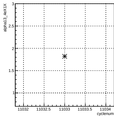
alpha13_4eX1X:cyclenum {run == 8277}
