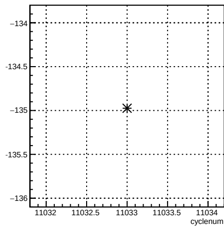
1X_coil1:cyclenum {run == 8277}
