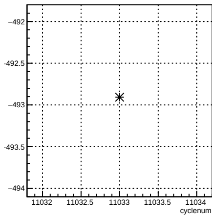
12X_coil7:cyclenum {run == 8277}
