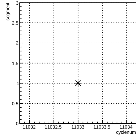
segment:cyclenum {run == 8277}
