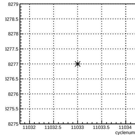
run:cyclenum {run == 8277}
