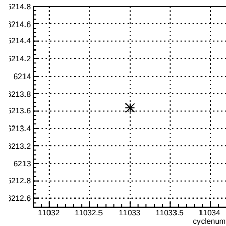
usl_coil4:cyclenum {run == 8277}
