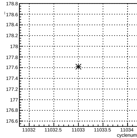
usr_4eX:cyclenum {run == 8277}
