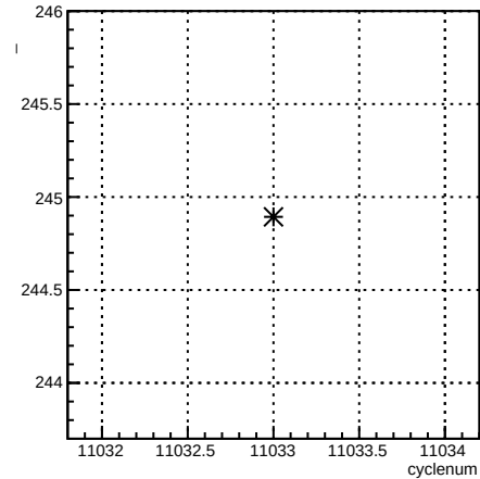
1X_coil7:cyclenum {run == 8277}
