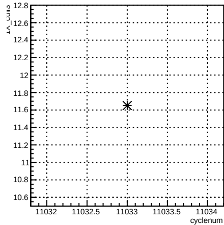
1X_coil3:cyclenum {run == 8277}
