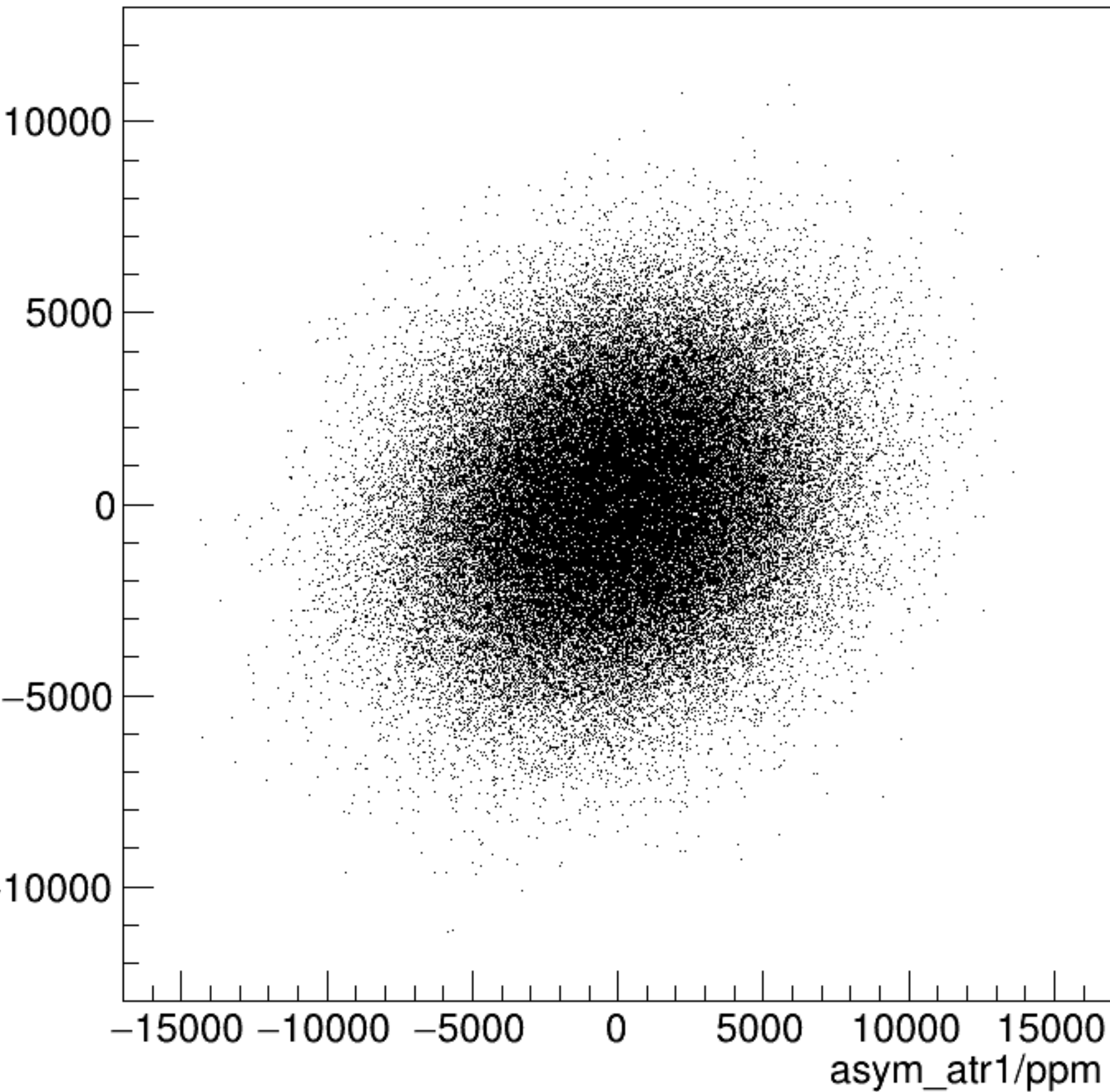
asym_atl1/ppm:asym_atr1/ppm {ok_cut}
