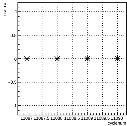
usl_4eY:cyclenum {run == 8299}
