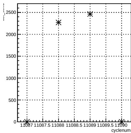
usl_coil3:cyclenum {run == 8299}
