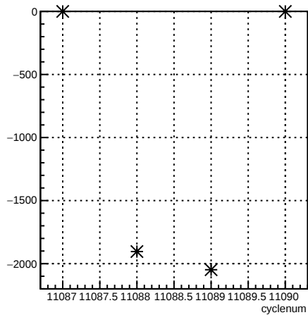
usr_coil3:cyclenum {run == 8299}
