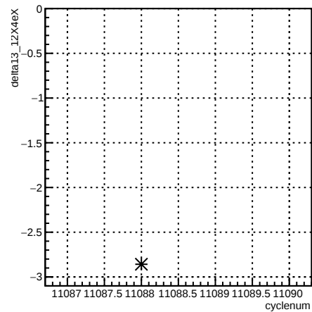
delta13_12X4eX:cyclenum {run == 8299}
