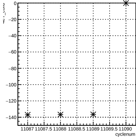
4eY_coil6:cyclenum {run == 8299}
