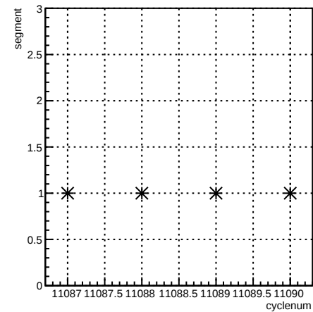
segment:cyclenum {run == 8299}
