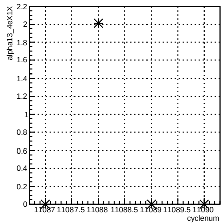
alpha13_4eX1X:cyclenum {run == 8299}
