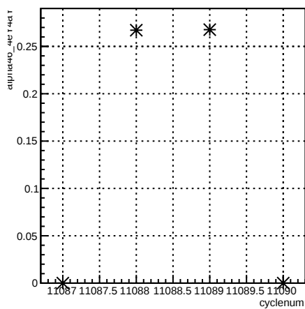
alpha46_4eY4aY:cyclenum {run == 8299}
