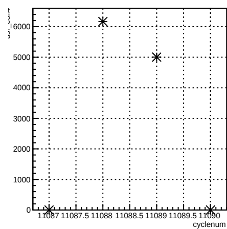
usr_coil4:cyclenum {run == 8299}
