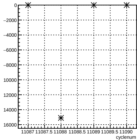
usr_coil1:cyclenum {run == 8299}
