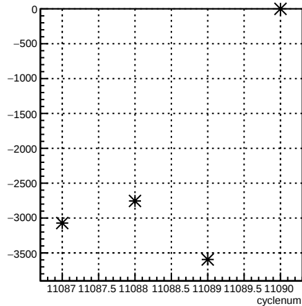
usl_coil6:cyclenum {run == 8299}
