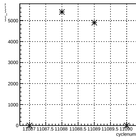
usl_coil4:cyclenum {run == 8299}
