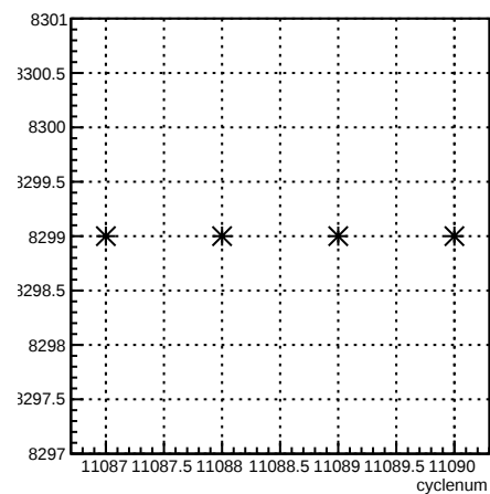
run:cyclenum {run == 8299}
