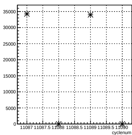
usr_coil7:cyclenum {run == 8299}
