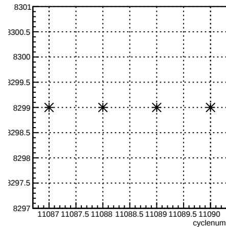
run:cyclenum {run == 8299}
