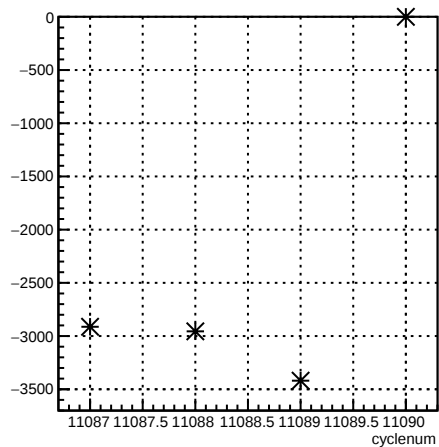
usr_coil6:cyclenum {run == 8299}
