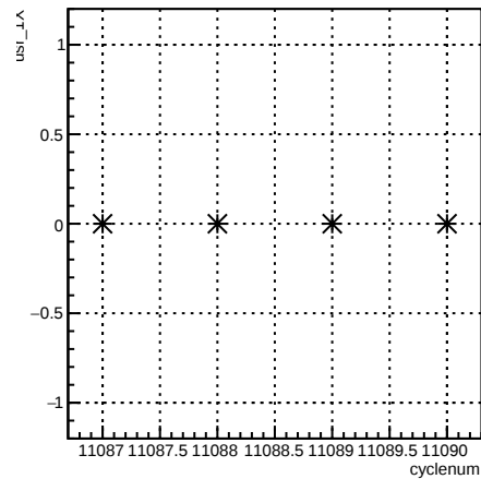
usr_4eY:cyclenum {run == 8299}
