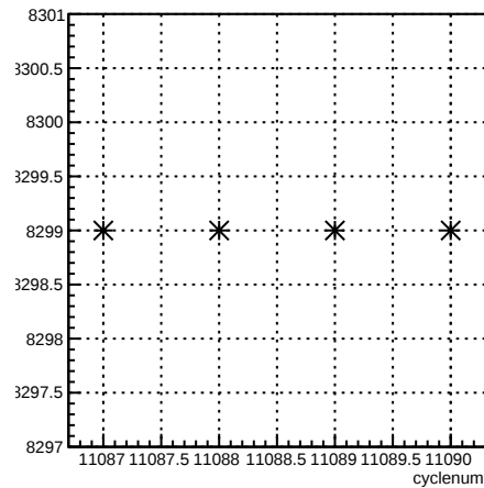
run:cyclenum {run == 8299}
