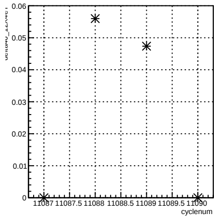
delta46_12X4eY:cyclenum {run == 8299}
