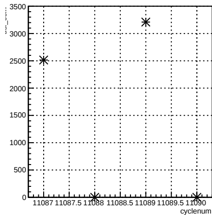
usl_coil7:cyclenum {run == 8299}
