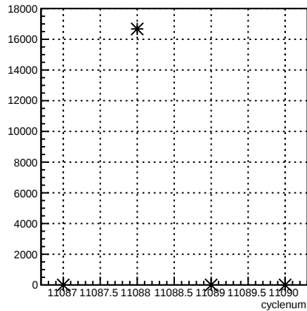
usl_coil1:cyclenum {run == 8299}
