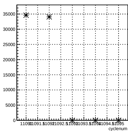
usr_coil7:cyclenum {run == 8300}
