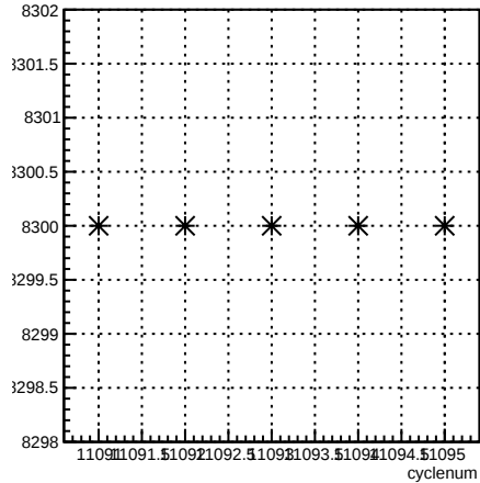
run:cyclenum {run == 8300}
