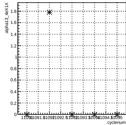
alpha13_4eX1X:cyclenum {run == 8300}
