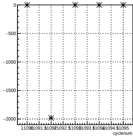
usr_coil3:cyclenum {run == 8300}
