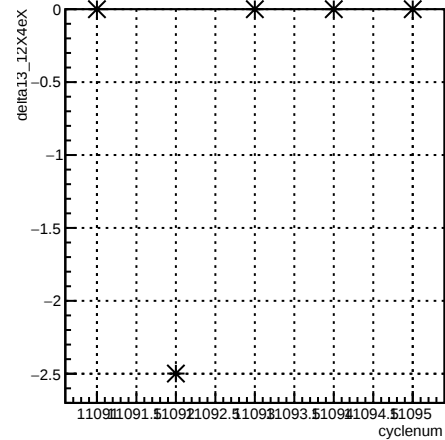
delta13_12X4eX:cyclenum {run == 8300}
