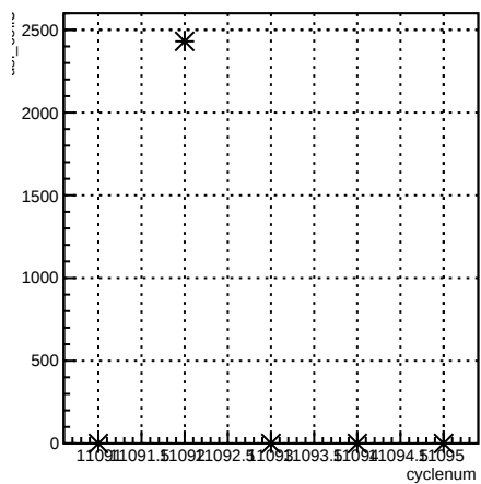
usl_coil3:cyclenum {run == 8300}
