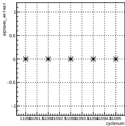
alpha46_4eY4aY:cyclenum {run == 8300}
