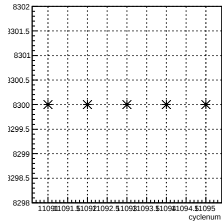
run:cyclenum {run == 8300}
