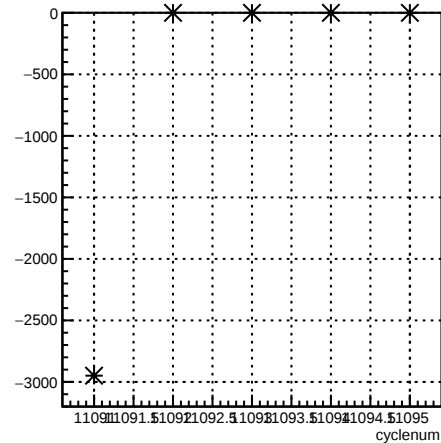
usl_coil6:cyclenum {run == 8300}
