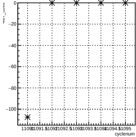
4eY_coil6:cyclenum {run == 8300}
