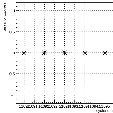
delta46_12X4eY:cyclenum {run == 8300}
