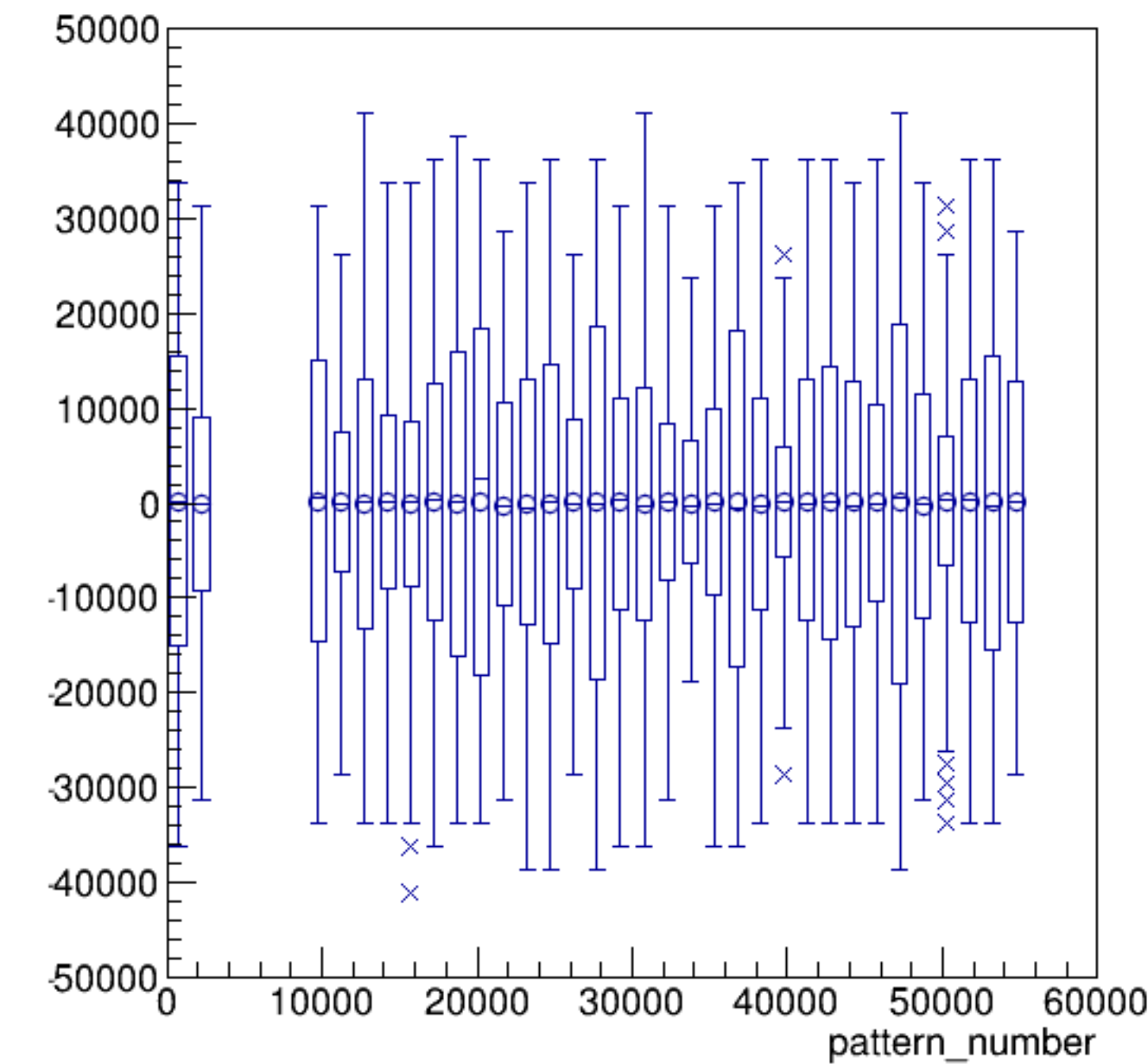
asym_sam4/ppm:pattern_number {ErrorFlag==0}
