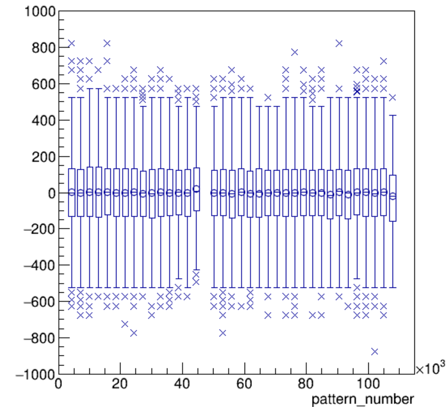
asym_bcm_an_us/ppm:pattern_number {ErrorFlag==0}
