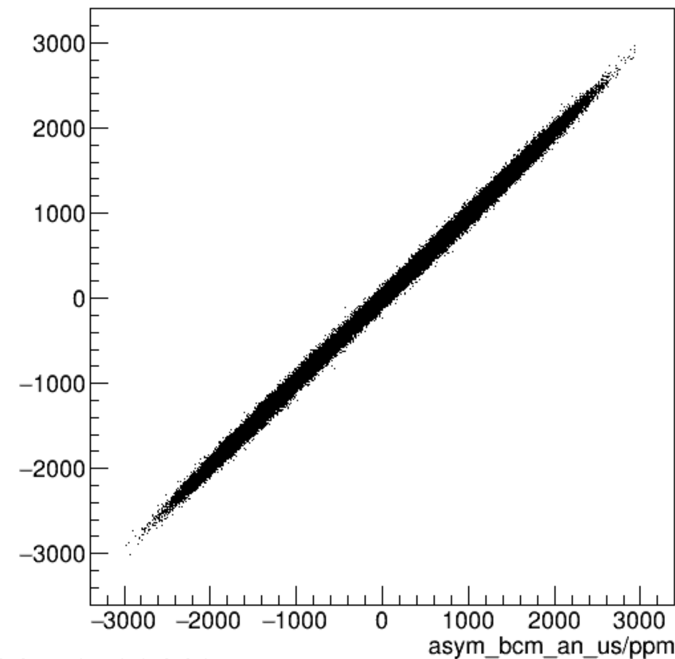
run8303_000_asym_bcm_dg_ds_vs_asym_bcm_an_us_pr.png
