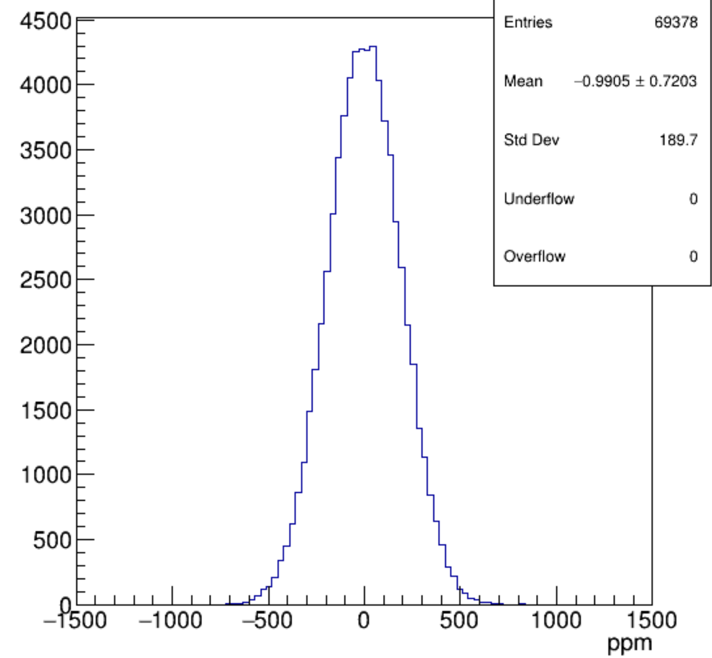
asym_bcm_an_us
