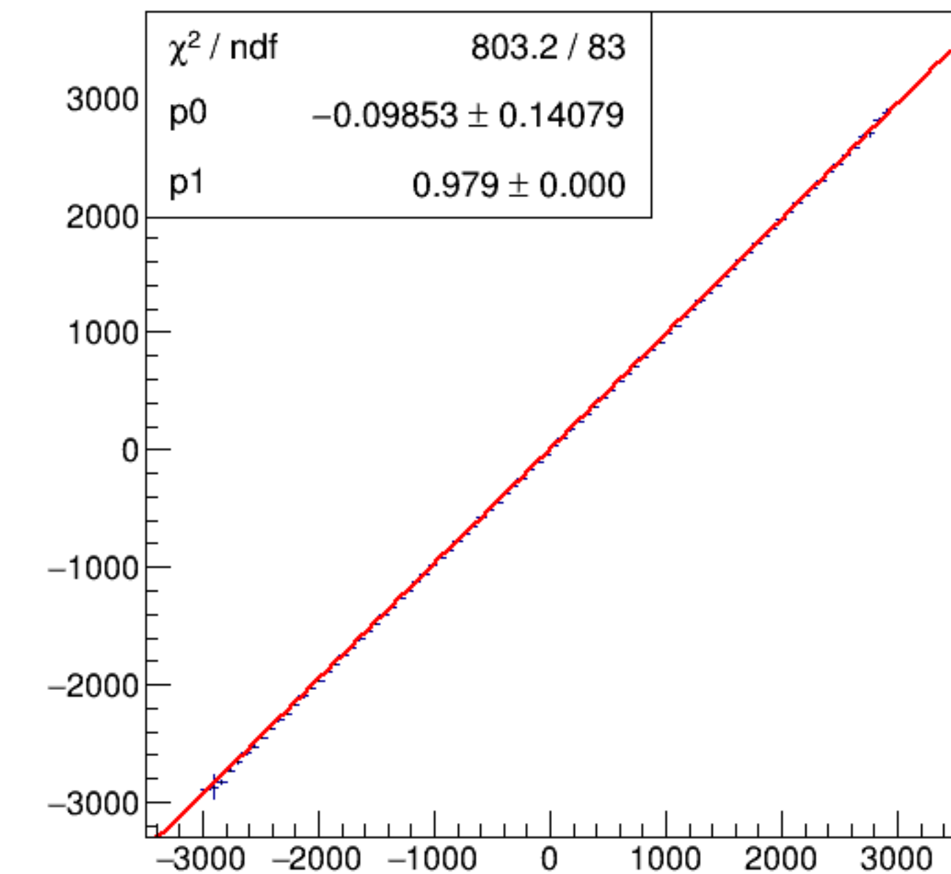
run8303_000_asym_bcm_dg_ds_vs_asym_bcm_an_us_pr.png
