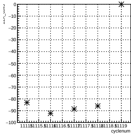
12X_coil3:cyclenum {run == 8305}
