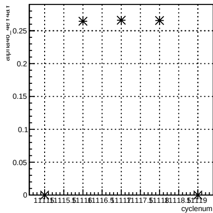
alpha46_4eY4aY:cyclenum {run == 8305}
