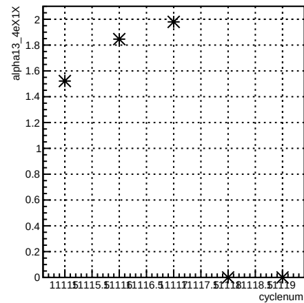
alpha13_4eX1X:cyclenum {run == 8305}
