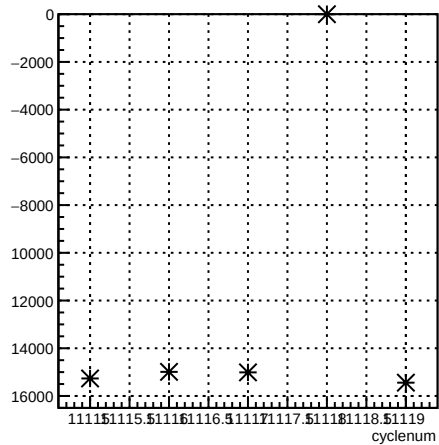
usr_coil1:cyclenum {run == 8305}
