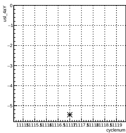
usl_4aY:cyclenum {run == 8305}
