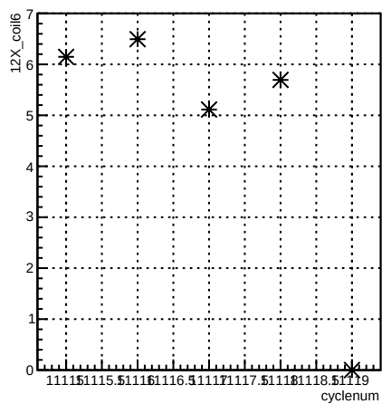
12X_coil6:cyclenum {run == 8305}
