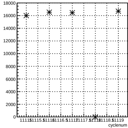
usl_coil1:cyclenum {run == 8305}
