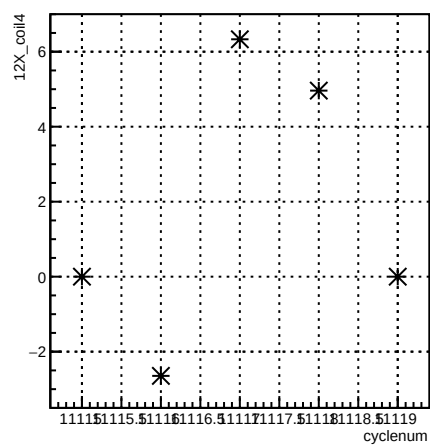
12X_coil4:cyclenum {run == 8305}
