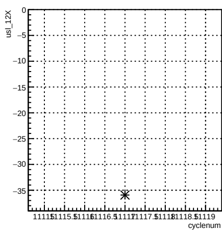
usl_12X:cyclenum {run == 8305}
