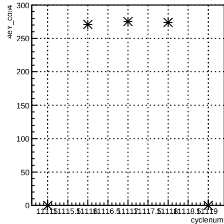
4eY_coil4:cyclenum {run == 8305}
