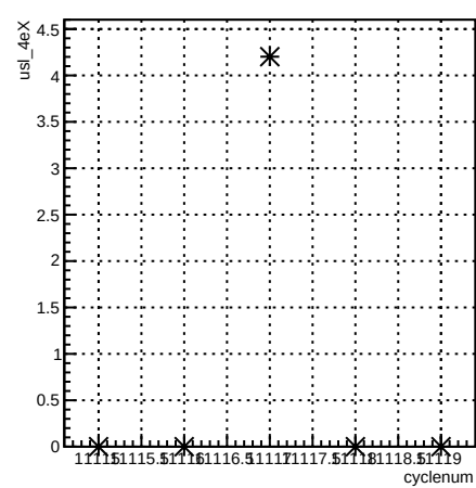
usl_4eX:cyclenum {run == 8305}
