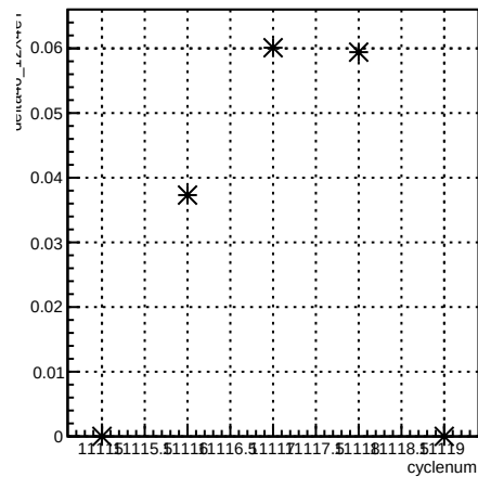
delta46_12X4eY:cyclenum {run == 8305}
