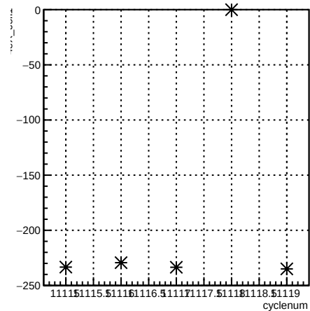
4eX_coil1:cyclenum {run == 8305}
