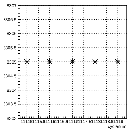
run:cyclenum {run == 8305}
