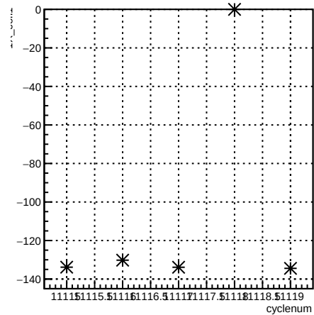
1X_coil1:cyclenum {run == 8305}
