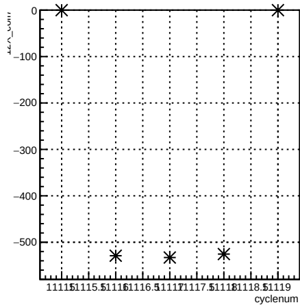
12X_coil7:cyclenum {run == 8305}
