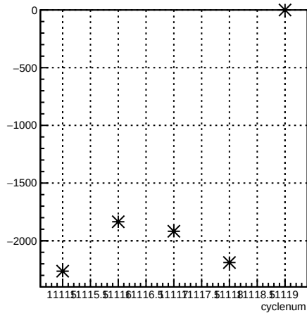
usr_coil3:cyclenum {run == 8305}
