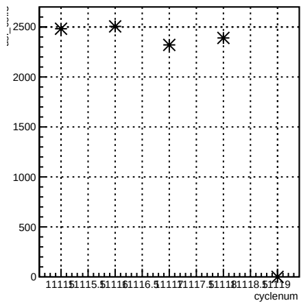
usl_coil3:cyclenum {run == 8305}
