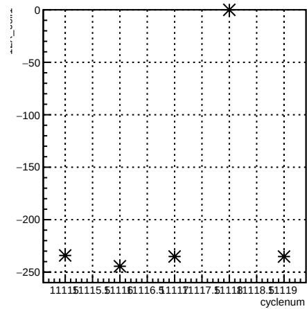
12X_coil1:cyclenum {run == 8305}
