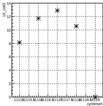
1X_coil3:cyclenum {run == 8305}
