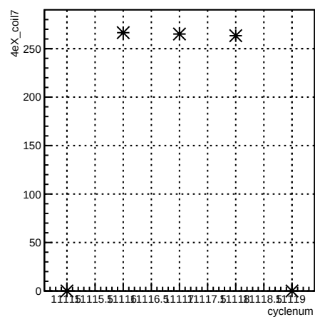
4eX_coil7:cyclenum {run == 8305}
