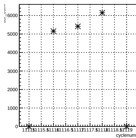
usr_coil4:cyclenum {run == 8305}
