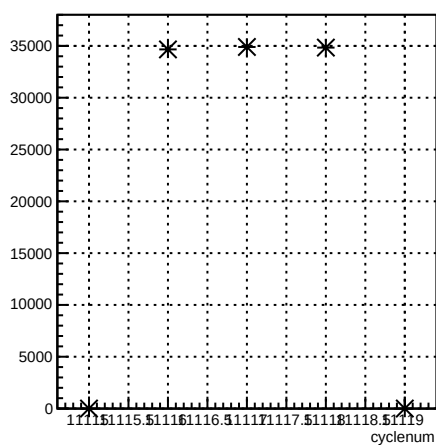
usr_coil7:cyclenum {run == 8305}
