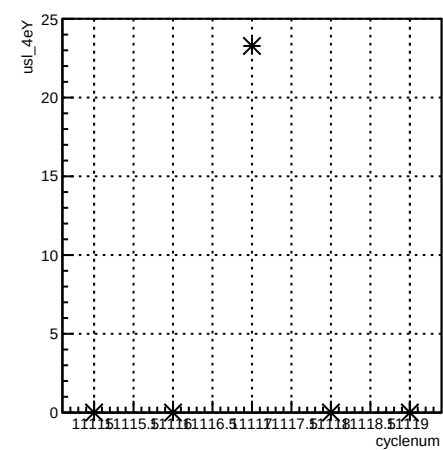
usl_4eY:cyclenum {run == 8305}
