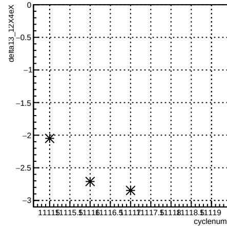
delta13_12X4eX:cyclenum {run == 8305}
