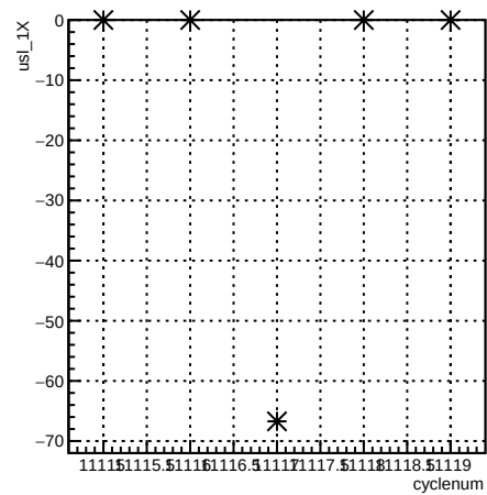
usl_1X:cyclenum {run == 8305}
