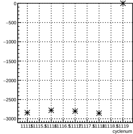
usl_coil6:cyclenum {run == 8305}
