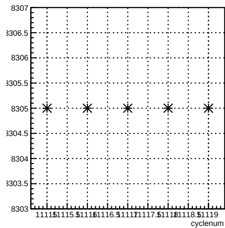
run:cyclenum {run == 8305}
