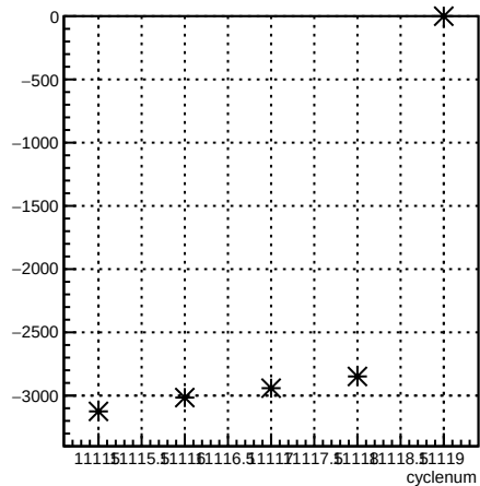
usr_coil6:cyclenum {run == 8305}
