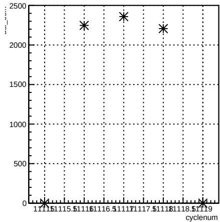
usl_coil7:cyclenum {run == 8305}
