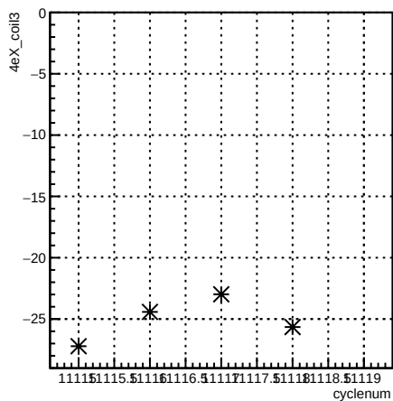
4eX_coil3:cyclenum {run == 8305}
