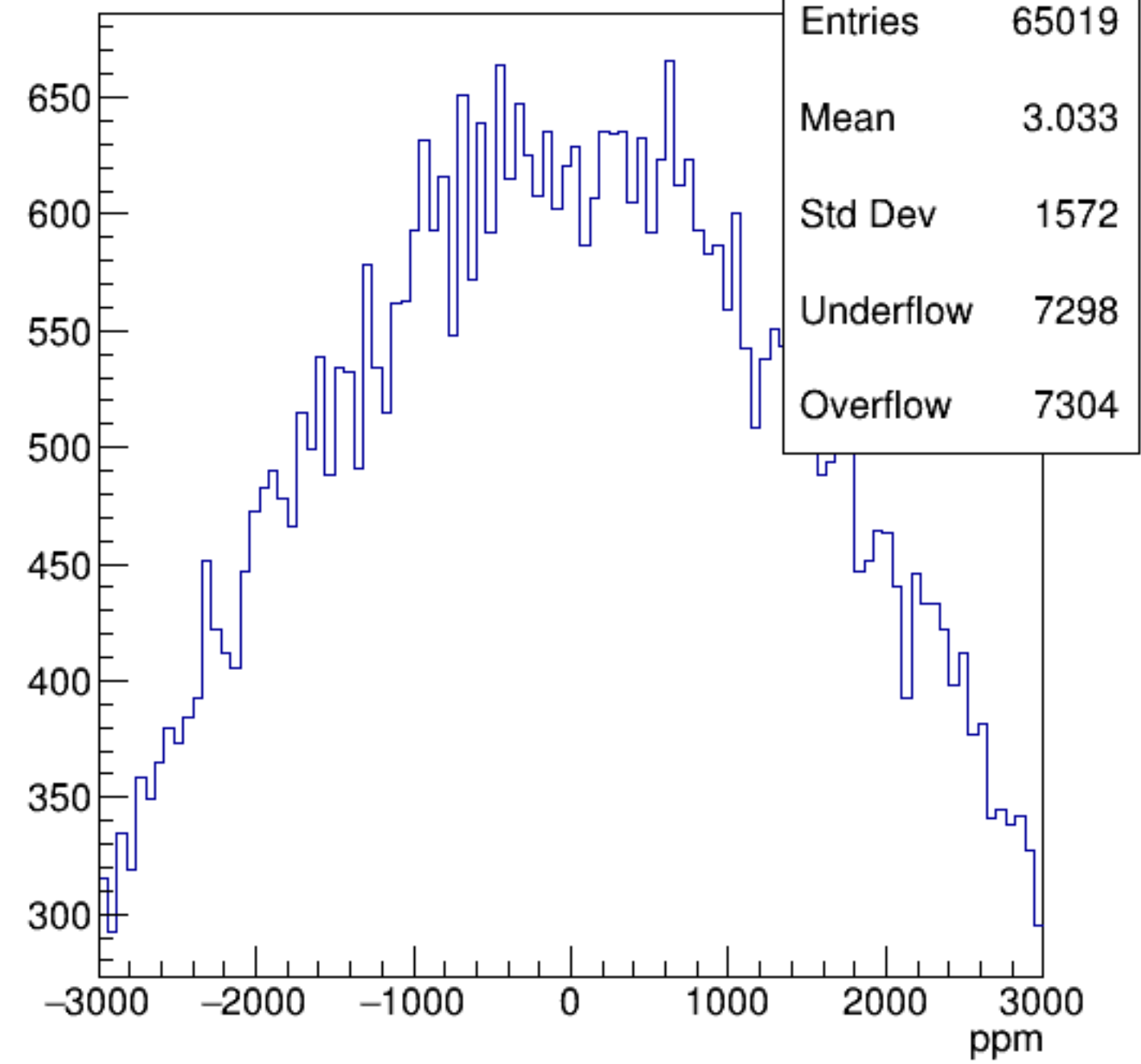
asym_atl1
