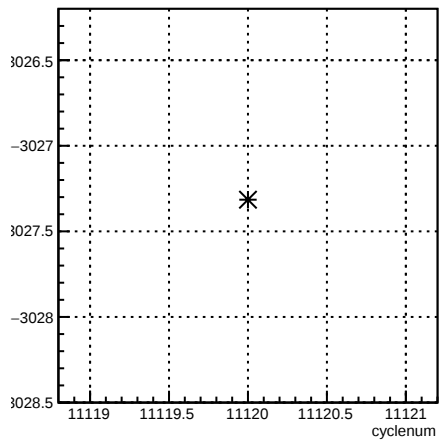
usr_coil6:cyclenum {run == 8306}
