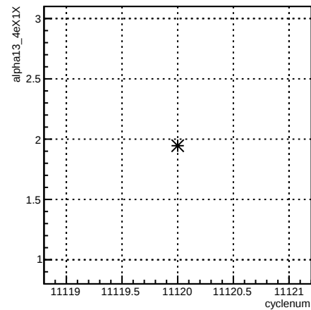
alpha13_4eX1X:cyclenum {run == 8306}
