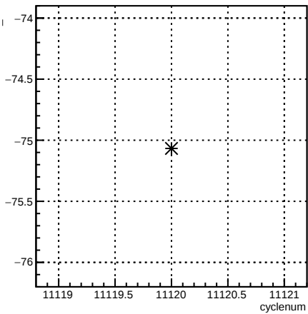
usl_4eY:cyclenum {run == 8306}
