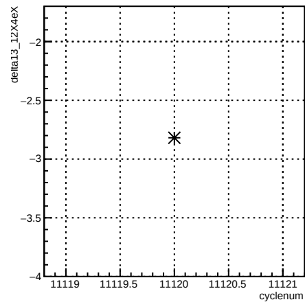
delta13_12X4eX:cyclenum {run == 8306}
