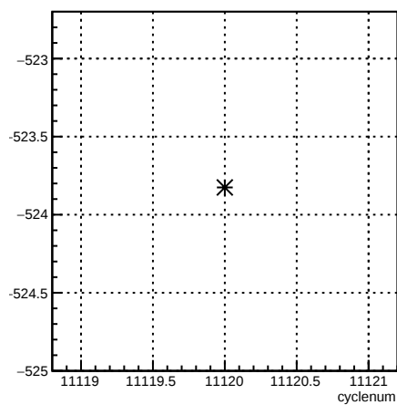
12X_coil7:cyclenum {run == 8306}
