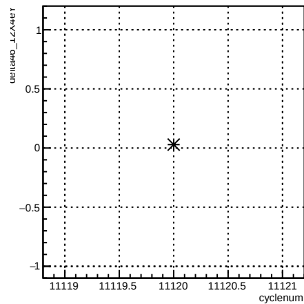
delta46_12X4eY:cyclenum {run == 8306}
