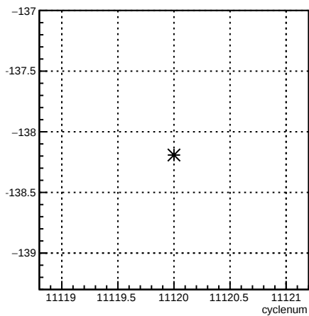
4eY_coil6:cyclenum {run == 8306}
