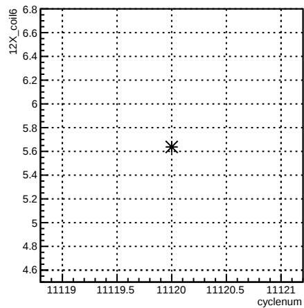
12X_coil6:cyclenum {run == 8306}
