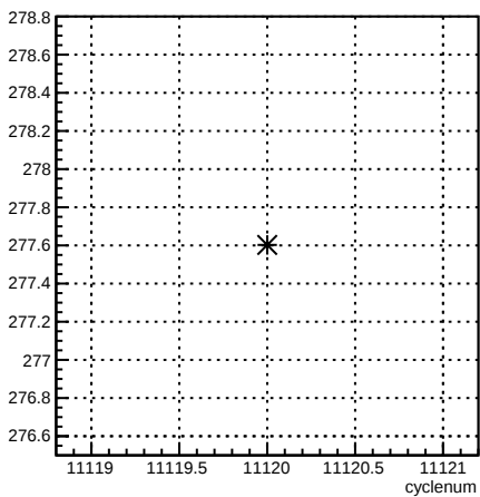
4eY_coil4:cyclenum {run == 8306}
