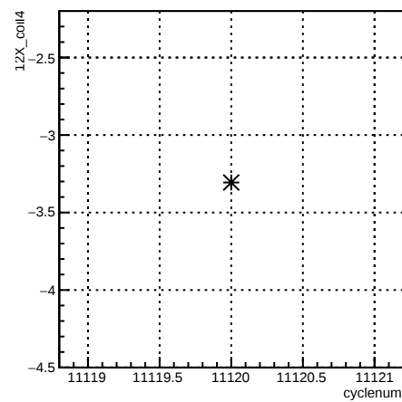
12X_coil4:cyclenum {run == 8306}
