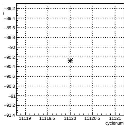
12X_coil3:cyclenum {run == 8306}
