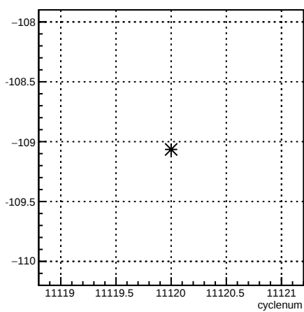
4aY_coil6:cyclenum {run == 8306}
