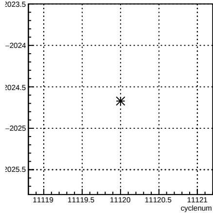
usr_coil7:cyclenum {run == 8306}
