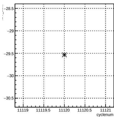
4eY_coil7:cyclenum {run == 8306}
