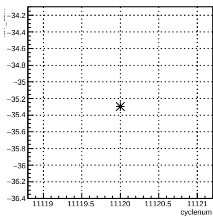
4aY_coil7:cyclenum {run == 8306}
