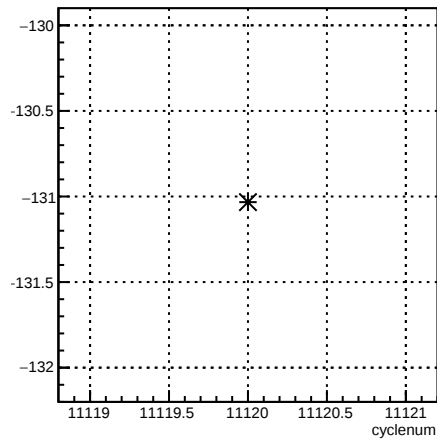
4eX_coil1:cyclenum {run == 8306}
