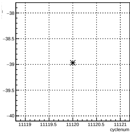
usr_12X:cyclenum {run == 8306}
