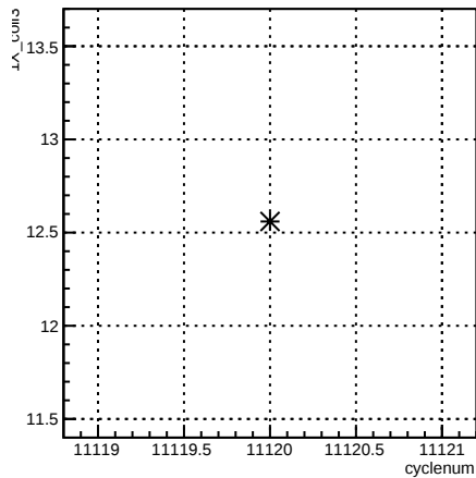
4eX_coil3:cyclenum {run == 8306}
