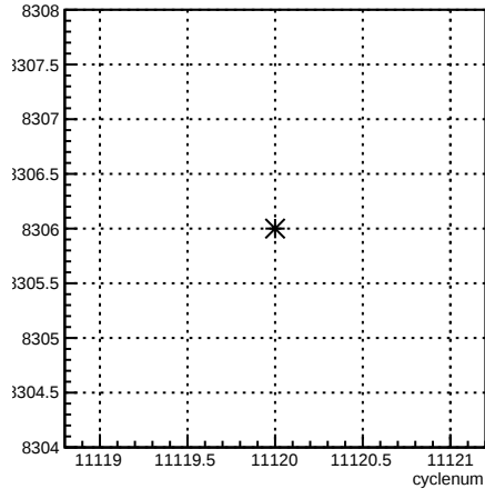
run:cyclenum {run == 8306}
