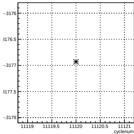
usl_coil6:cyclenum {run == 8306}
