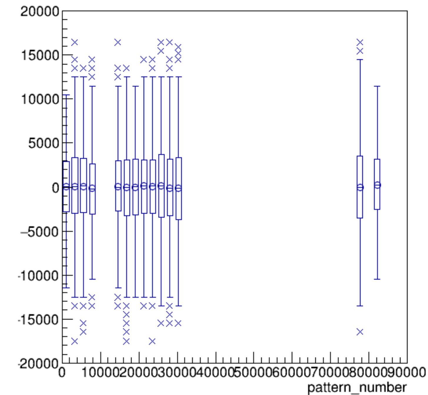
asym_sam4/ppm:pattern_number {ErrorFlag==0}
