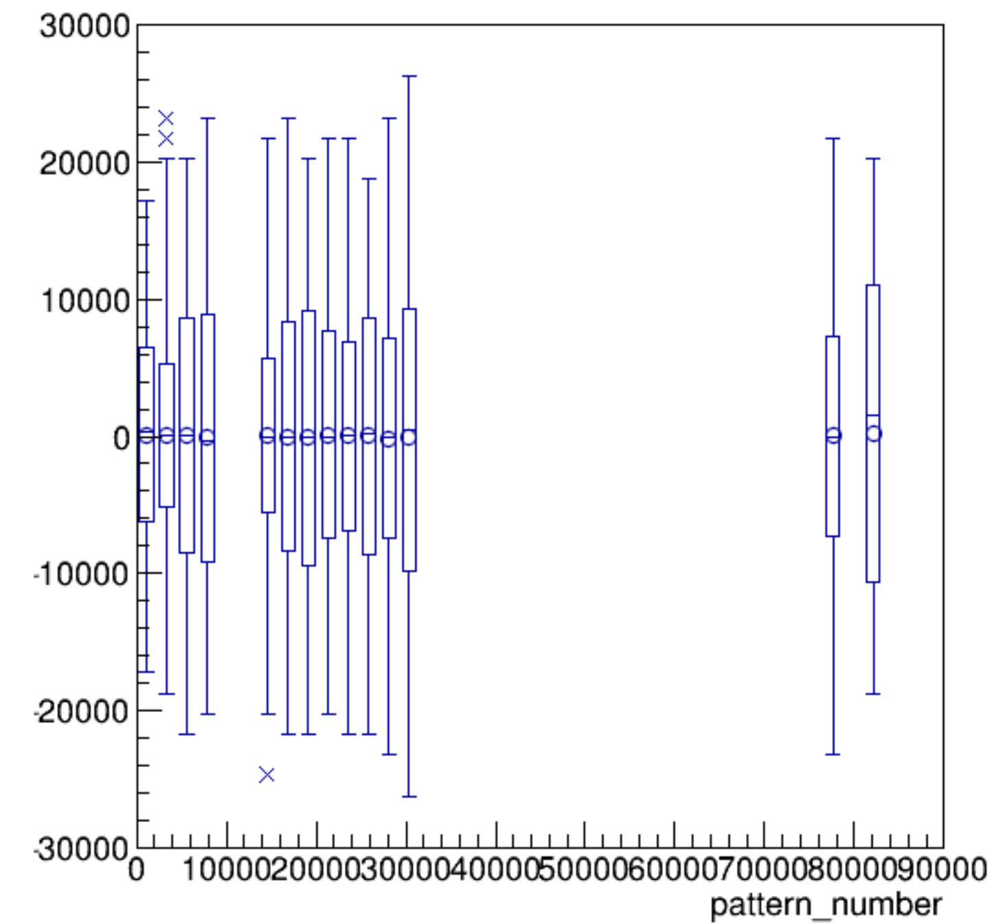
asym_sam3/ppm:pattern_number {ErrorFlag==0}
