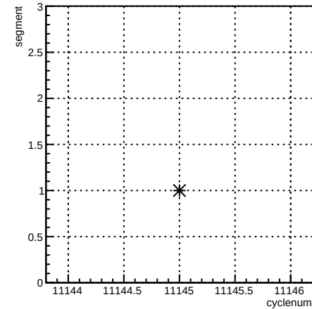
segment:cyclenum {run == 8312}
