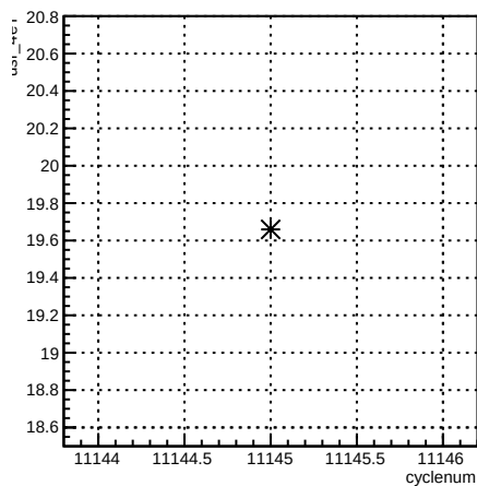
usr_4eY:cyclenum {run == 8312}
