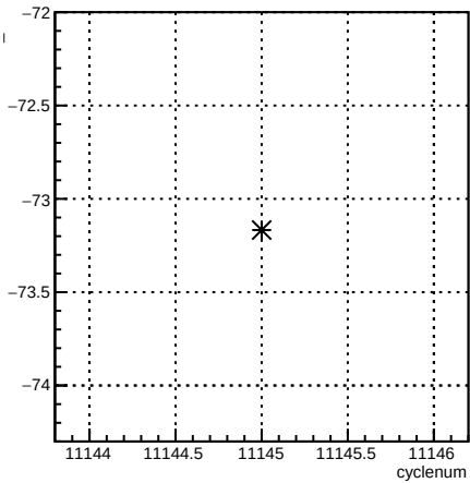
usl_1X:cyclenum {run == 8312}
