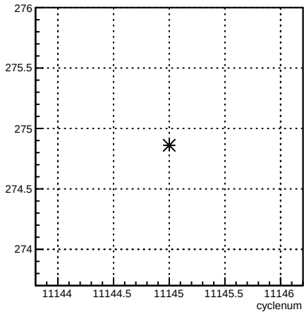
4eY_coil4:cyclenum {run == 8312}
