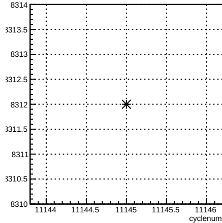
run:cyclenum {run == 8312}
