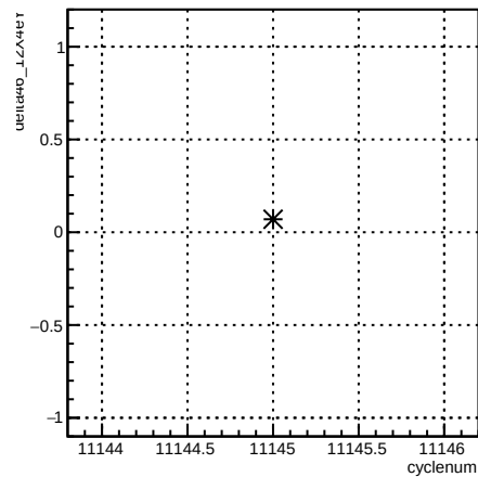
delta46_12X4eY:cyclenum {run == 8312}
