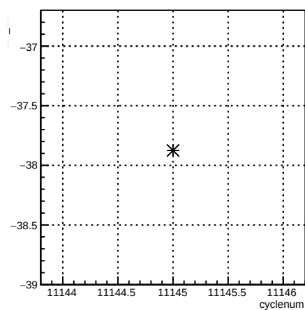
usr_12X:cyclenum {run == 8312}
