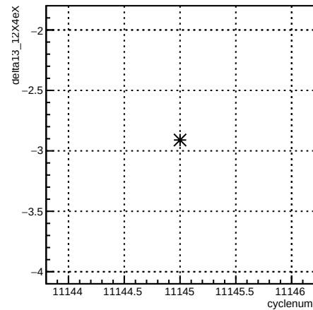
delta13_12X4eX:cyclenum {run == 8312}
