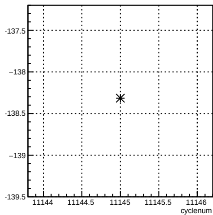
4eY_coil6:cyclenum {run == 8312}
