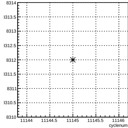
run:cyclenum {run == 8312}
