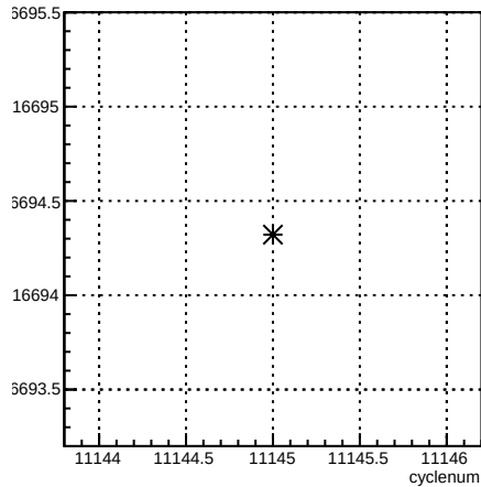
usl_coil1:cyclenum {run == 8312}
