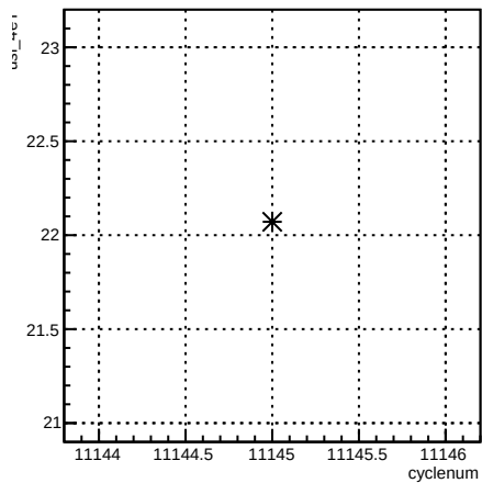
usl_4eY:cyclenum {run == 8312}
