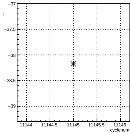
4aY_coil7:cyclenum {run == 8312}
