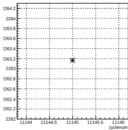
usl_coil3:cyclenum {run == 8312}
