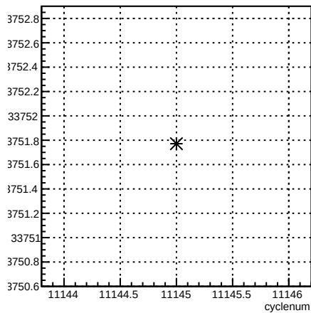
usr_coil7:cyclenum {run == 8312}
