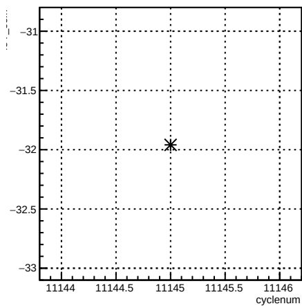
4eY_coil7:cyclenum {run == 8312}
