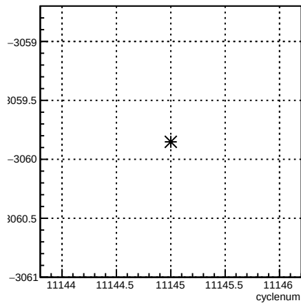
usl_coil6:cyclenum {run == 8312}
