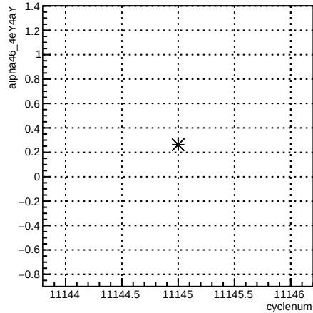
alpha46_4eY4aY:cyclenum {run == 8312}
