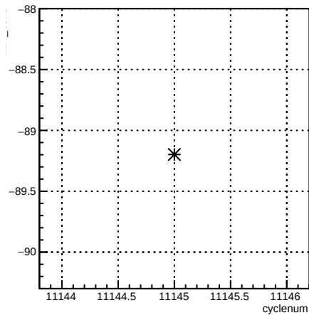
12X_coil3:cyclenum {run == 8312}
