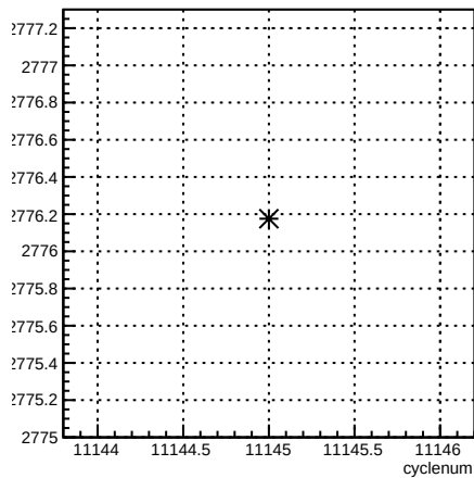
usl_coil7:cyclenum {run == 8312}
