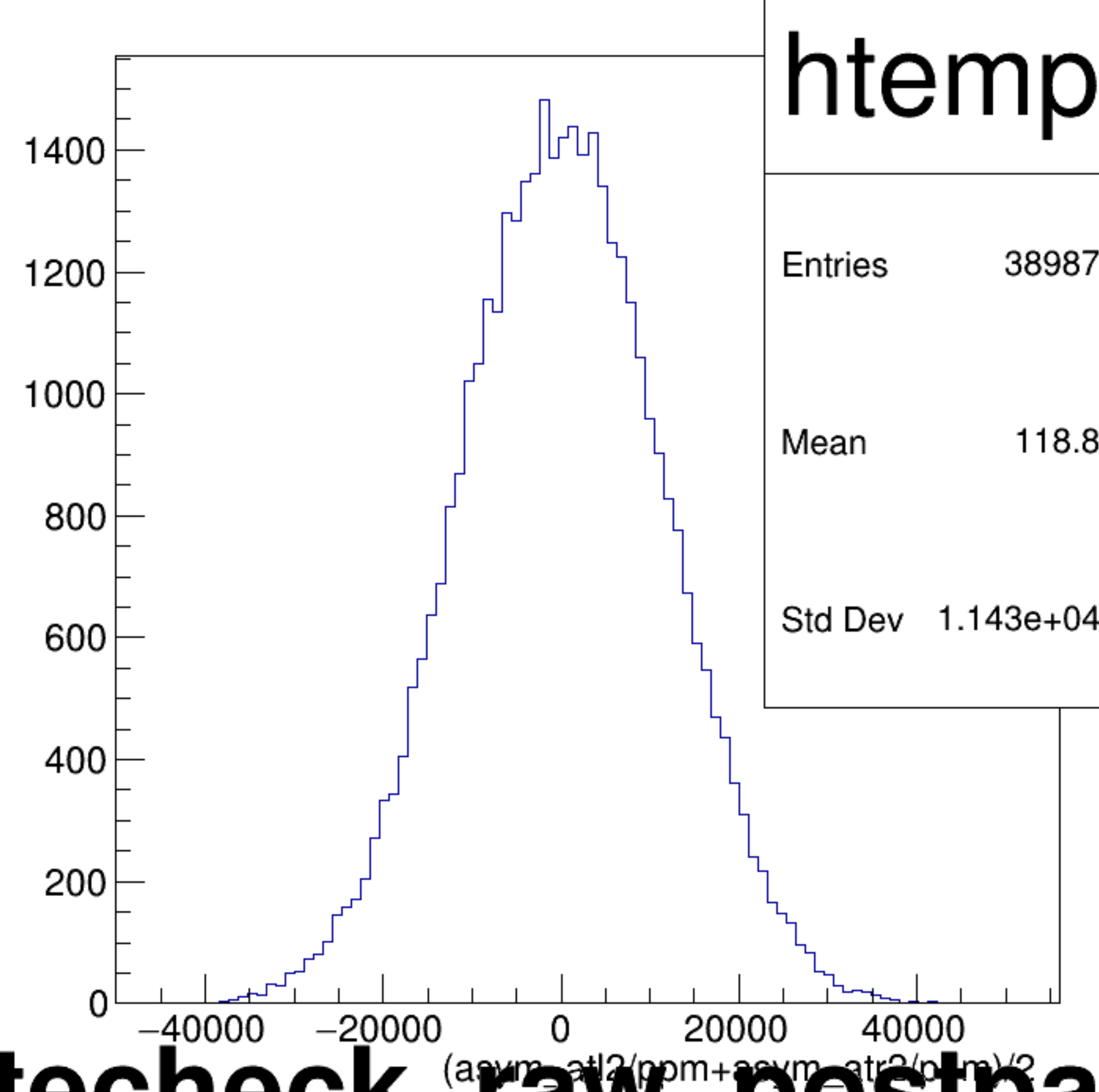
(asym_atl2/ppm+asym_atr2/ppm)/2 {ok_cut}
