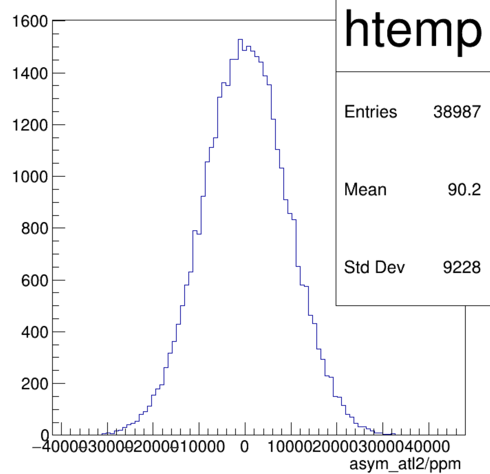
asym_atl2/ppm {ok_cut}
