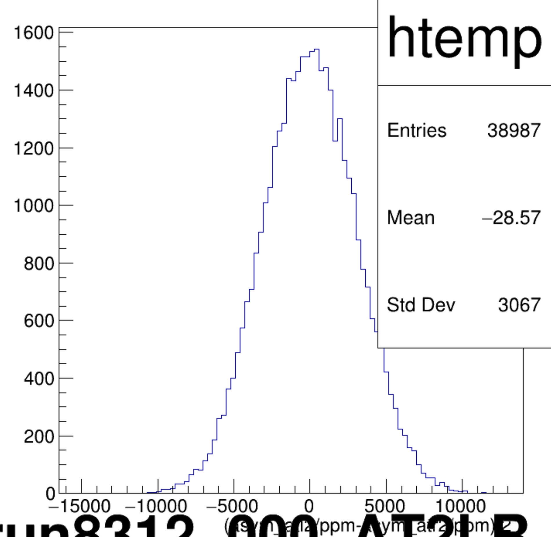
(asym_atl2/ppm-asym_atr2/ppm)/2 {ok_cut}
