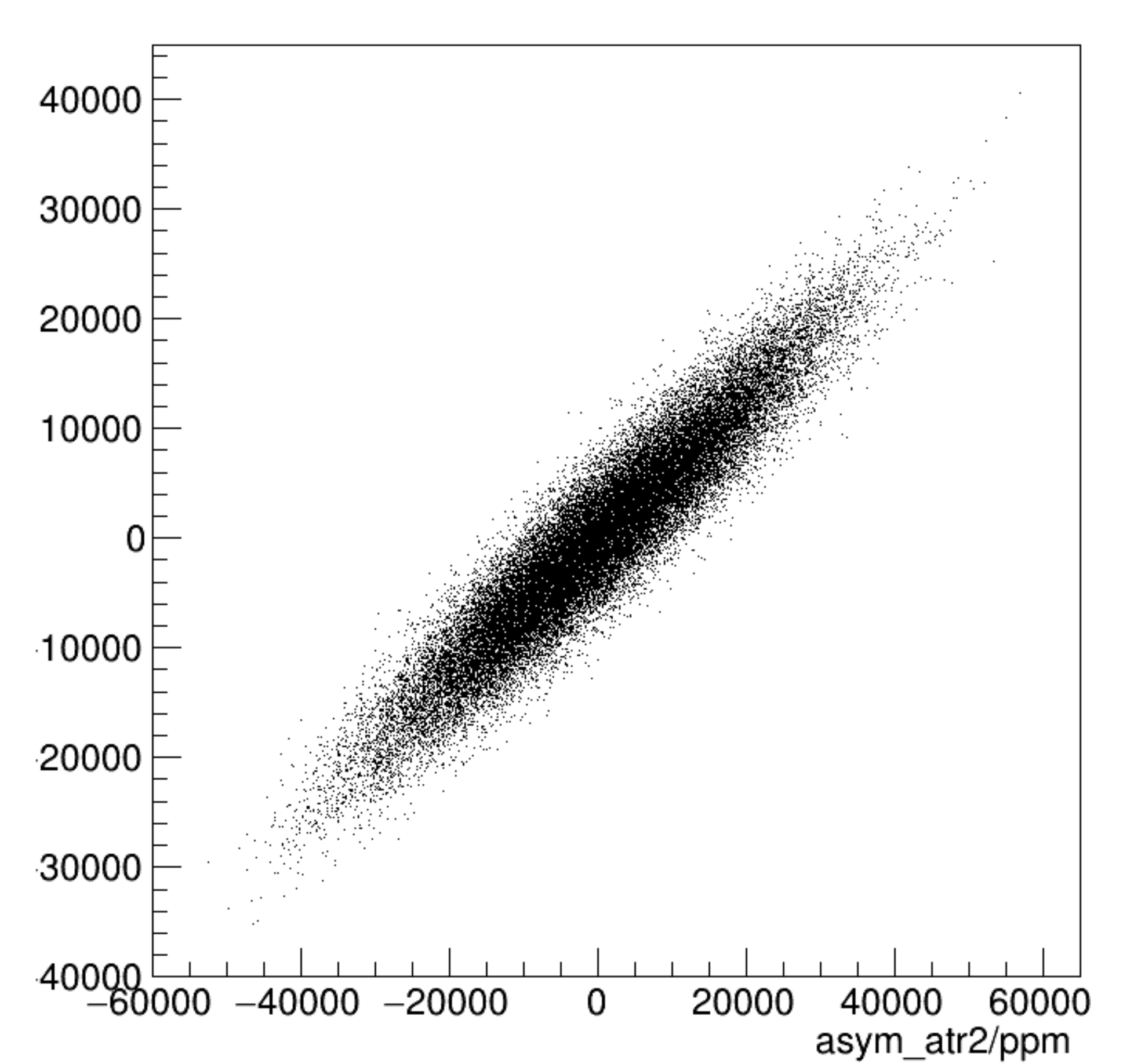
asym_atl2/ppm:asym_atr2/ppm {ok_cut}
