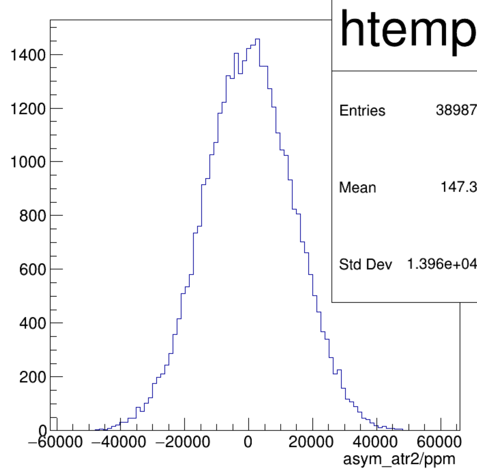
asym_atr2/ppm {ok_cut}
