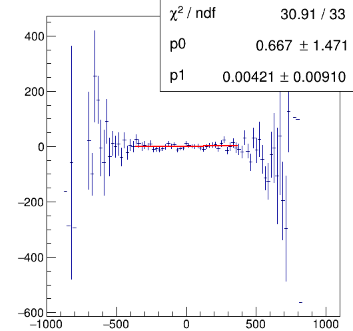
reg_asym_dsr/ppm:AqDS/ppm {ok_cut}
