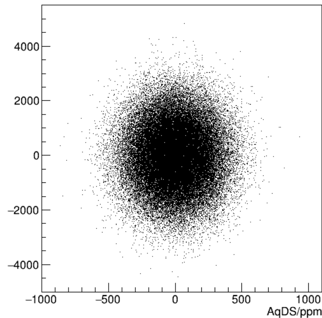
reg_asym_usr/ppm:AqDS/ppm {ok_cut}
