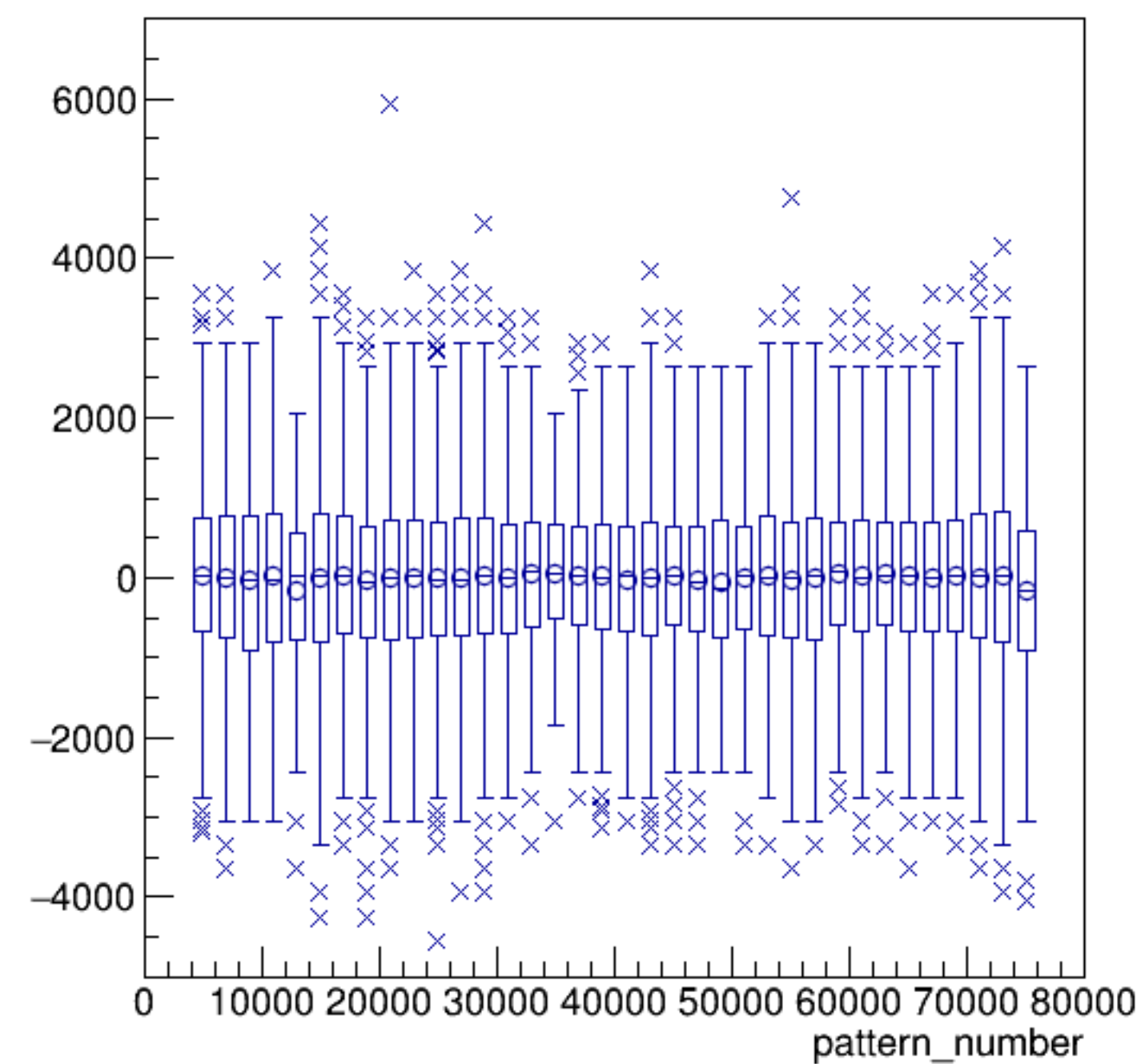
asym_sam5/ppm:pattern_number {ErrorFlag==0}
