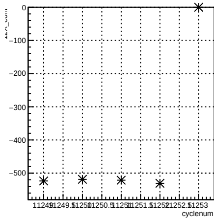
12X_coil7:cyclenum {run == 8340}
