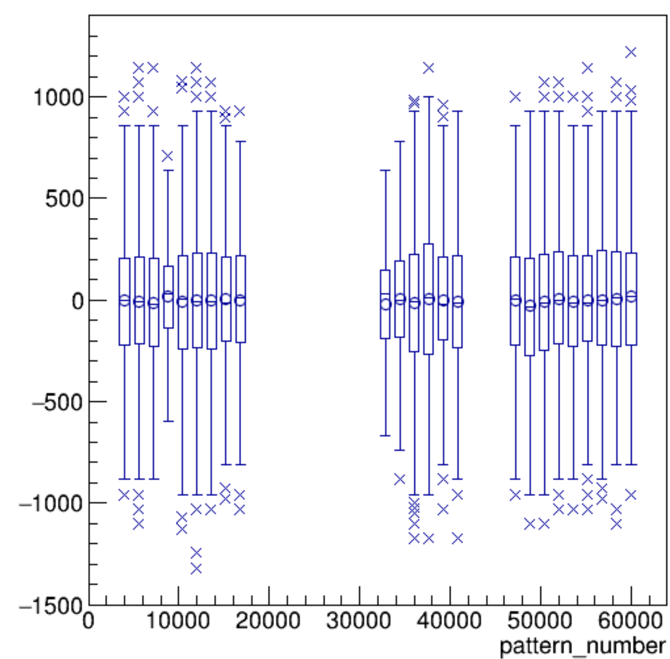
asym_sam8/ppm:pattern_number {ErrorFlag==0}
