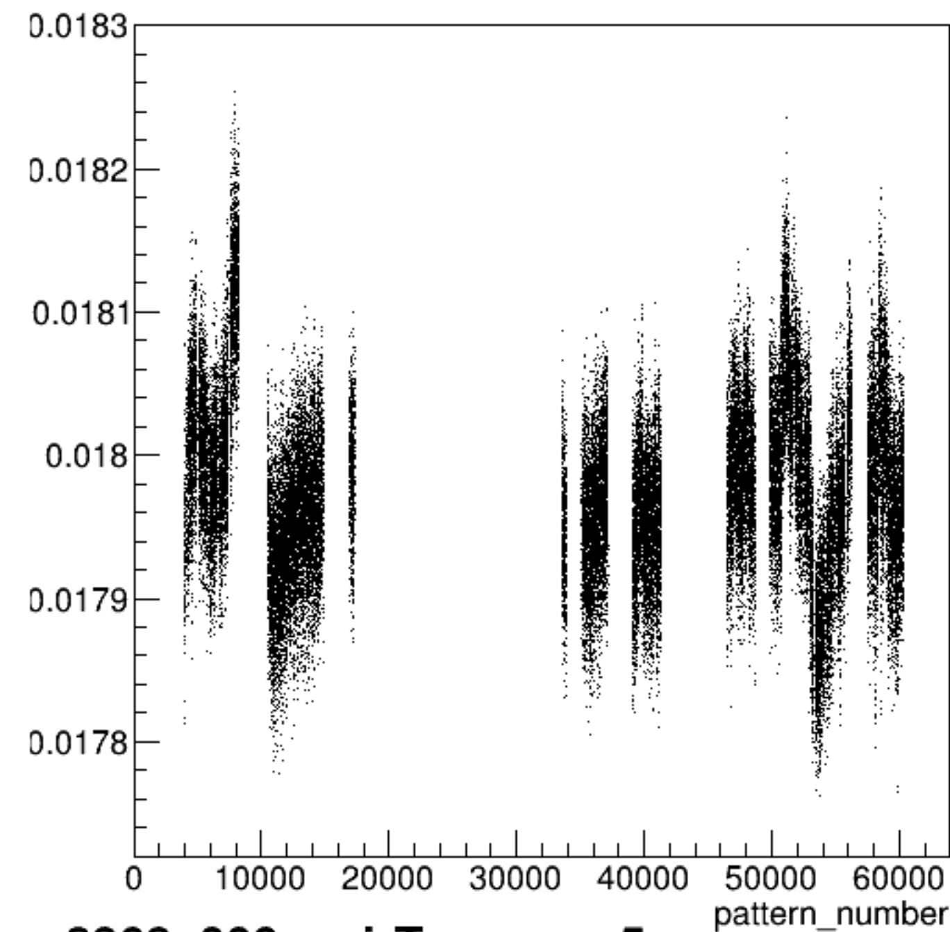
yield_sam5:pattern_number {ErrorFlag==0}
