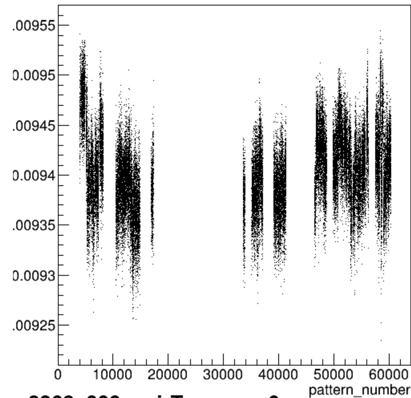
yield_sam6:pattern_number {ErrorFlag==0}
