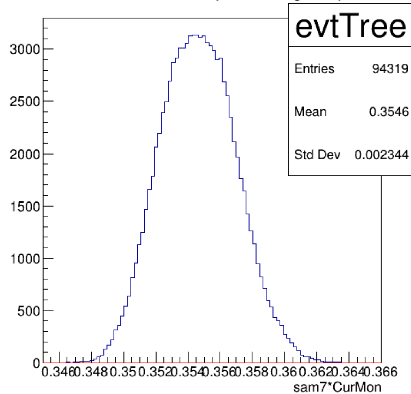
sam7*CurMon {ErrorFlag==0}
