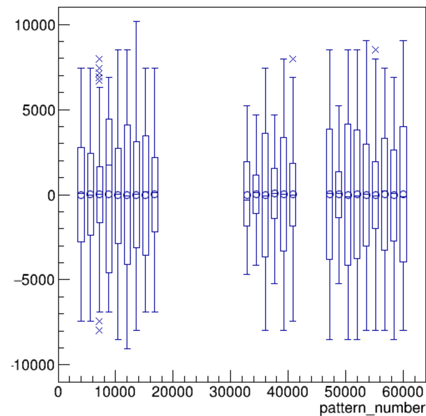
asym_sam5/ppm:pattern_number {ErrorFlag==0}
