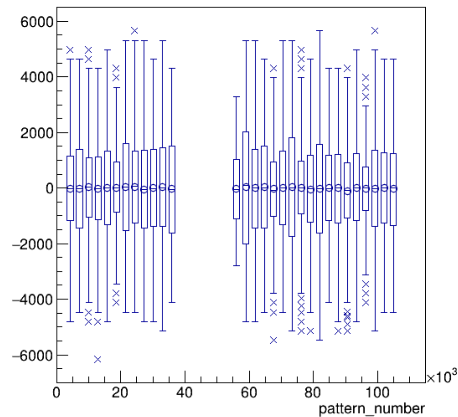
asym_sam7/ppm:pattern_number {ErrorFlag==0}
