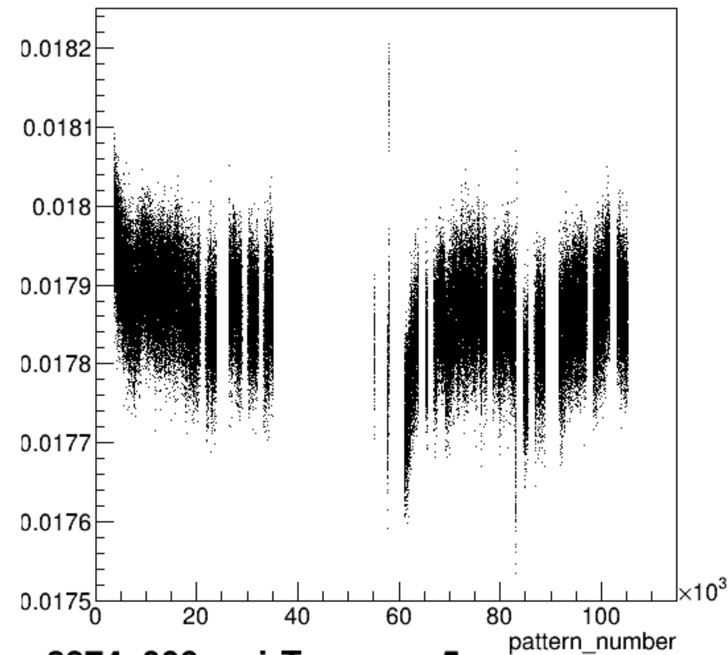
yield_sam5:pattern_number {ErrorFlag==0}
