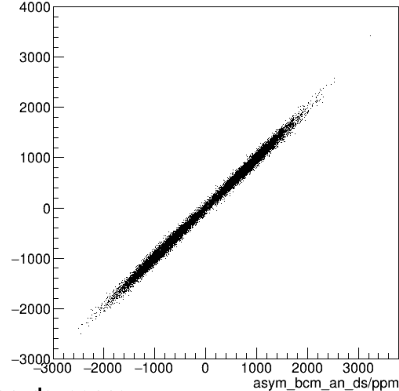
run8376_000_asym_bcm_dg_us_vs_asym_bcm_an_ds_pr.png
