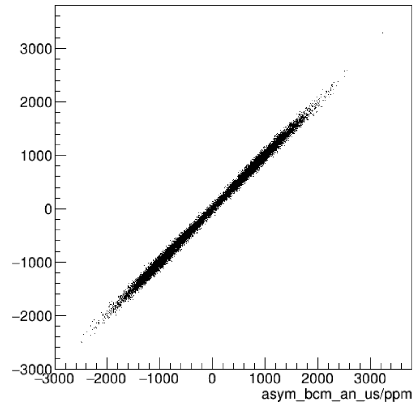
run8376_000_asym_bcm_dg_ds_vs_asym_bcm_an_us_pr.png
