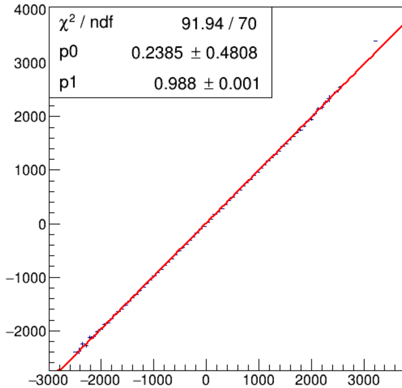
run8376_000_asym_bcm_dg_us_vs_asym_bcm_an_ds_pr.png
