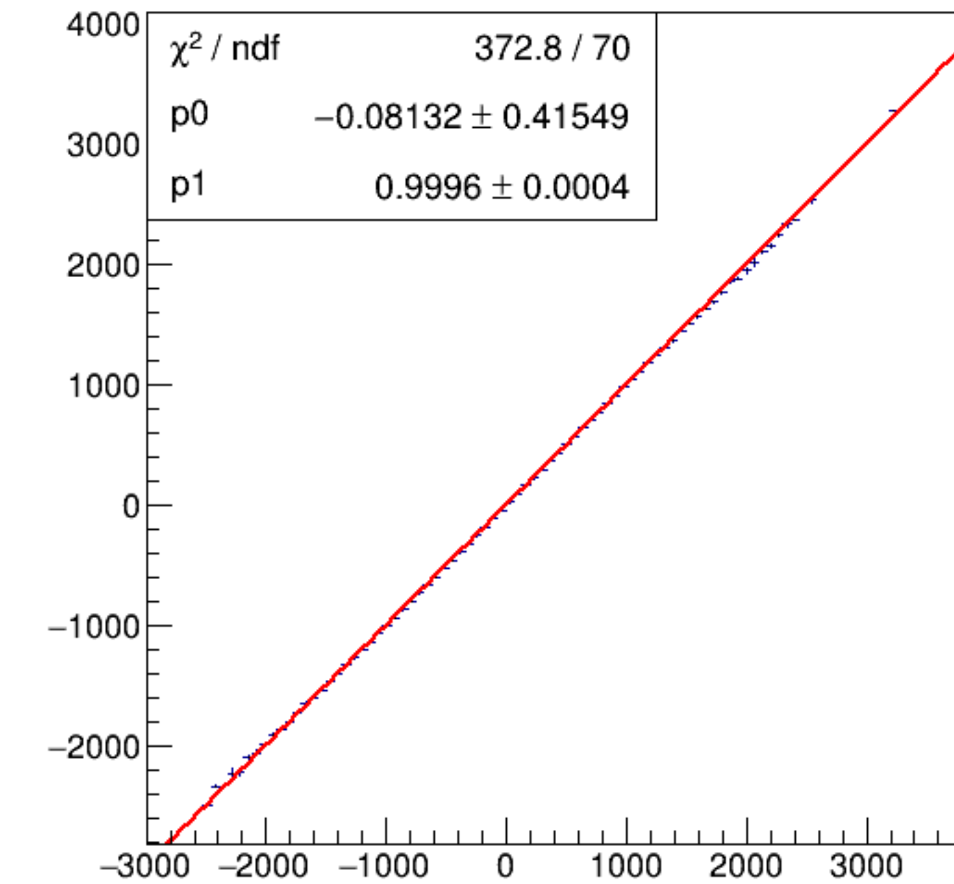
run8376_000_asym_bcm_dg_ds_vs_asym_bcm_an_us_pr.png
