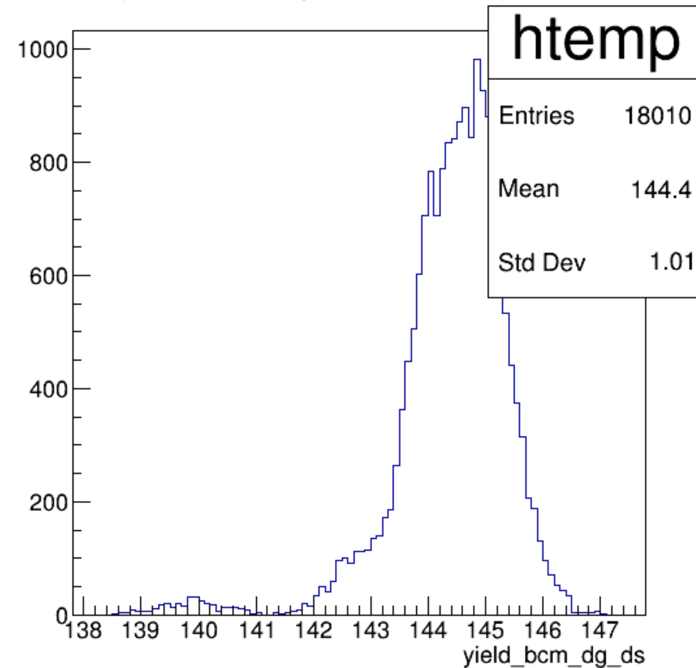
yield_bcm_dg_ds {ErrorFlag==0}
