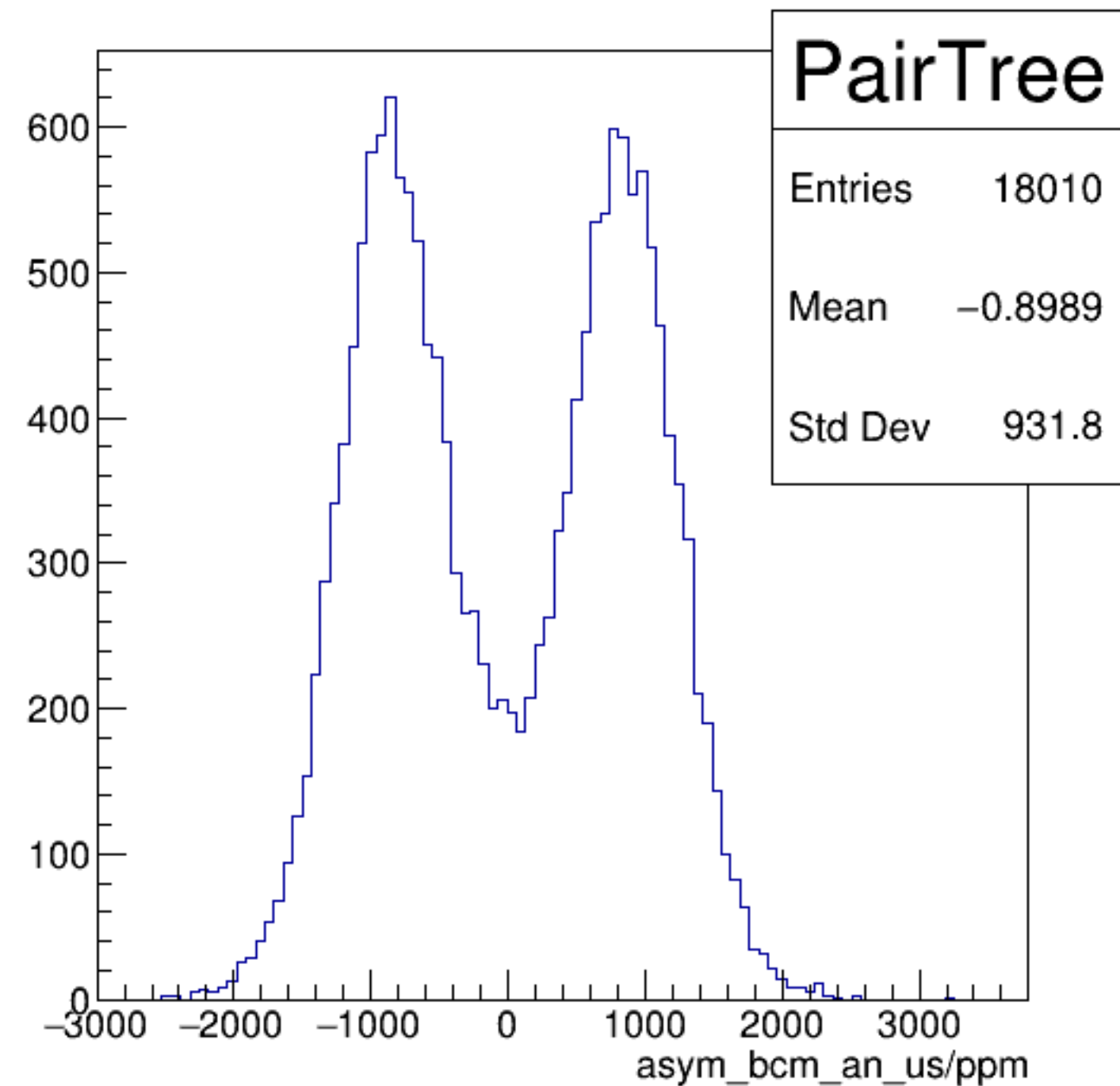
asym_bcm_an_us/ppm {ErrorFlag==0}
