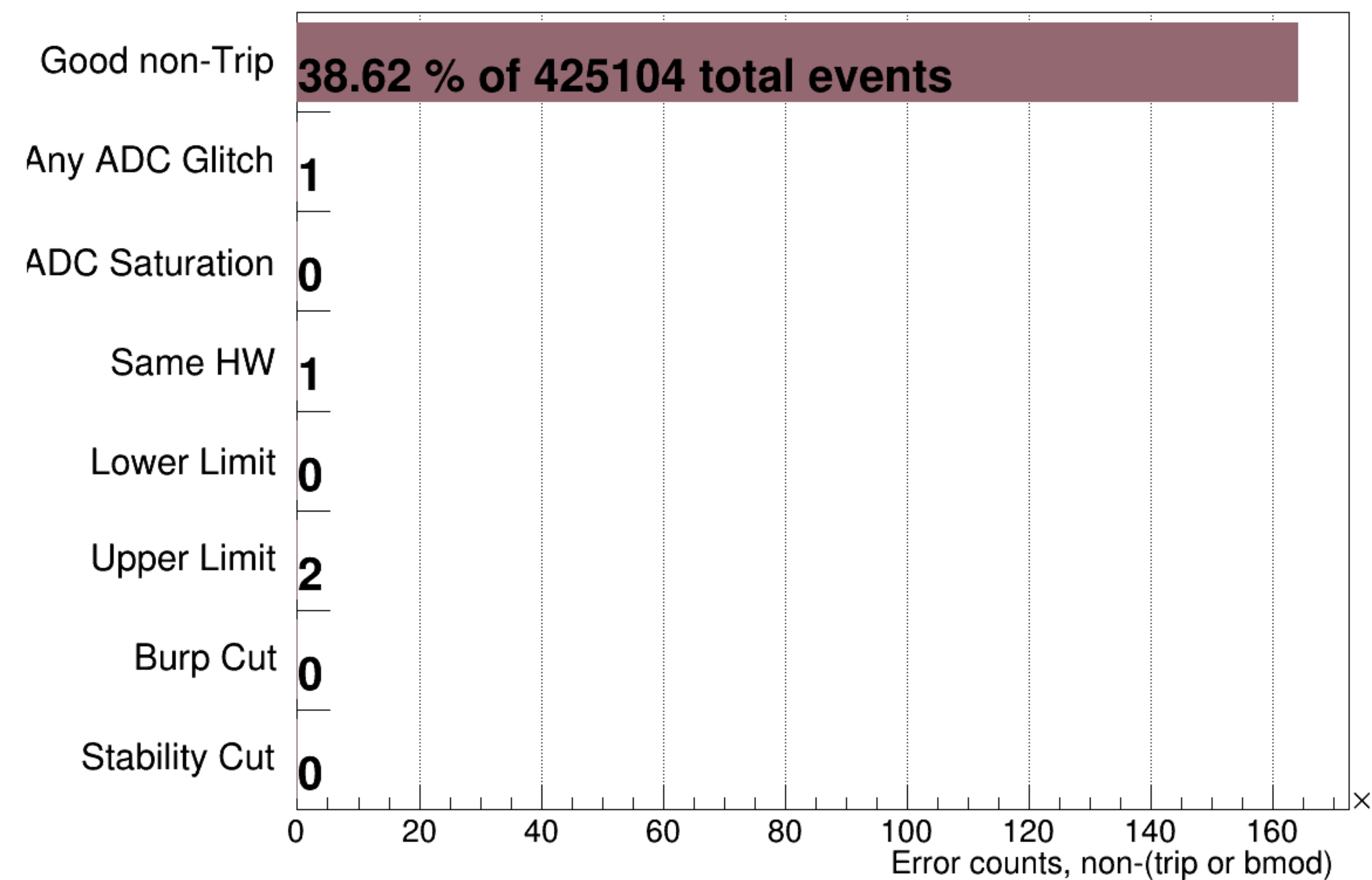
bpm11XM's Device Error Counter &amp; Not (Trip || BMOD)
