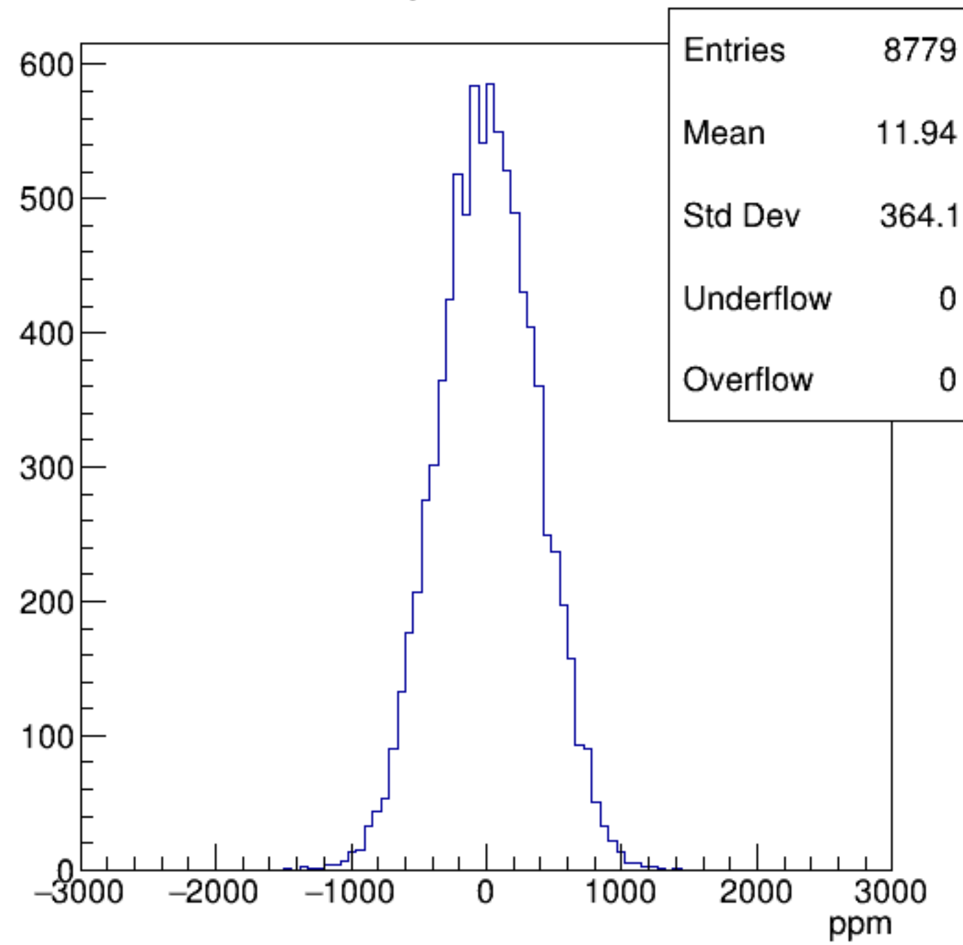
asym_sam8
