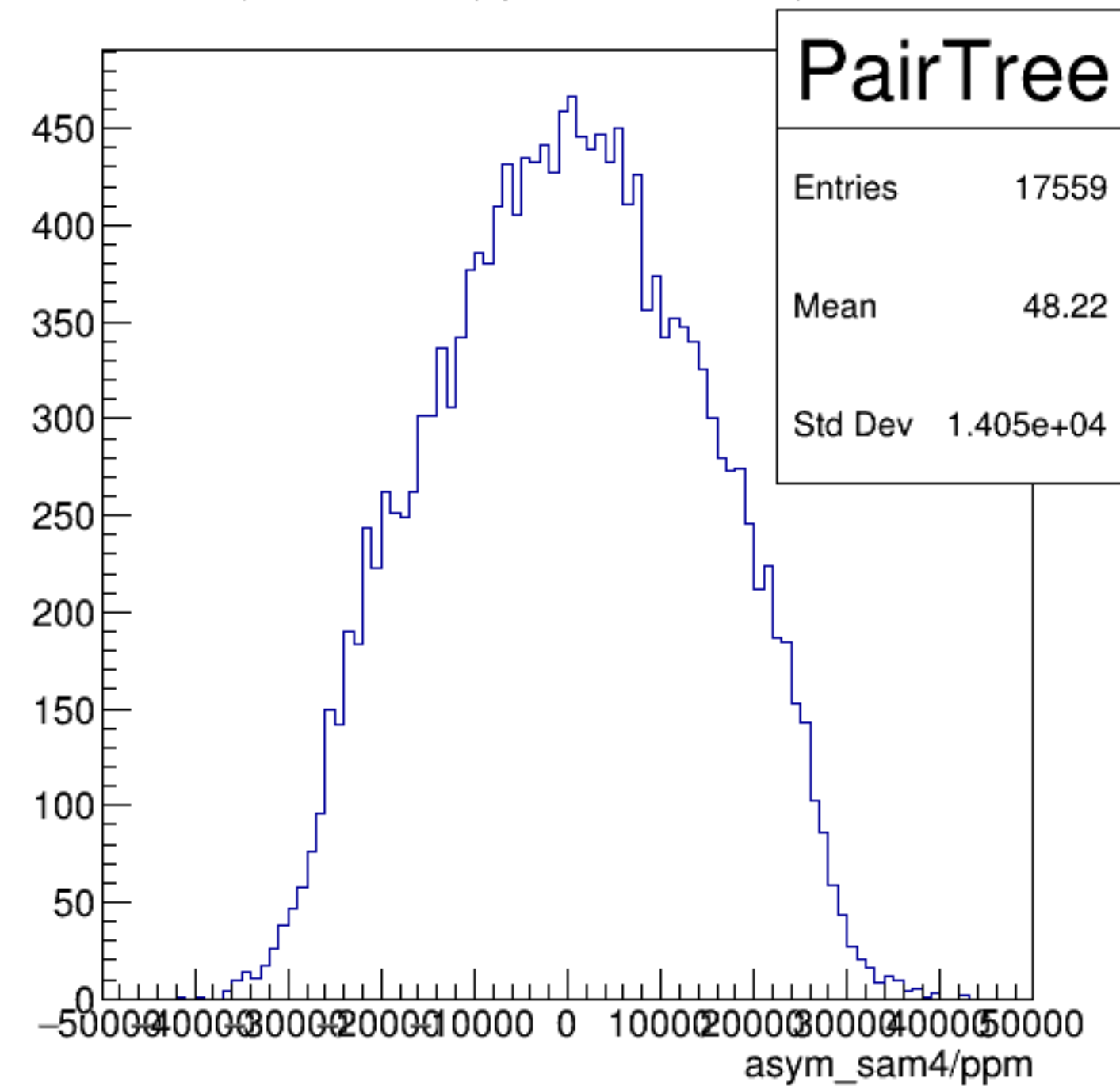
asym_sam4/ppm {ErrorFlag==0}
