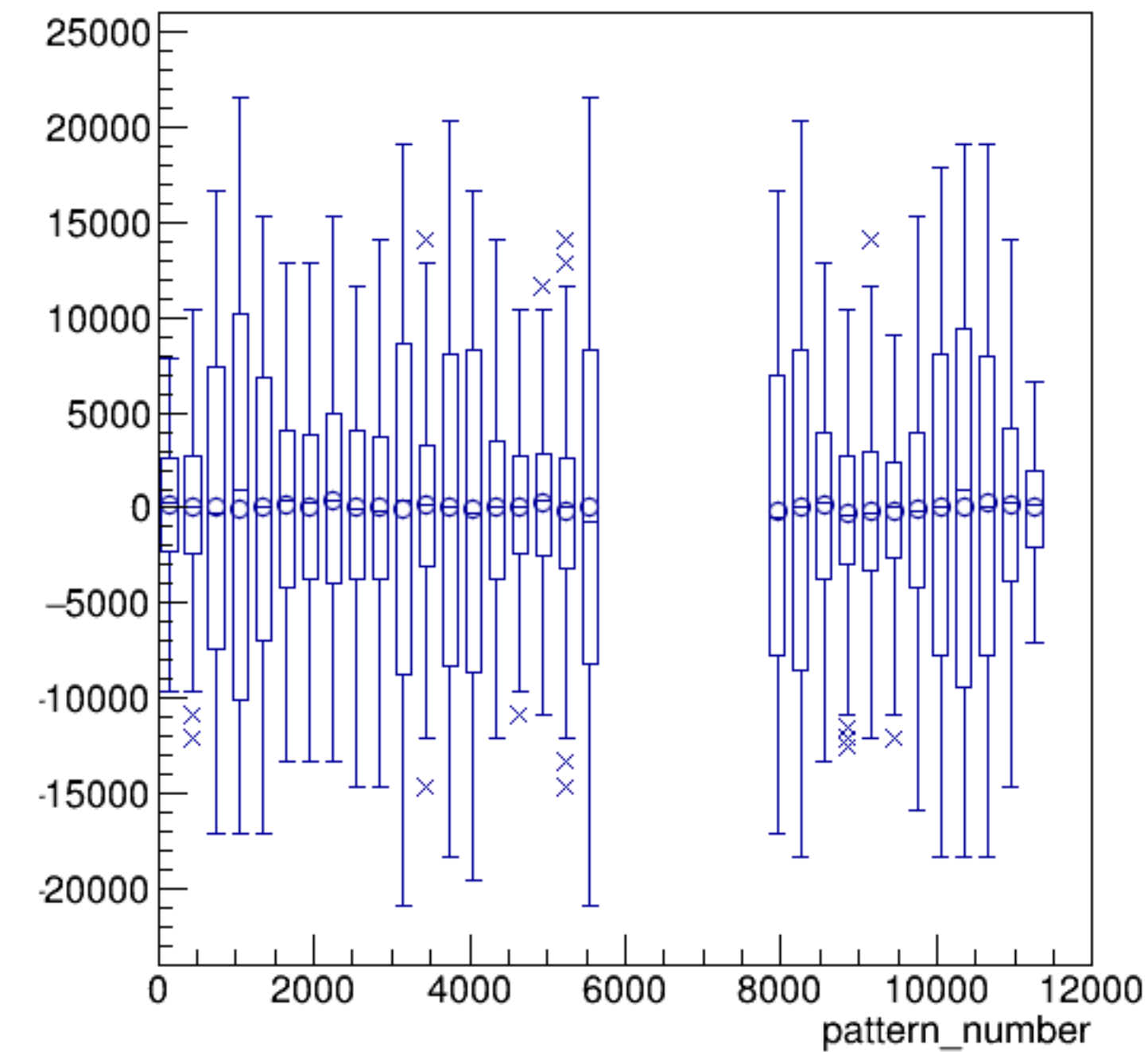
asym_sam3/ppm:pattern_number {ErrorFlag==0}
