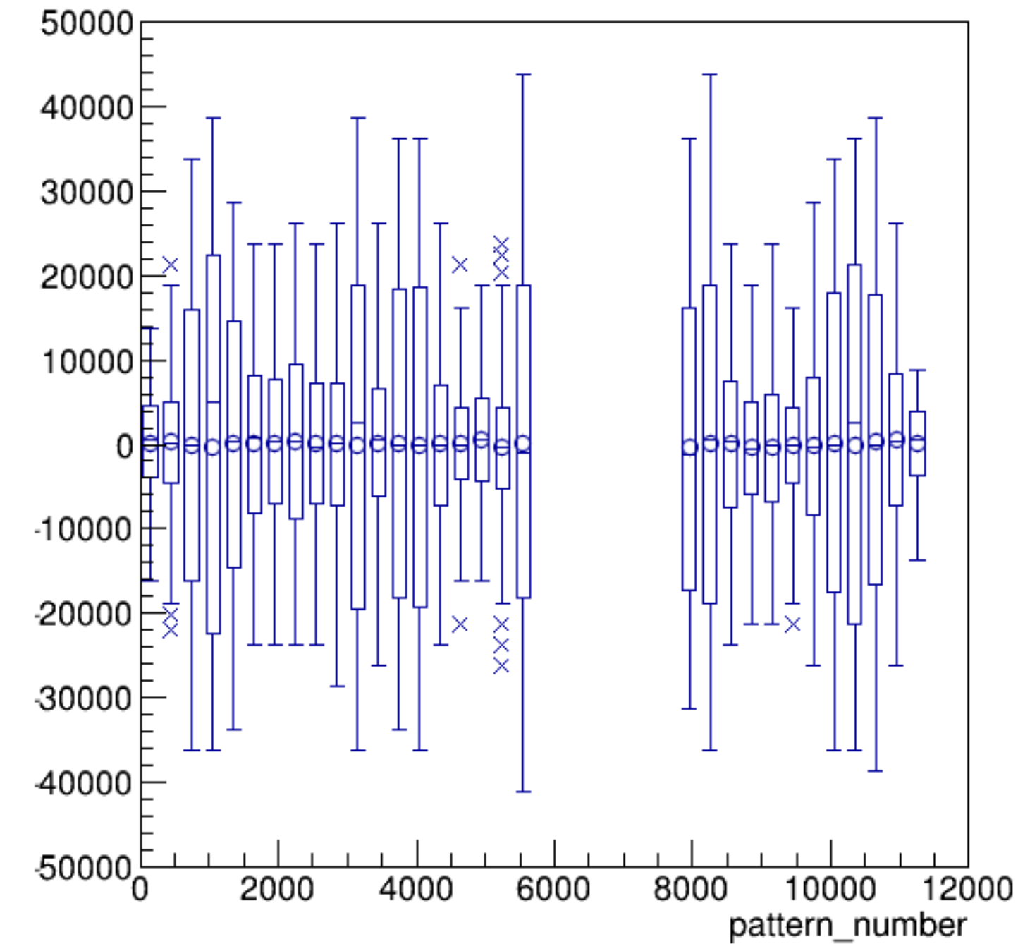
asym_sam4/ppm:pattern_number {ErrorFlag==0}
