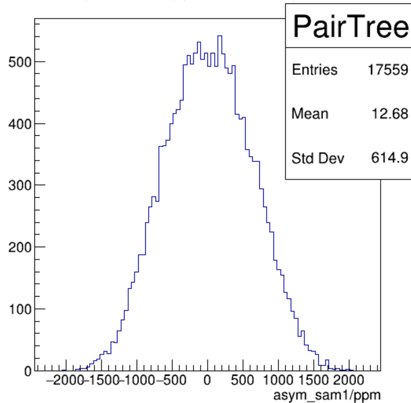
asym_sam1/ppm {ErrorFlag==0}
