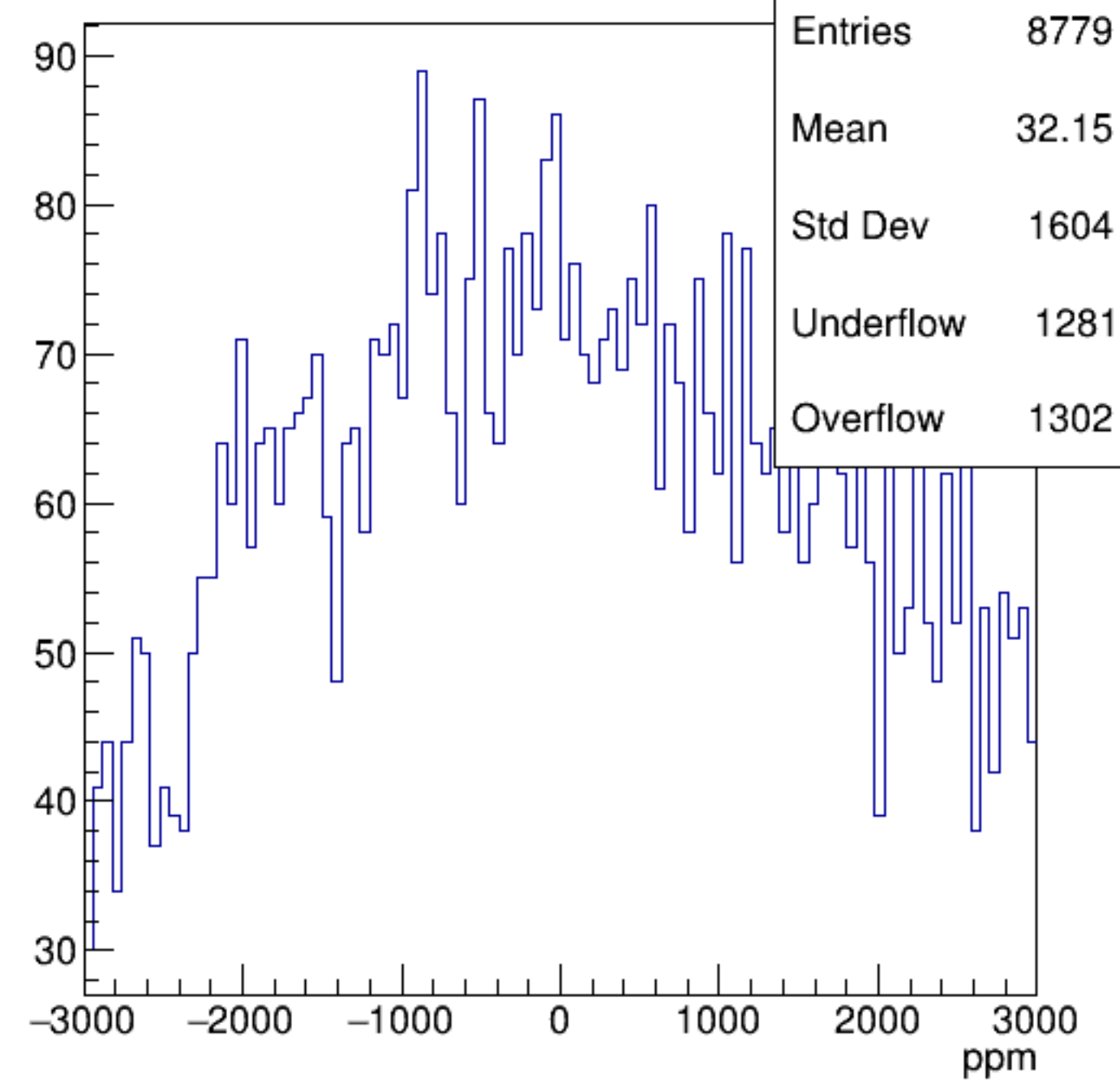
asym_sam3
