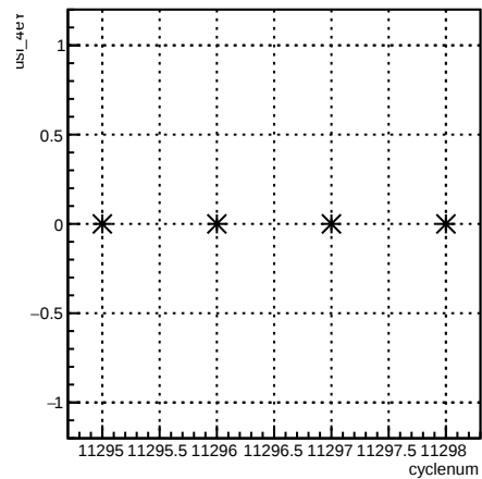
usl_4eY:cyclenum {run == 8350}
