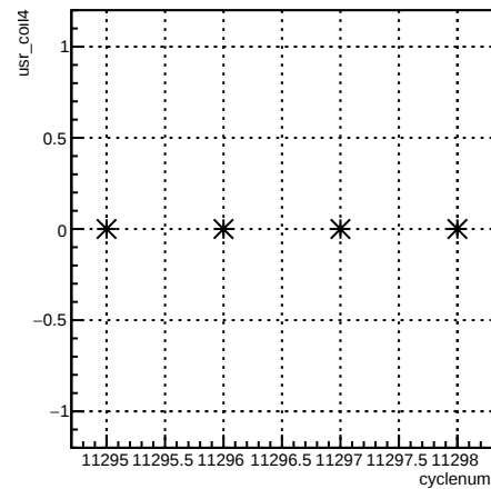
usr_coil4:cyclenum {run == 8350}
