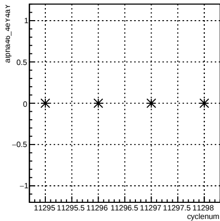
alpha46_4eY4aY:cyclenum {run == 8350}
