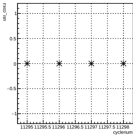
usl_coil3:cyclenum {run == 8350}
