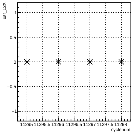
usr_12X:cyclenum {run == 8350}
