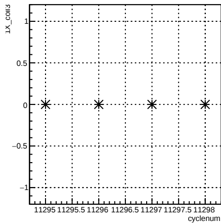
1X_coil3:cyclenum {run == 8350}
