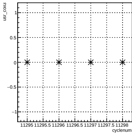
usr_coil3:cyclenum {run == 8350}
