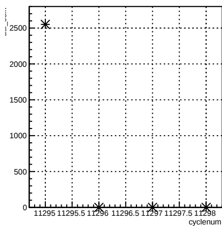
usl_coil7:cyclenum {run == 8350}
