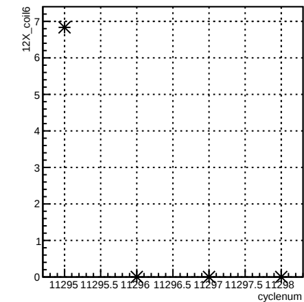
12X_coil6:cyclenum {run == 8350}
