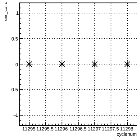
usr_coil1:cyclenum {run == 8350}
