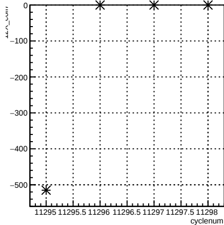
12X_coil7:cyclenum {run == 8350}
