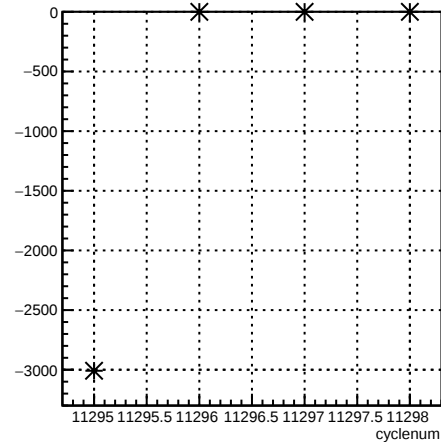
usr_coil6:cyclenum {run == 8350}
