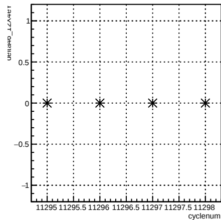
delta46_12X4eY:cyclenum {run == 8350}
