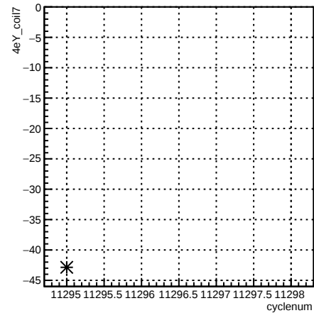
4eY_coil7:cyclenum {run == 8350}
