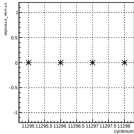
alpha13_4eX1X:cyclenum {run == 8350}
