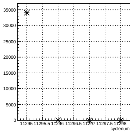
usr_coil7:cyclenum {run == 8350}
