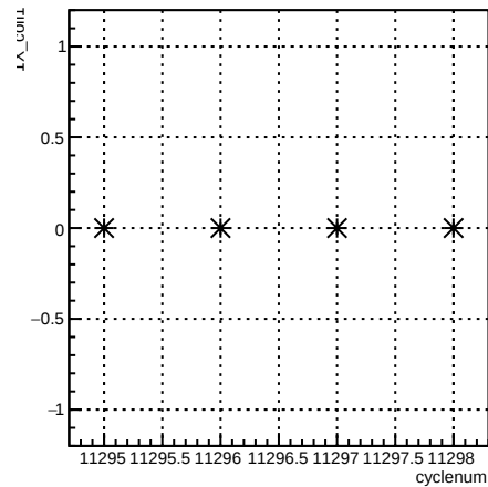
1X_coil1:cyclenum {run == 8350}
