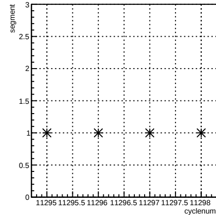
segment:cyclenum {run == 8350}
