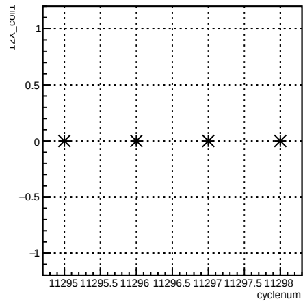
12X_coil1:cyclenum {run == 8350}
