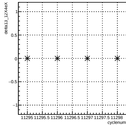
delta13_12X4eX:cyclenum {run == 8350}
