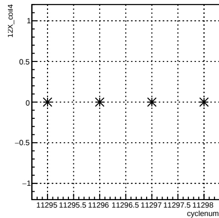
12X_coil4:cyclenum {run == 8350}
