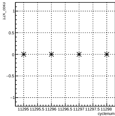
12X_coil3:cyclenum {run == 8350}
