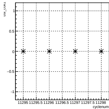
usl_coil1:cyclenum {run == 8350}
