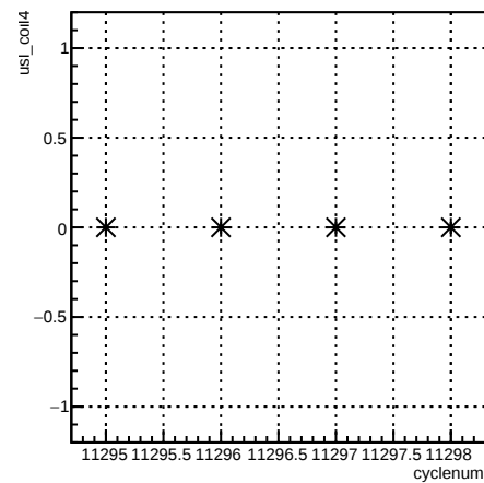
usl_coil4:cyclenum {run == 8350}
