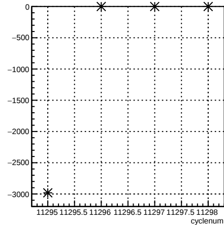
usl_coil6:cyclenum {run == 8350}
