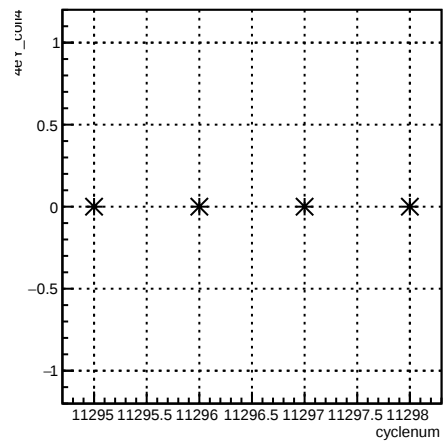
4eY_coil4:cyclenum {run == 8350}
