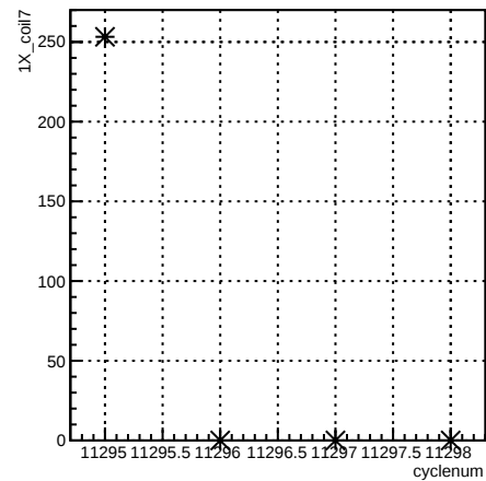
1X_coil7:cyclenum {run == 8350}
