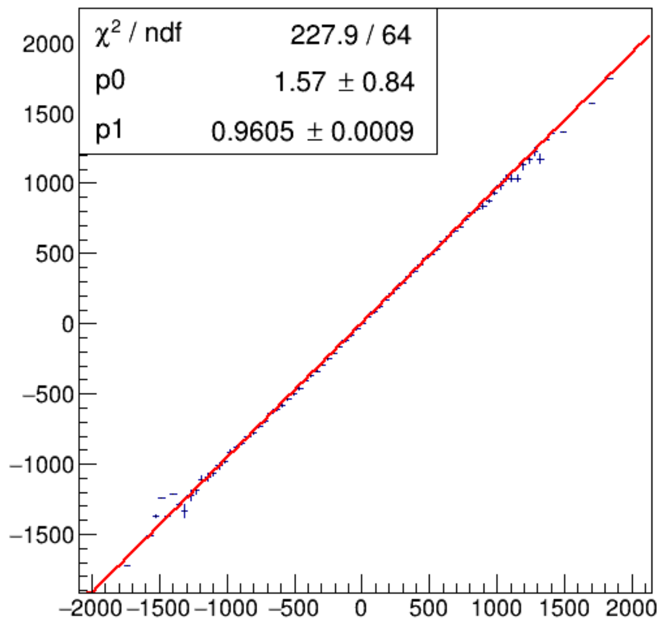
run8351_000_asym_bcm_dg_us_vs_asym_bcm_dg_ds_pr.png
