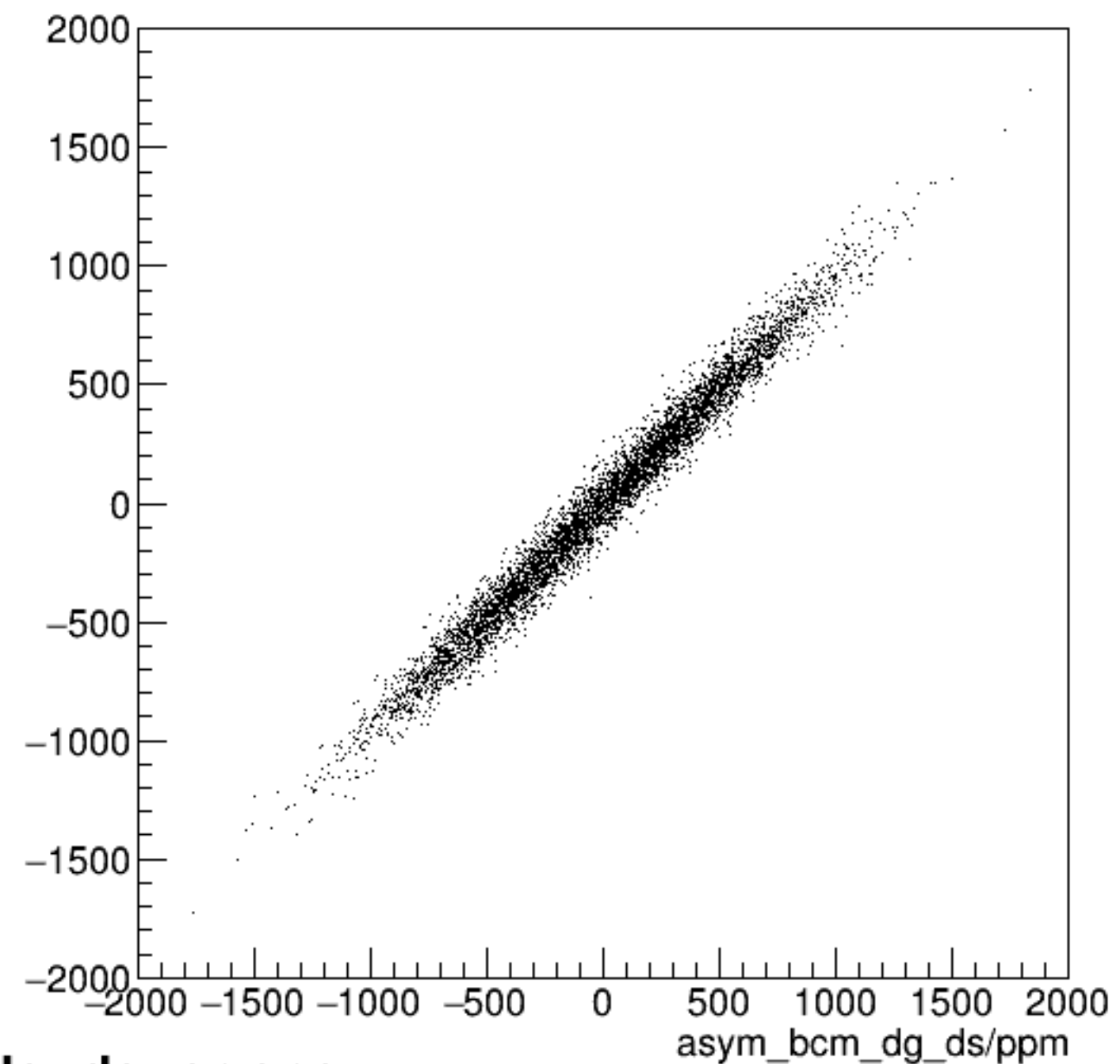
run8351_000_asym_bcm_dg_us_vs_asym_bcm_dg_ds_pr.png
