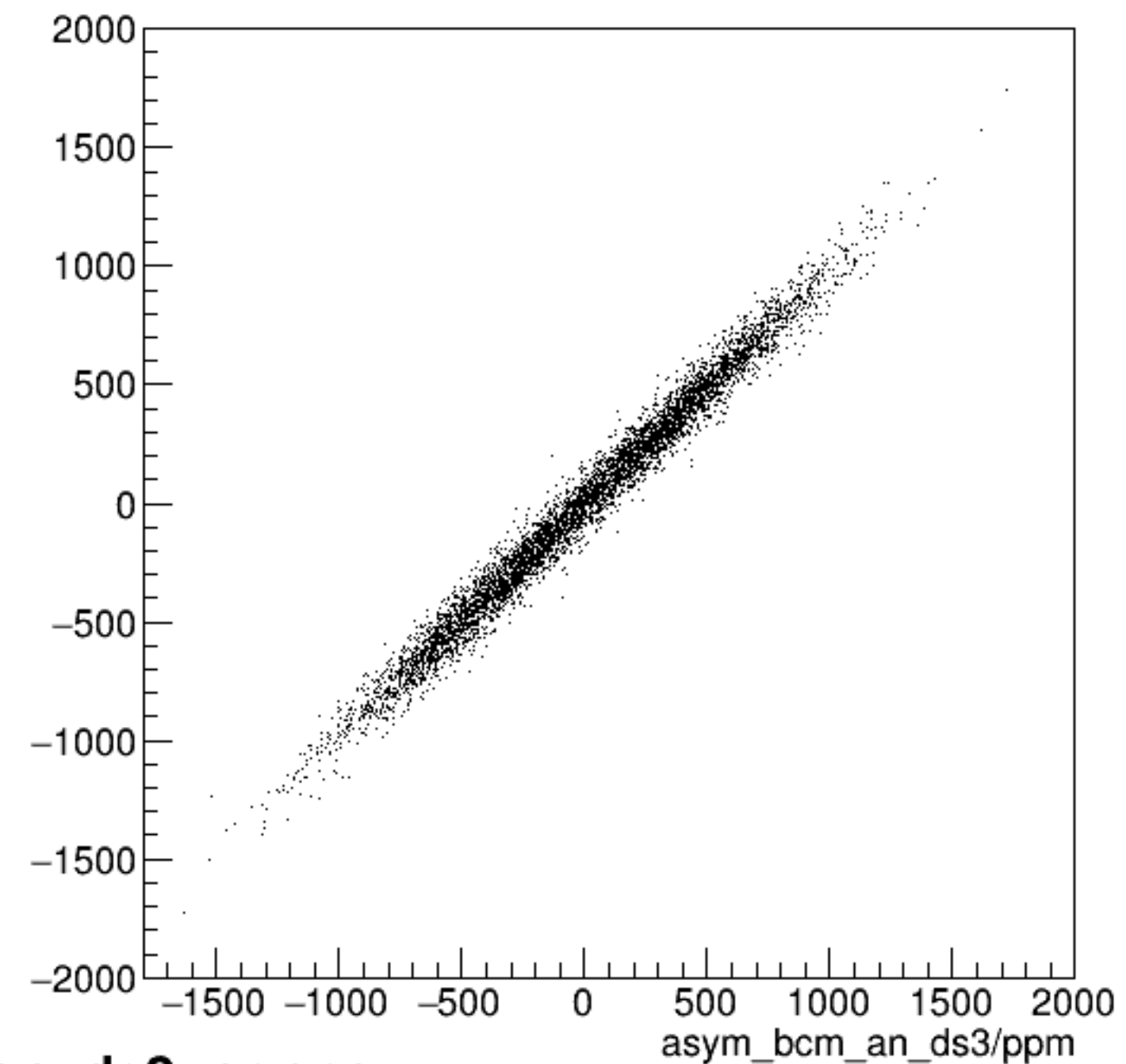
run8351_000_asym_bcm_dg_us_vs_asym_bcm_an_ds3_pr.png
