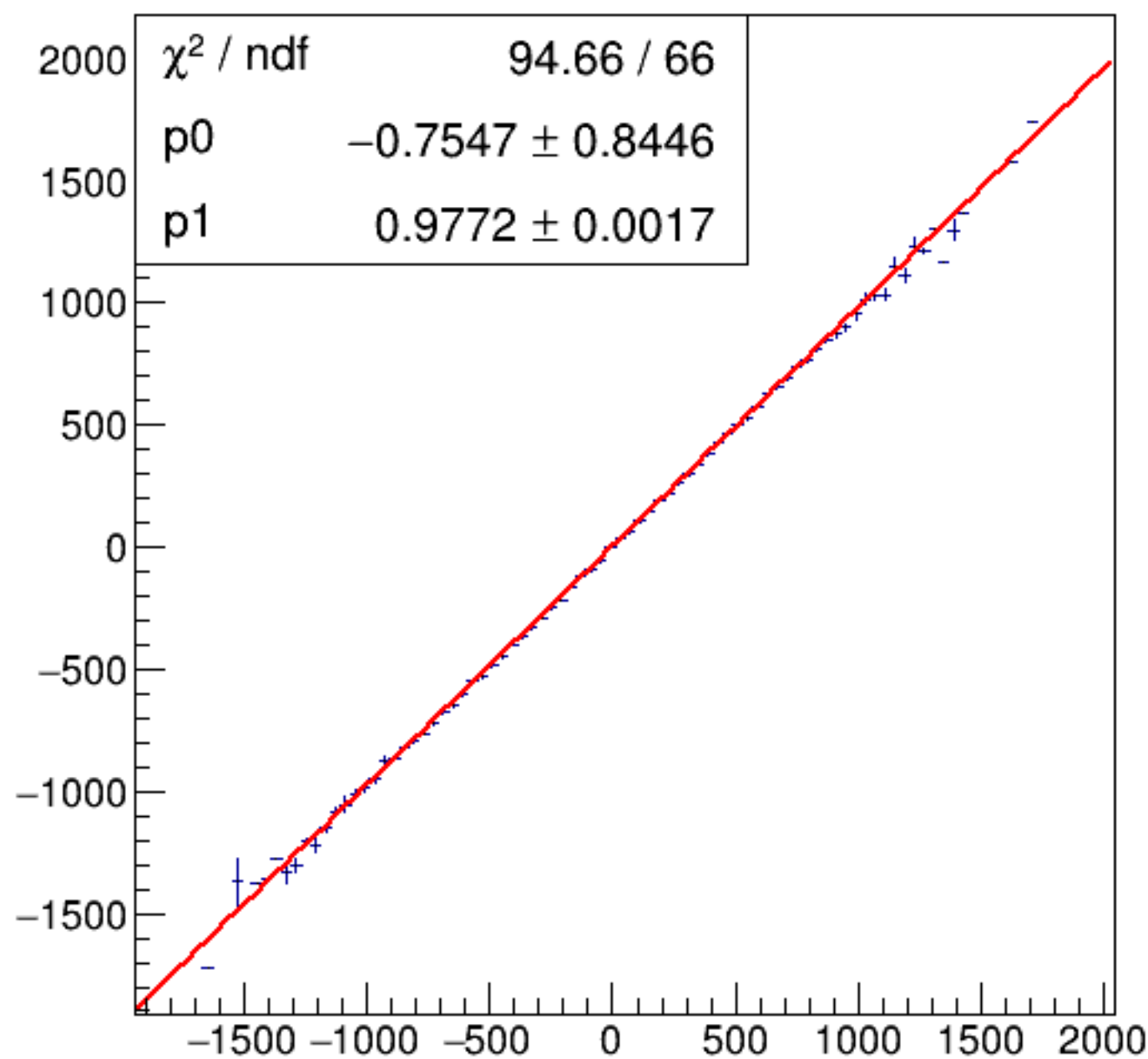
run8351_000_asym_bcm_dg_us_vs_asym_bcm_an_ds3_pr.png
