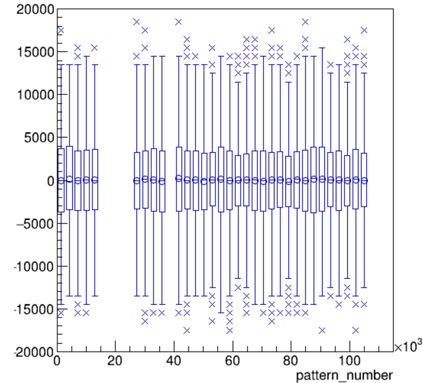
asym_usr/ppm:pattern_number {ErrorFlag==0}
