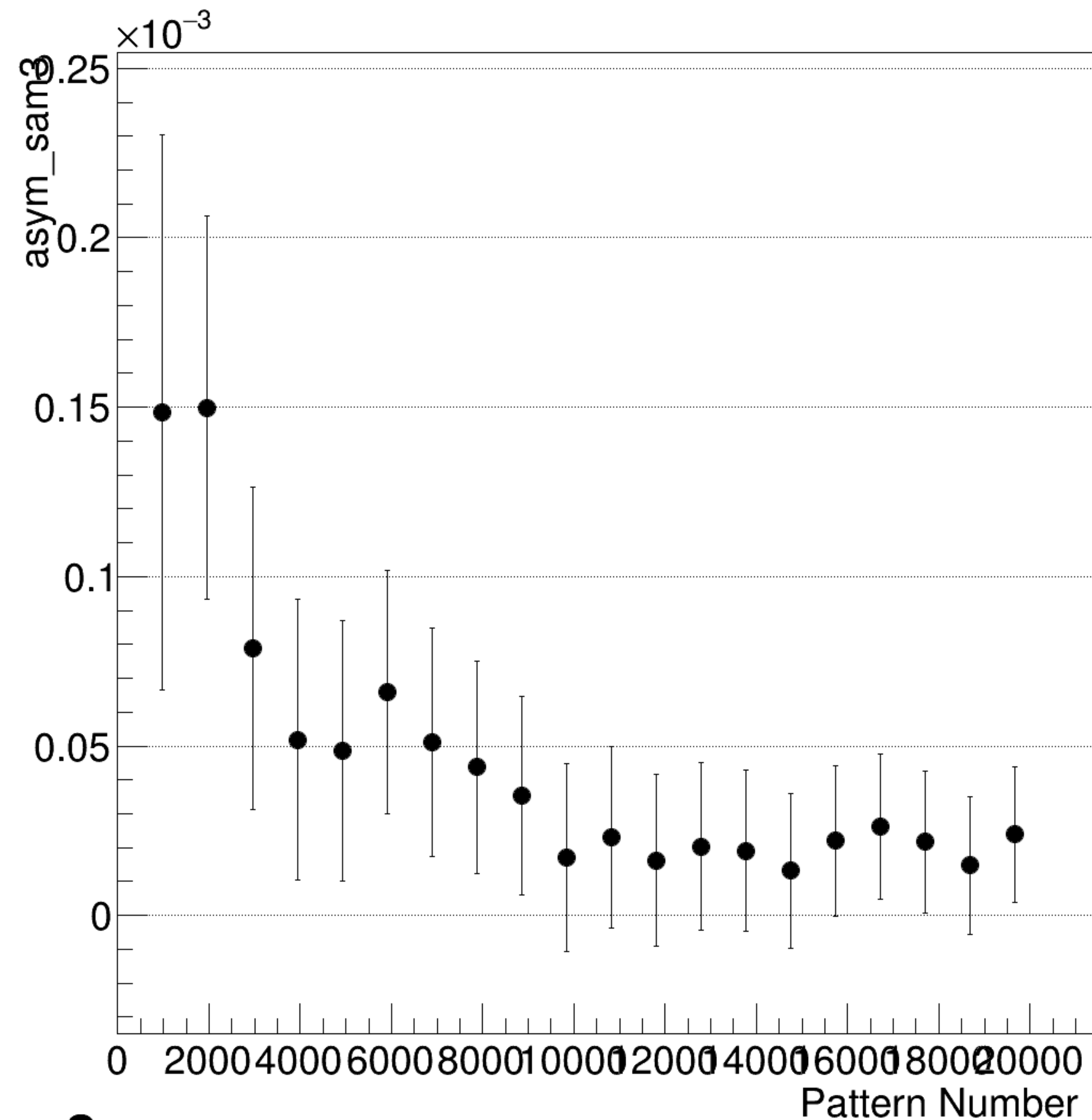
asym_sam3 Integrated Convergence
