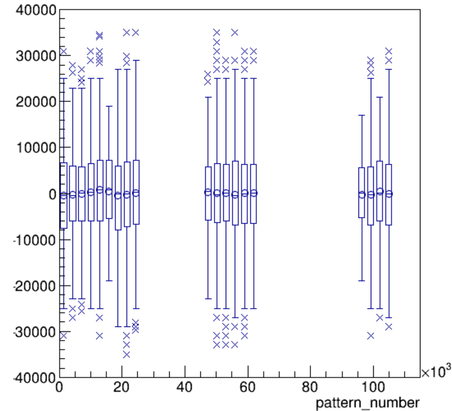
asym_atl2/ppm:pattern_number {ErrorFlag==0}
