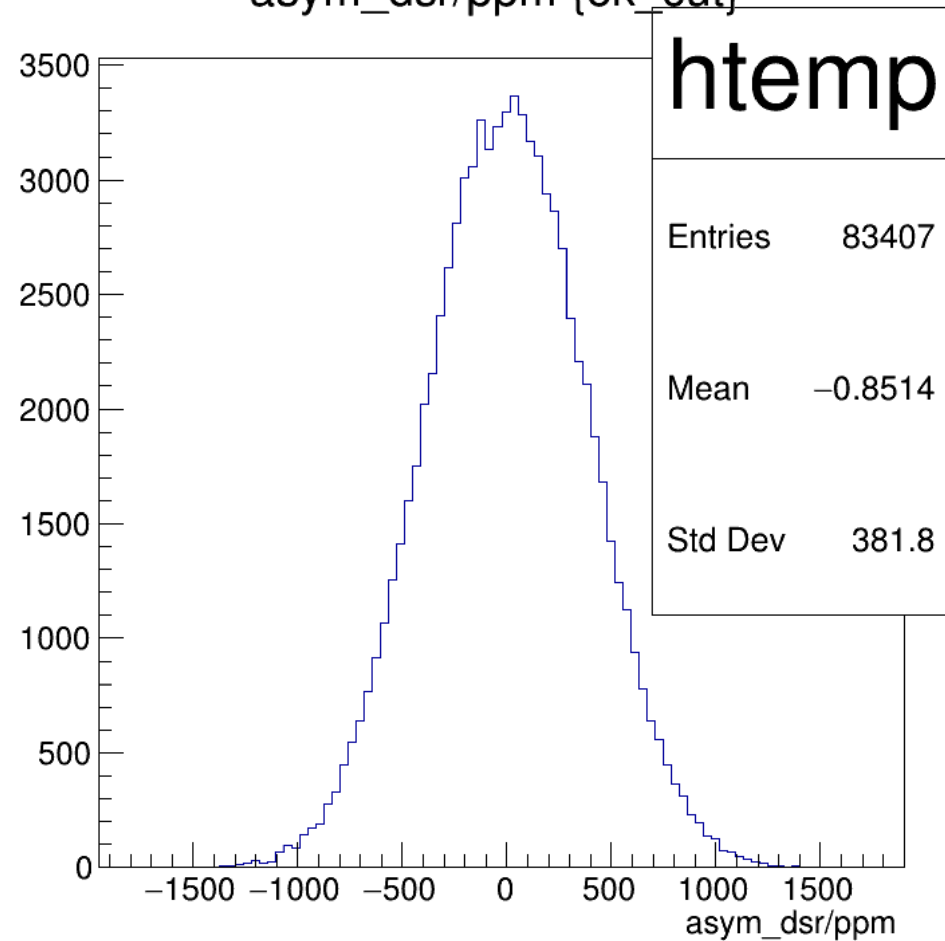
asym_dsr/ppm {ok_cut}
