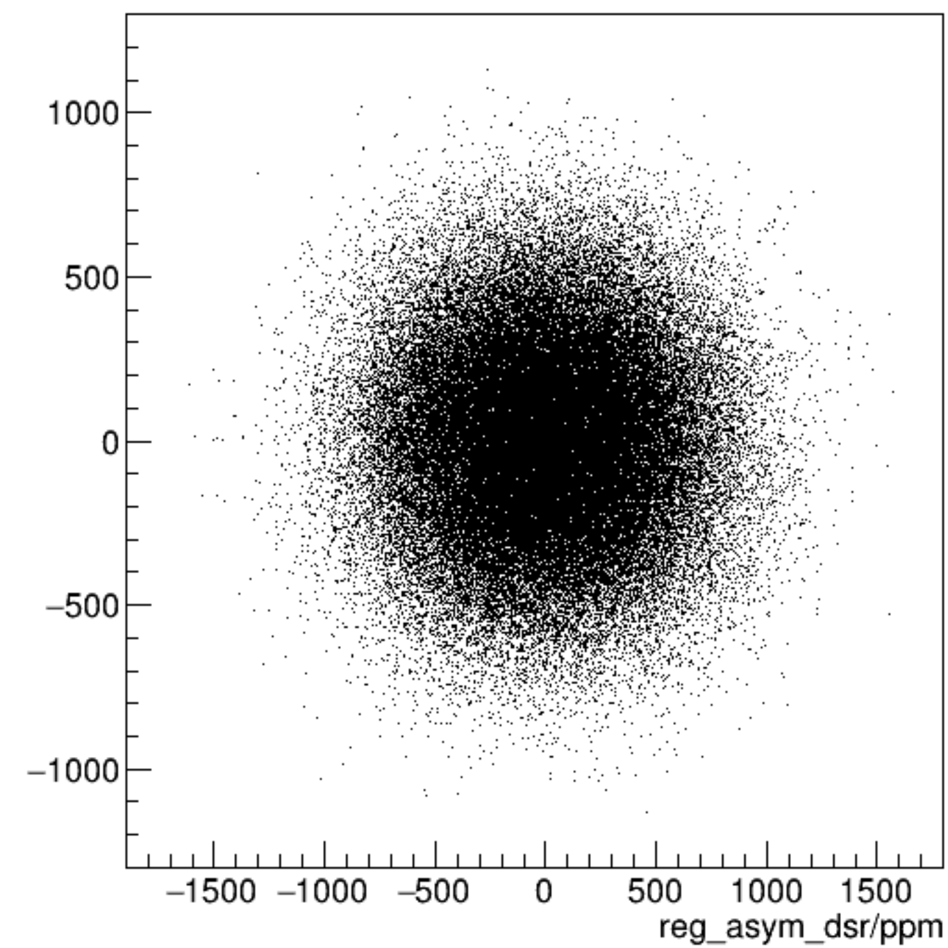
reg_asym_dsl/ppm:reg_asym_dsr/ppm {ok_cut}
