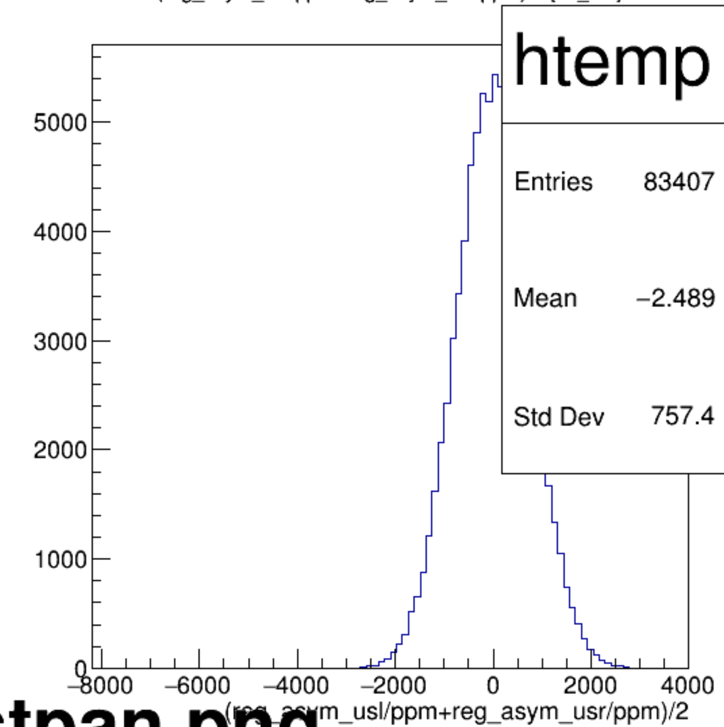
(reg_asym_usl/ppm+reg_asym_usr/ppm)/2 {ok_cut}
