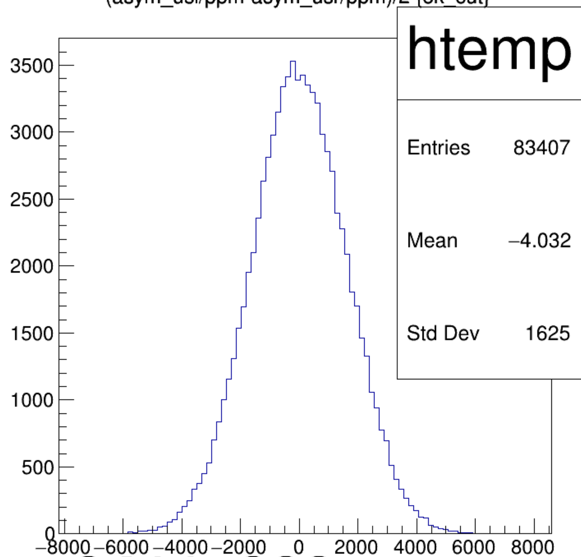
(asym_usl/ppm-asym_usr/ppm)/2 {ok_cut}
