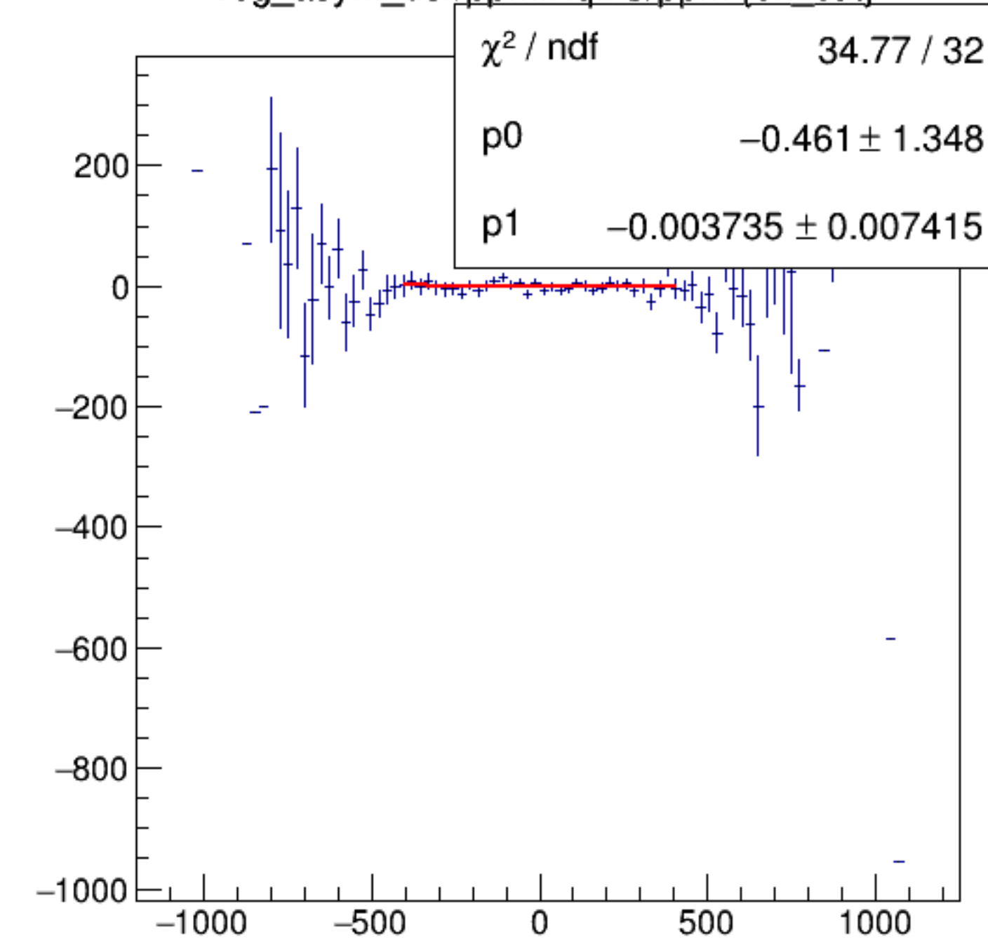
reg_asym_dsr/ppm:AqDS/ppm {ok_cut}
