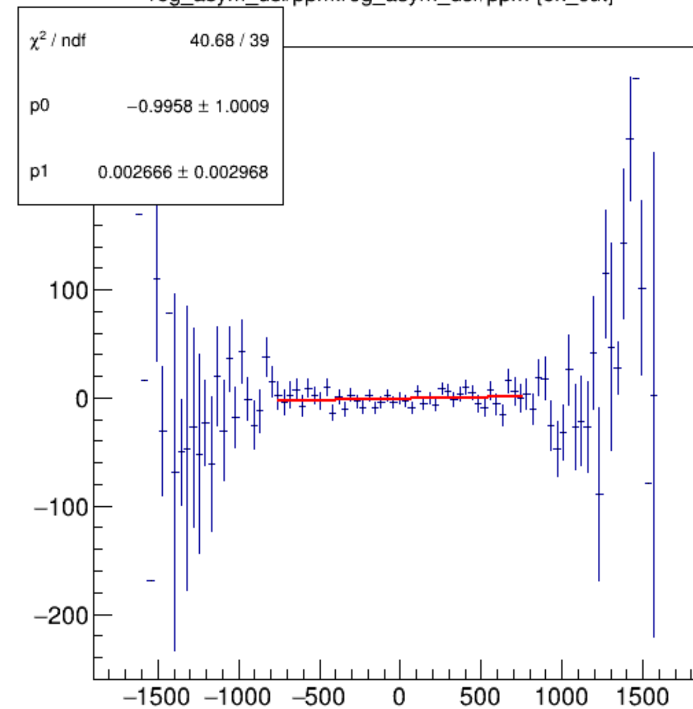
reg_asym_dsl/ppm:reg_asym_dsr/ppm {ok_cut}
