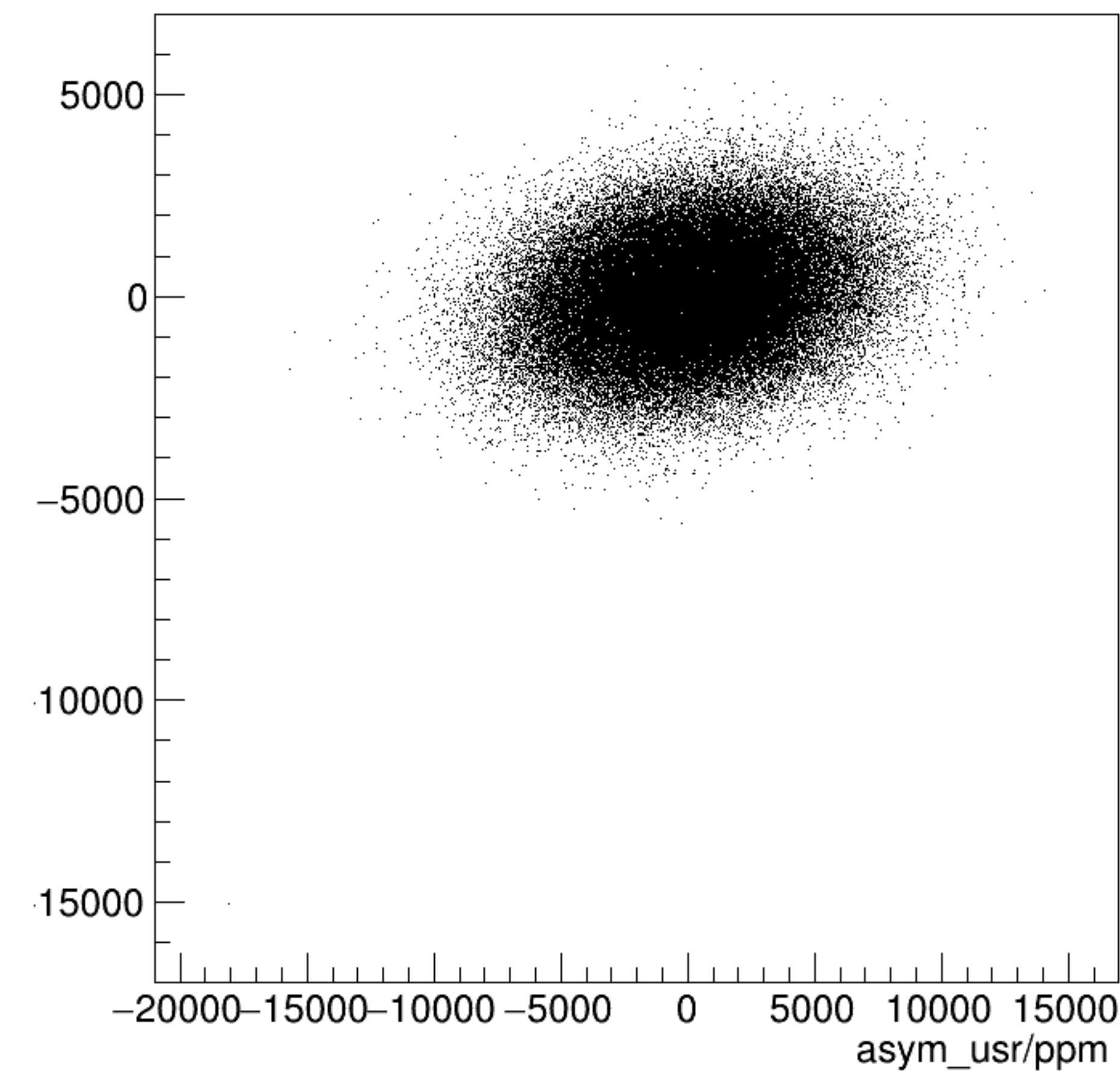
asym_usl/ppm:asym_usr/ppm {ok_cut}
