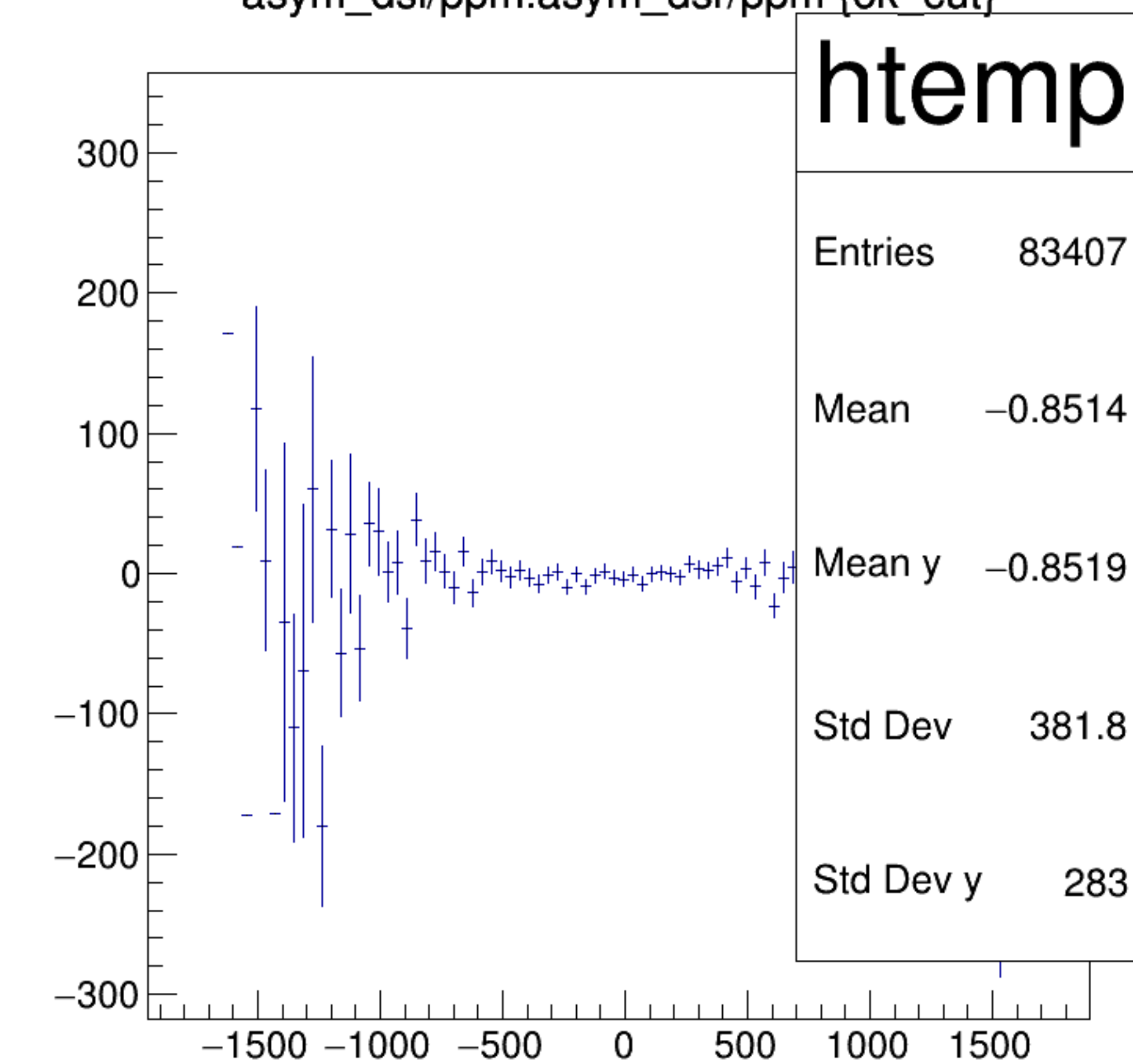
asym_dsl/ppm:asym_dsr/ppm {ok_cut}
