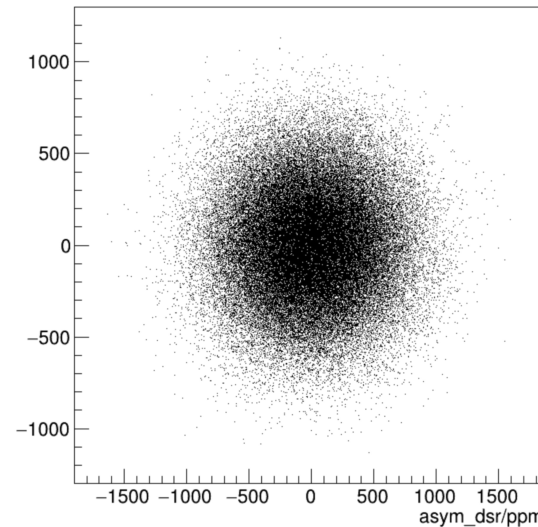
asym_dsl/ppm:asym_dsr/ppm {ok_cut}
