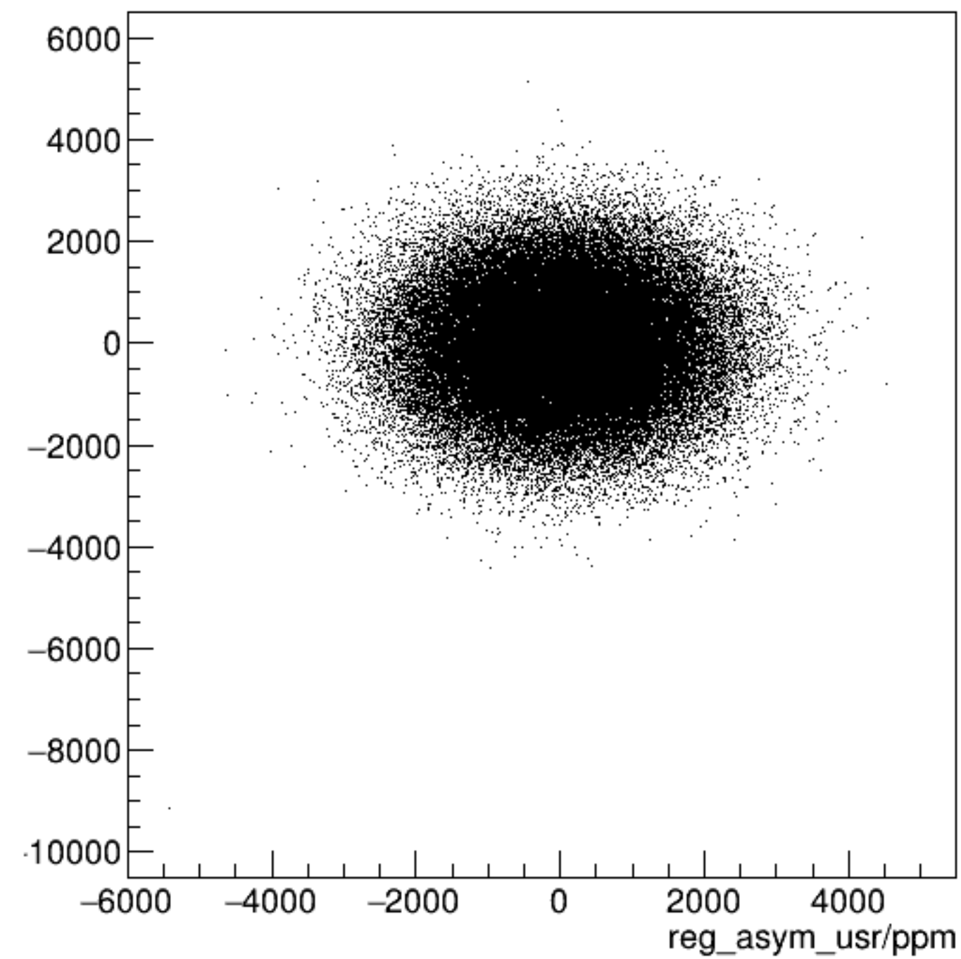
reg_asym_usl/ppm:reg_asym_usr/ppm {ok_cut}
