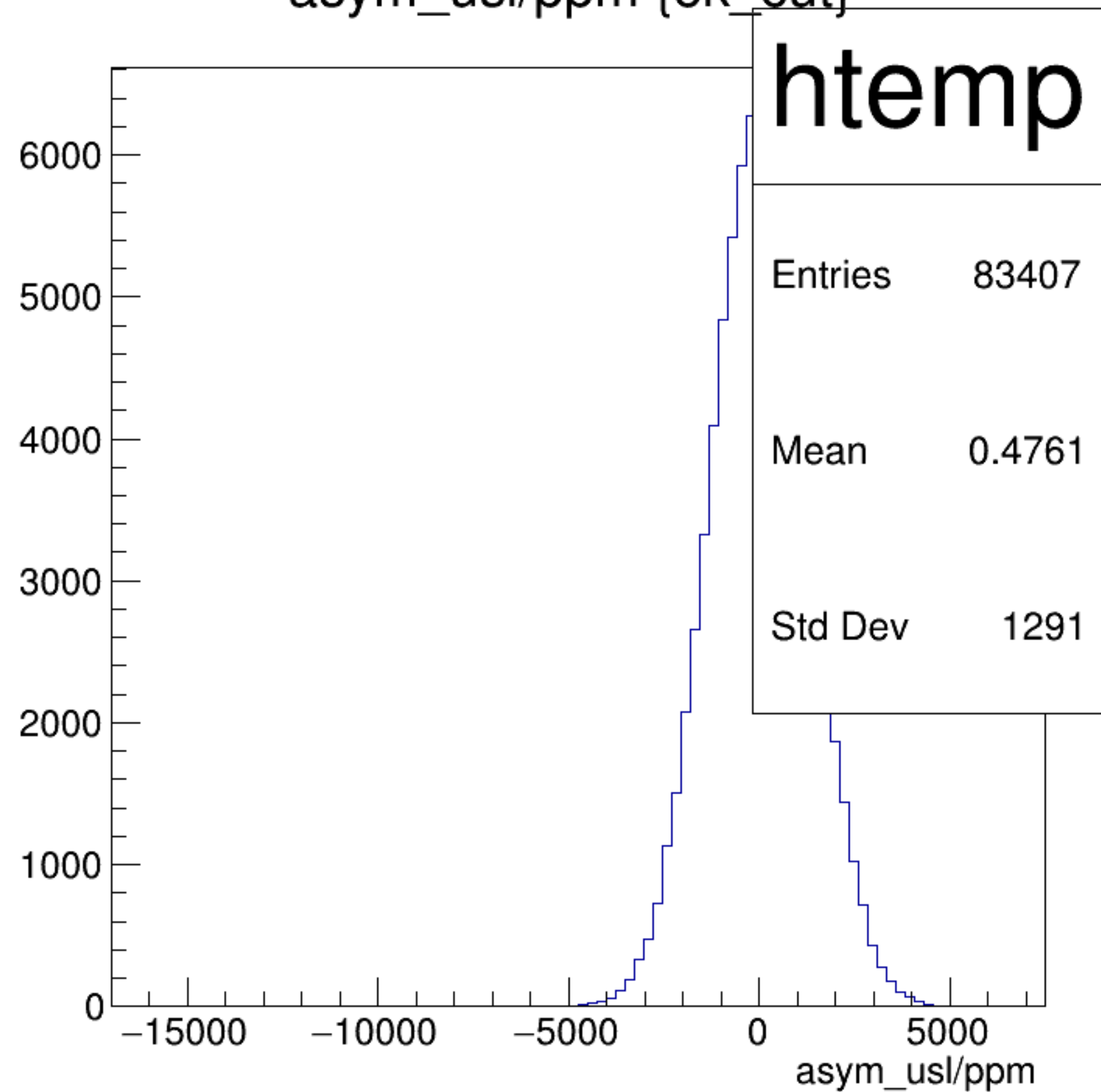
asym_usl/ppm {ok_cut}
