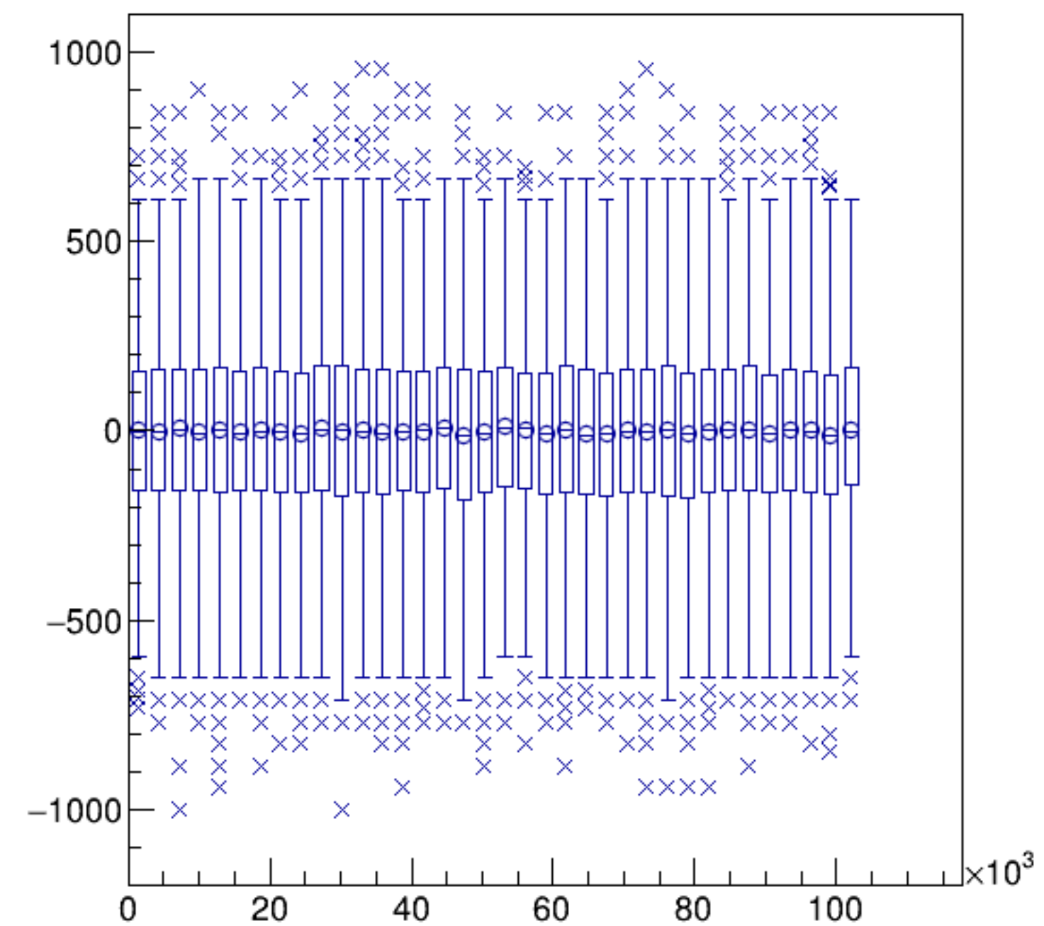
(reg_asym_dsl/ppm+reg_asym_dsr/ppm)/2:Entry$ {ok_cut}
