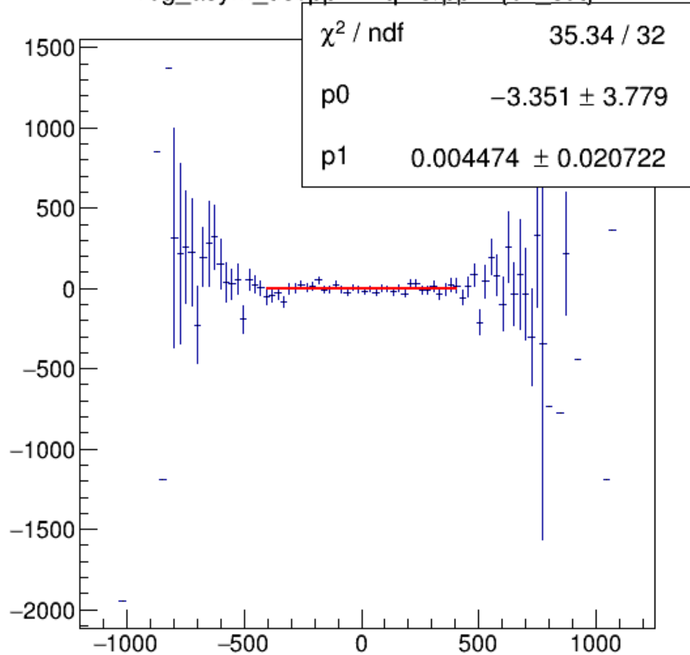
reg_asym_usl/ppm:AqDS/ppm {ok_cut}
