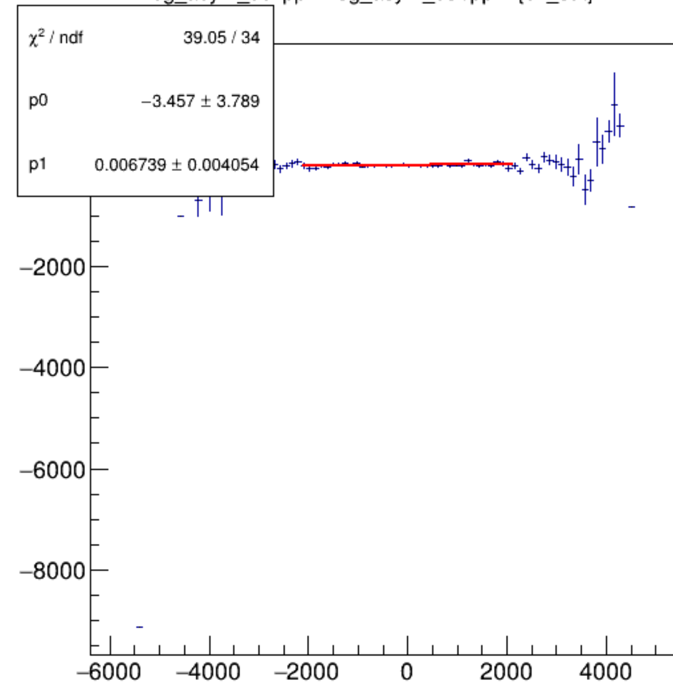
reg_asym_usl/ppm:reg_asym_usr/ppm {ok_cut}
