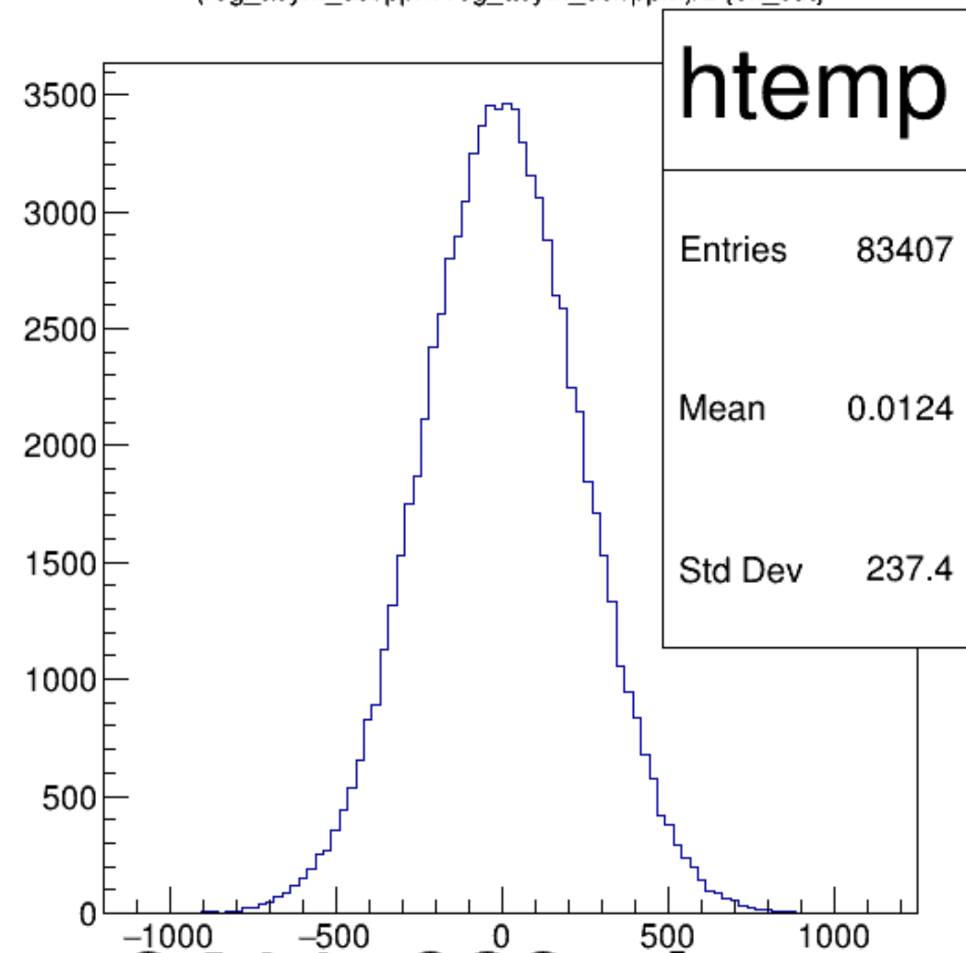
(reg_asym_dsl/ppm-reg_asym_dsr/ppm)/2 {ok_cut}
