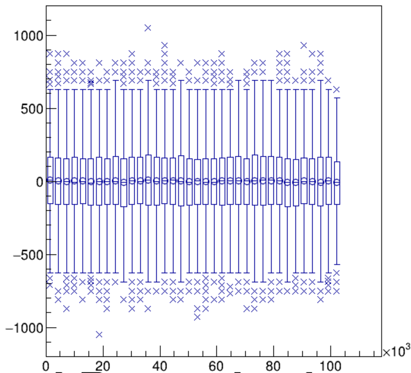
(reg_asym_dsl/ppm-reg_asym_dsr/ppm)/2:Entry$ {ok_cut}
