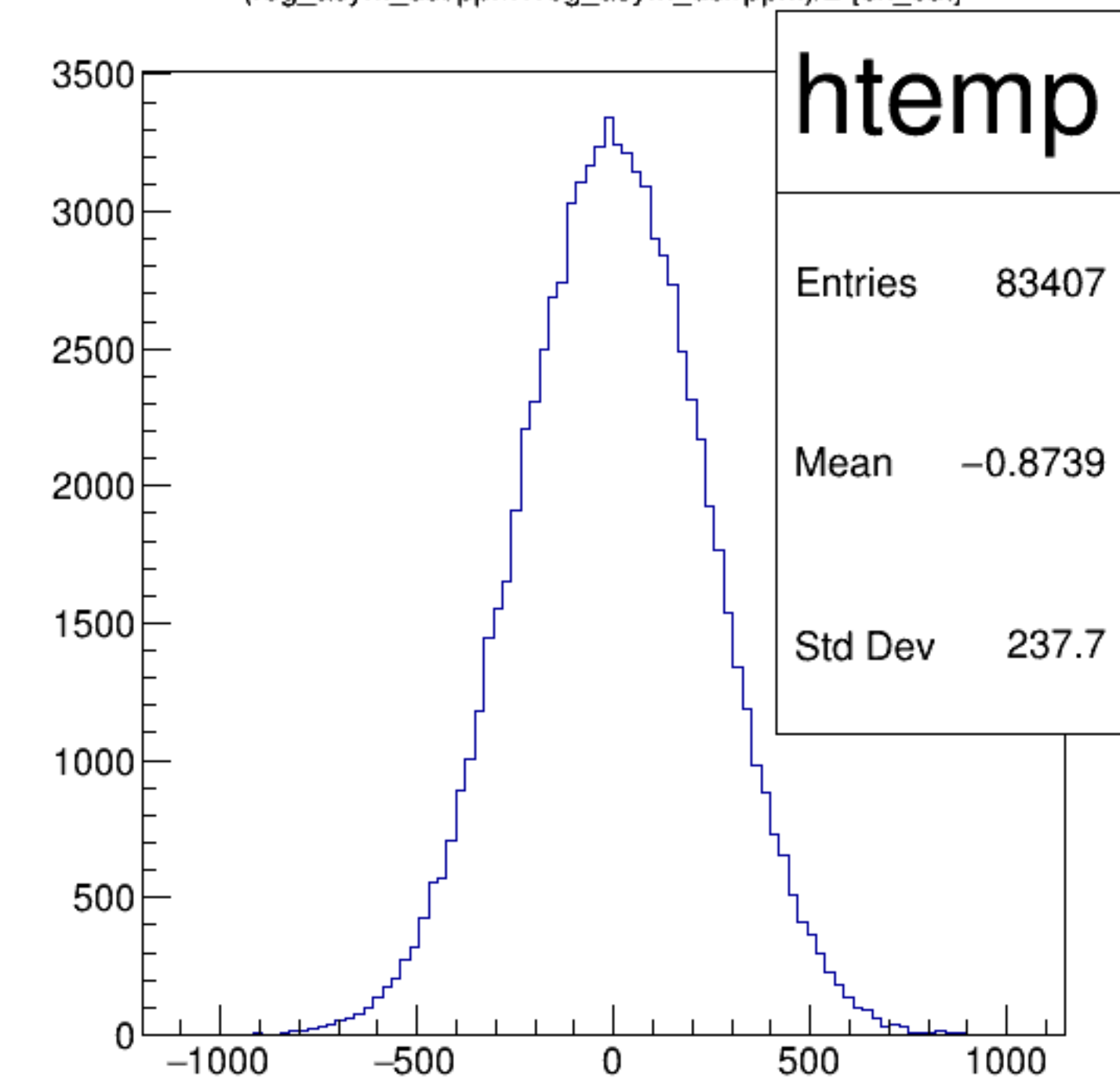
(reg_asym_dsl/ppm+reg_asym_dsr/ppm)/2 {ok_cut}
