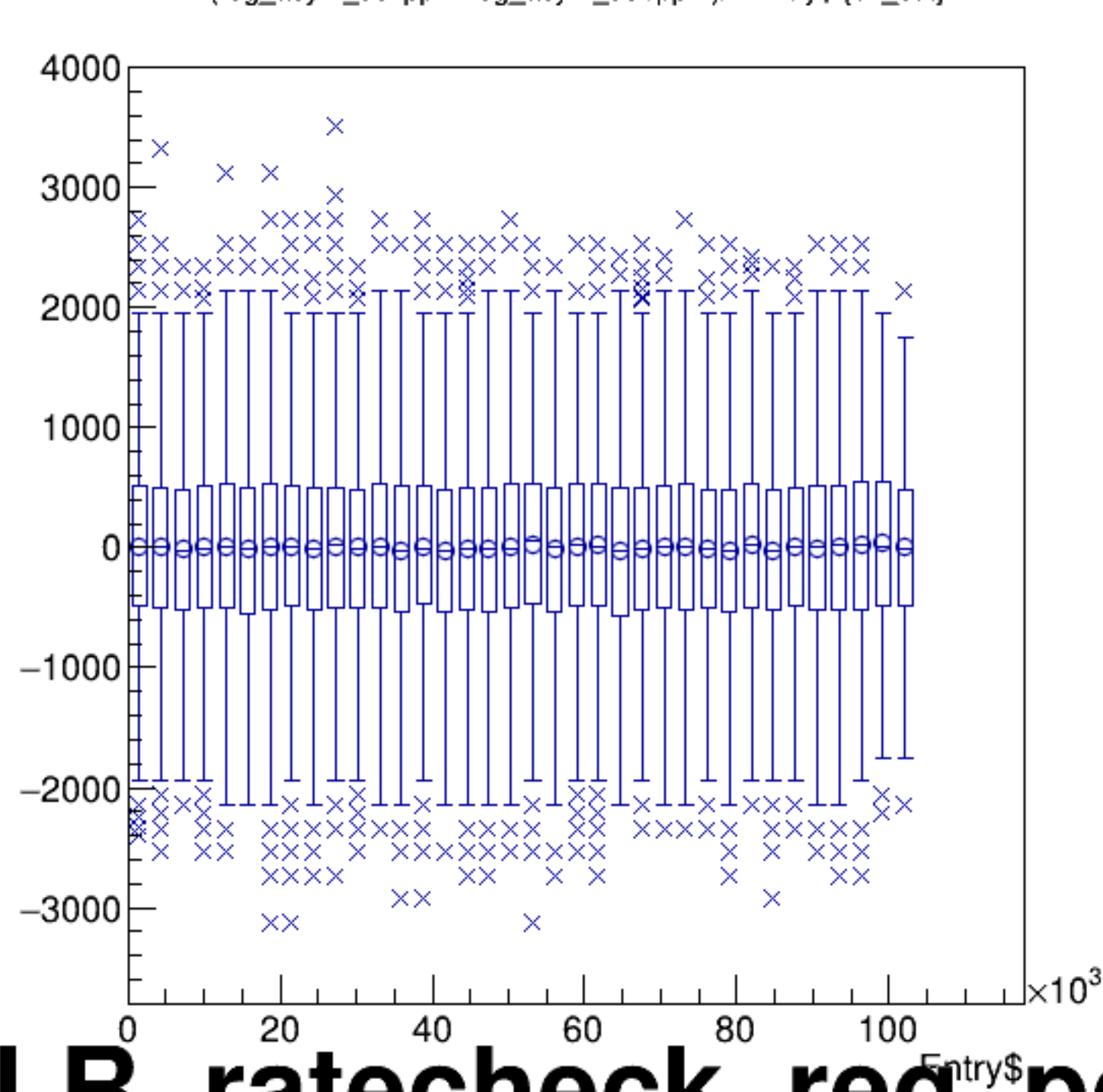
(reg_asym_usl/ppm-reg_asym_usr/ppm)/2:Entry$ {ok_cut}
