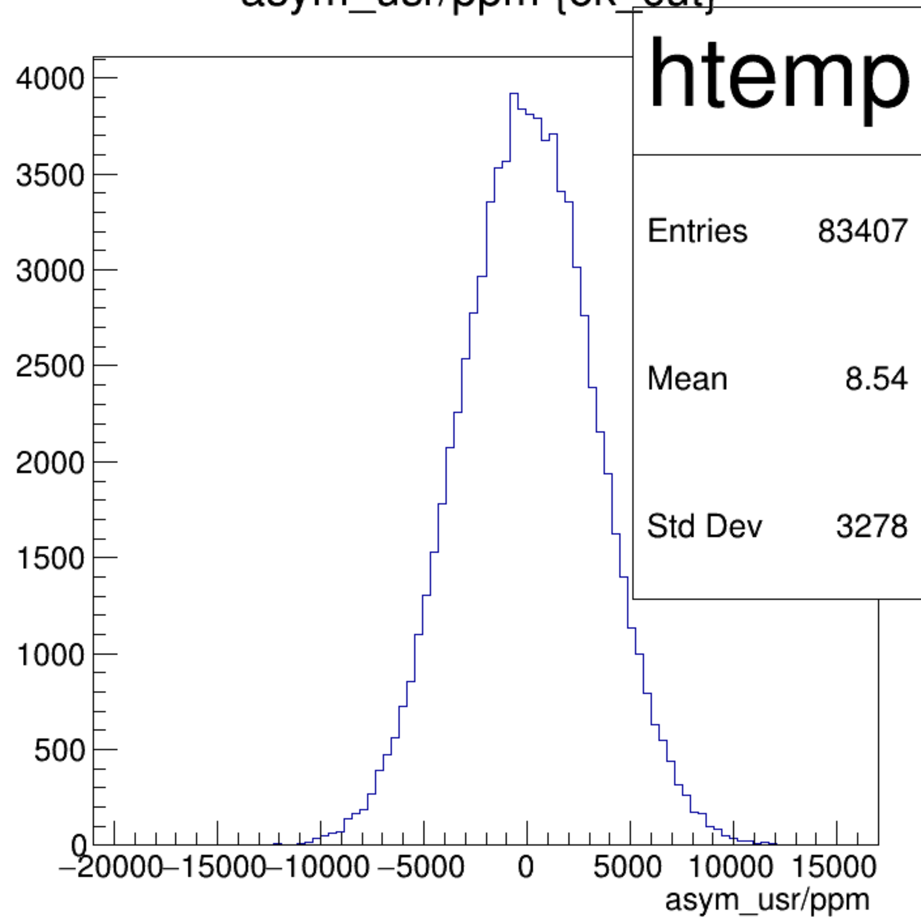
asym_usr/ppm {ok_cut}
