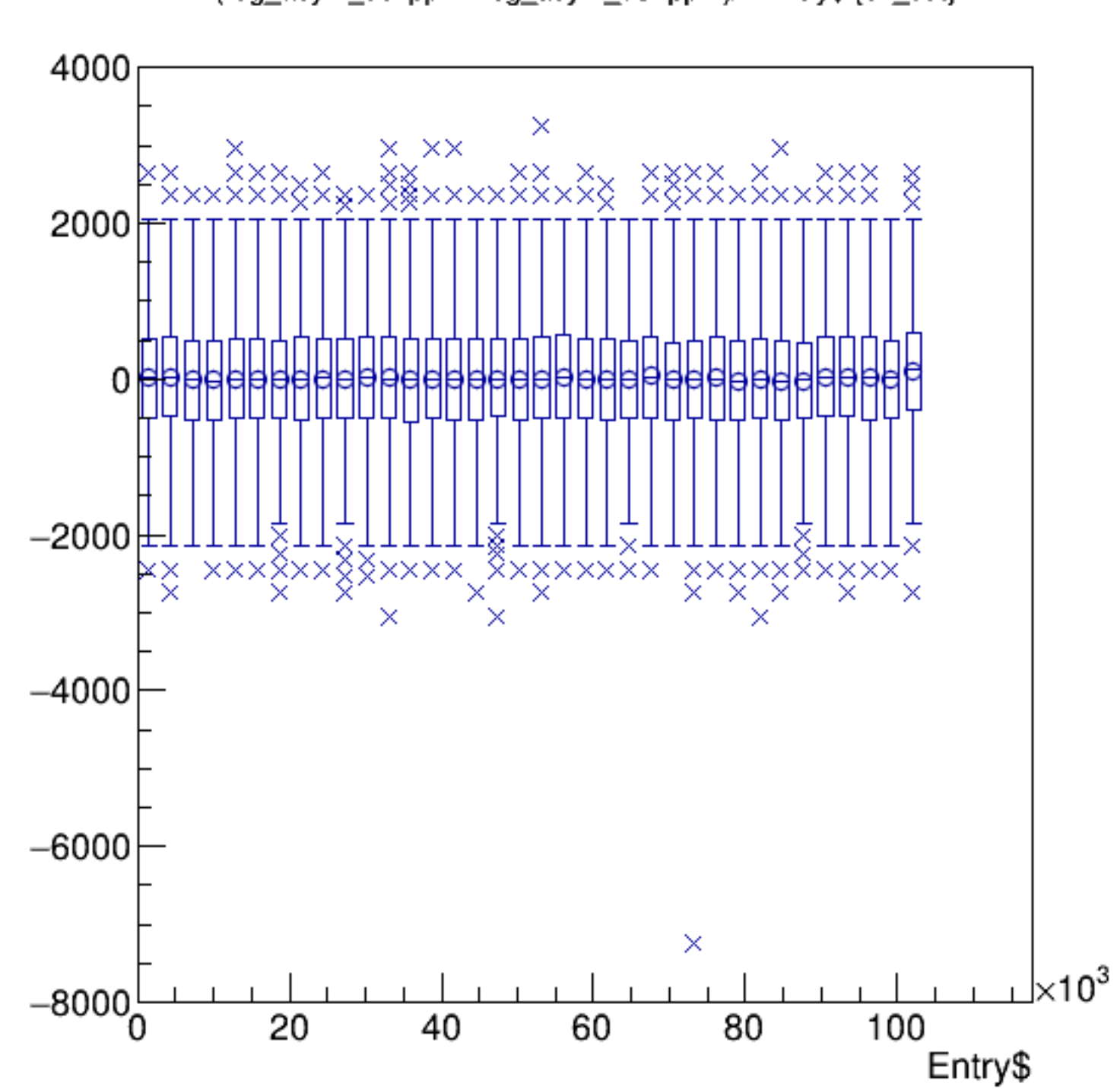
(reg_asym_usl/ppm+reg_asym_usr/ppm)/2:Entry$ {ok_cut}
