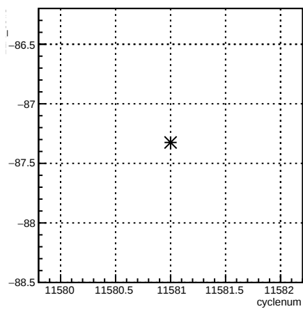
12X_coil3:cyclenum {run == 8413}
