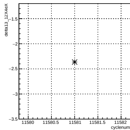
delta13_12X4eX:cyclenum {run == 8413}
