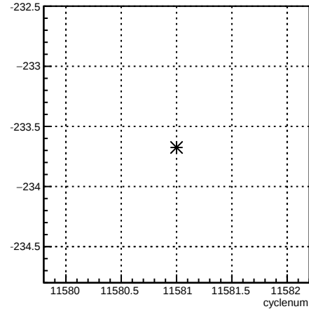
4eX_coil1:cyclenum {run == 8413}
