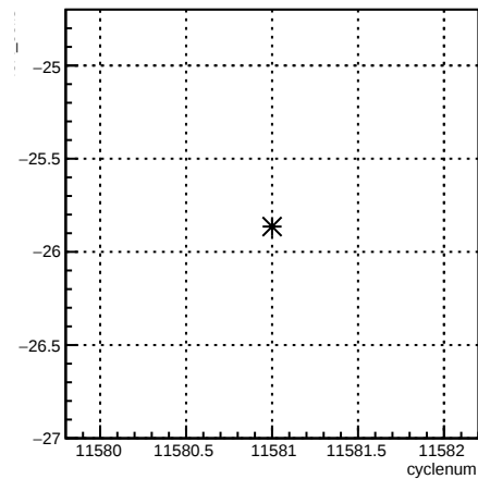
4eX_coil3:cyclenum {run == 8413}
