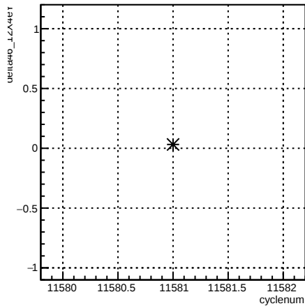
delta46_12X4eY:cyclenum {run == 8413}
