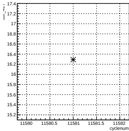
usr_4eY:cyclenum {run == 8413}
