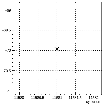
usl_4eY:cyclenum {run == 8413}
