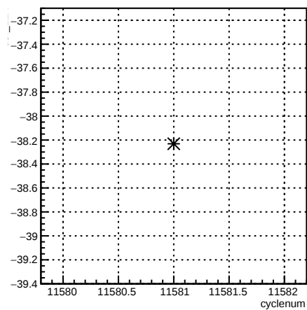
usr_12X:cyclenum {run == 8413}
