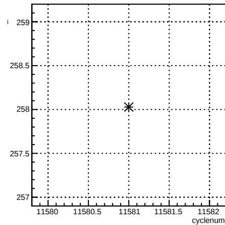
4eX_coil7:cyclenum {run == 8413}
