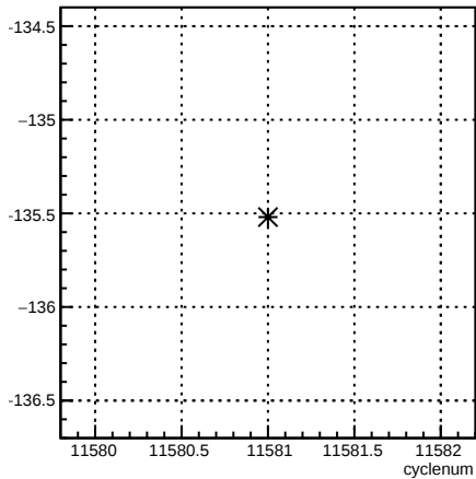
4eY_coil6:cyclenum {run == 8413}
