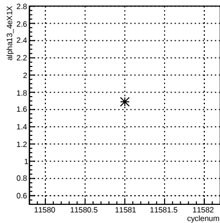
alpha13_4eX1X:cyclenum {run == 8413}
