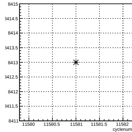
run:cyclenum {run == 8413}
