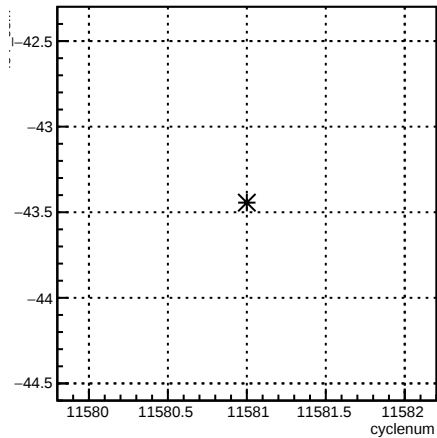
4eY_coil7:cyclenum {run == 8413}
