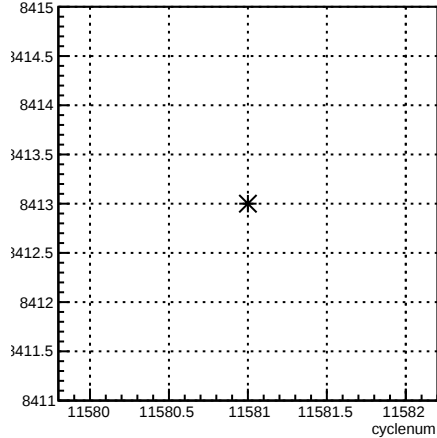
run:cyclenum {run == 8413}
