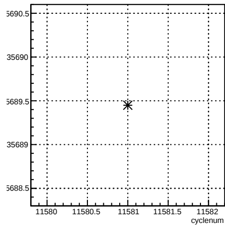
usr_coil7:cyclenum {run == 8413}
