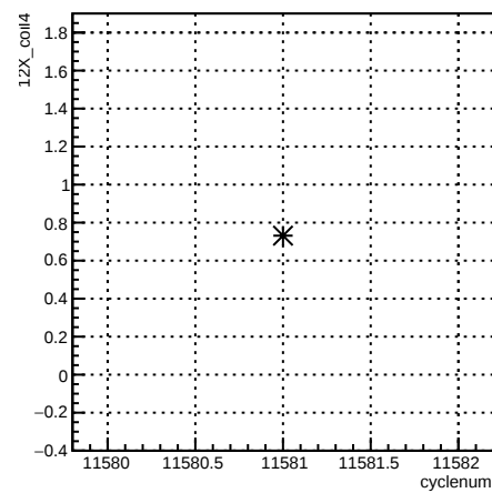
12X_coil4:cyclenum {run == 8413}
