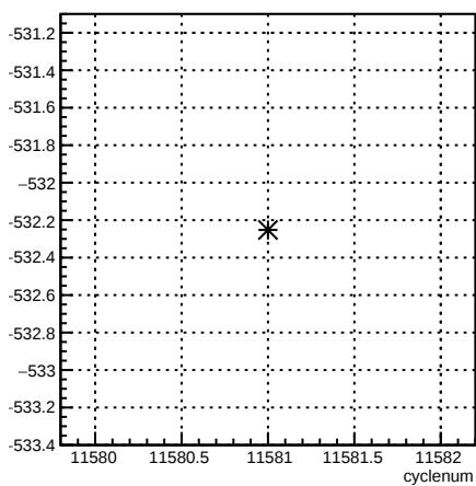
12X_coil7:cyclenum {run == 8413}
