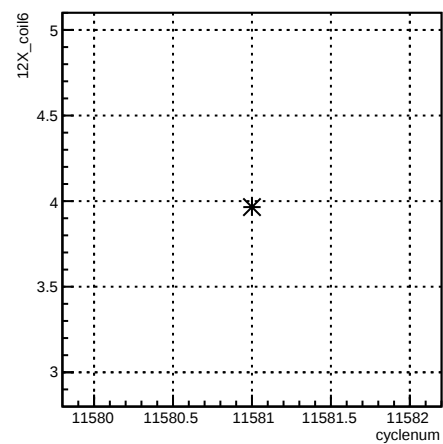
12X_coil6:cyclenum {run == 8413}
