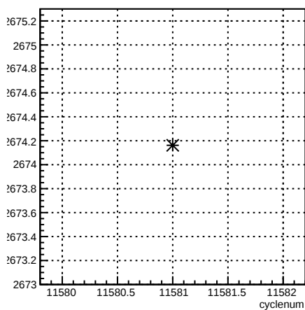
usl_coil7:cyclenum {run == 8413}
