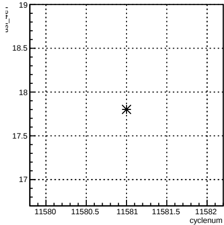
usl_4eY:cyclenum {run == 8413}
