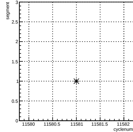
segment:cyclenum {run == 8413}
