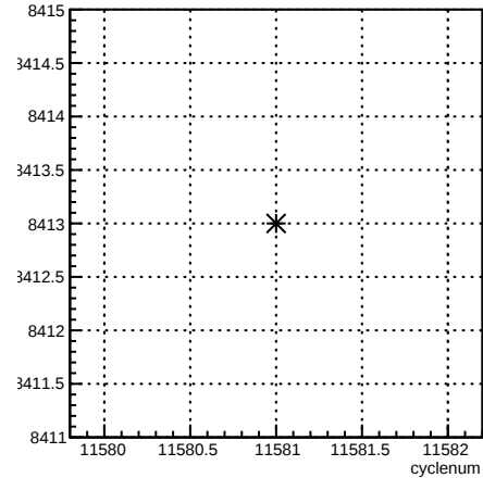
run:cyclenum {run == 8413}
