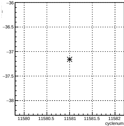
usl_12X:cyclenum {run == 8413}
