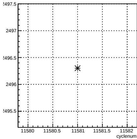
usl_coil3:cyclenum {run == 8413}
