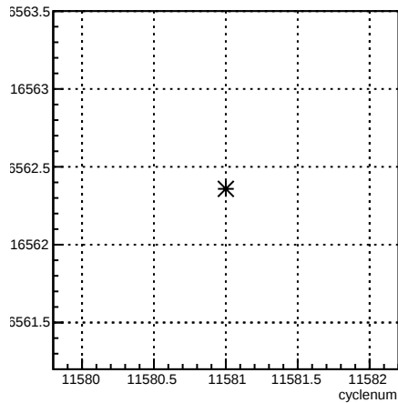
usl_coil1:cyclenum {run == 8413}
