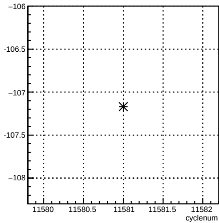
4aY_coil6:cyclenum {run == 8413}
