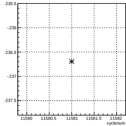
12X_coil1:cyclenum {run == 8413}
