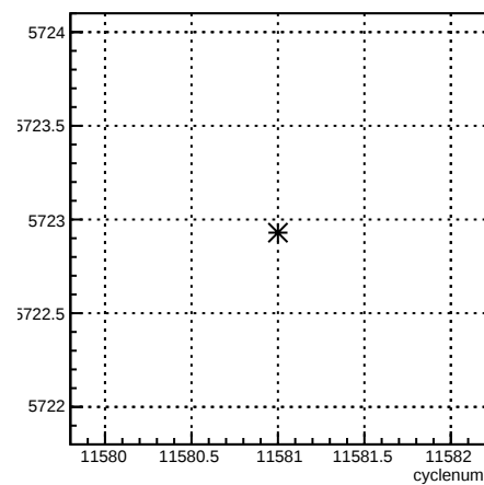
usl_coil4:cyclenum {run == 8413}
