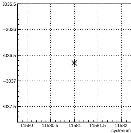
usl_coil6:cyclenum {run == 8413}
