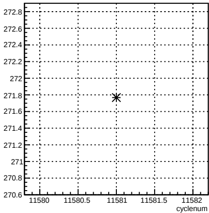
4eY_coil4:cyclenum {run == 8413}
