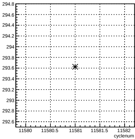
4aY_coil4:cyclenum {run == 8413}
