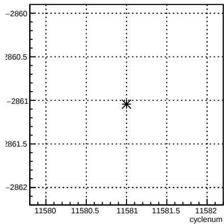
usr_coil6:cyclenum {run == 8413}
