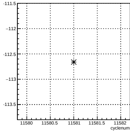
usr_1X:cyclenum {run == 8413}
