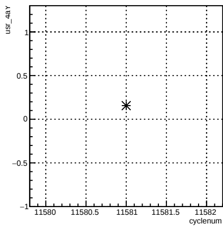
usr_4aY:cyclenum {run == 8413}
