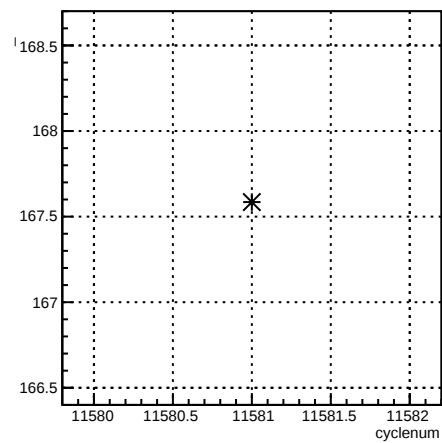
usr_4eX:cyclenum {run == 8413}
