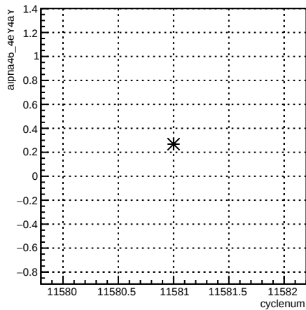
alpha46_4eY4aY:cyclenum {run == 8413}
