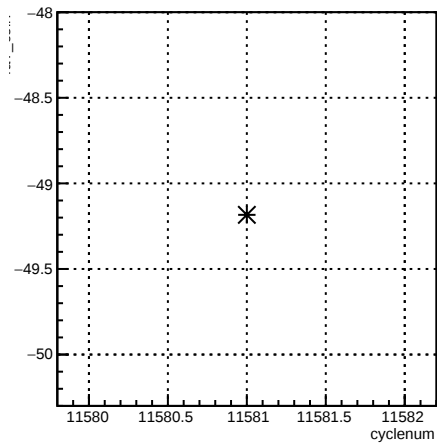
4aY_coil7:cyclenum {run == 8413}
