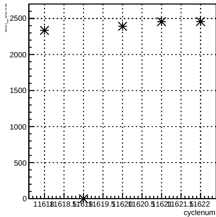
usl_coil7:cyclenum {run == 8421}
