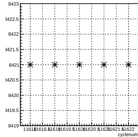
run:cyclenum {run == 8421}
