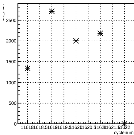
usl_coil7:cyclenum {run == 8421}
