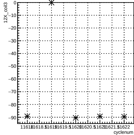
12X_coil3:cyclenum {run == 8421}
