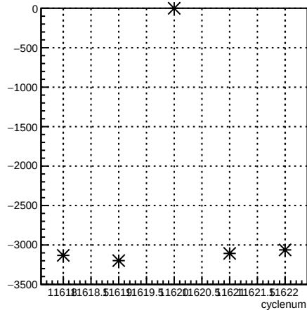
usl_coil6:cyclenum {run == 8421}
