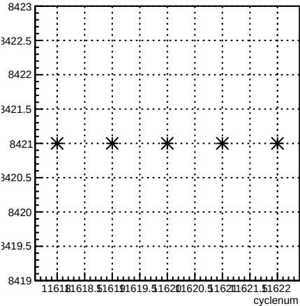
run:cyclenum {run == 8421}
