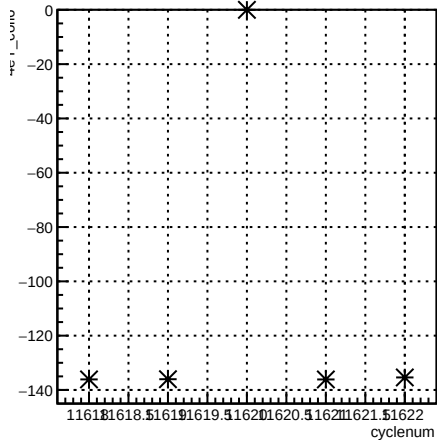
4eY_coil6:cyclenum {run == 8421}
