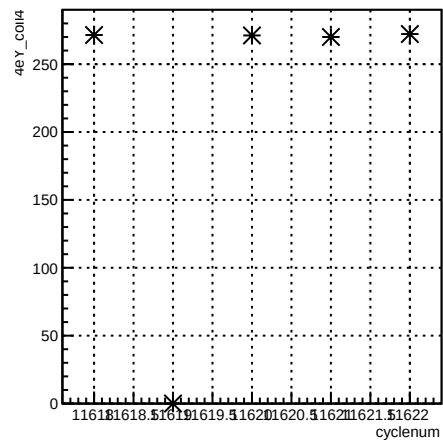
4eY_coil4:cyclenum {run == 8421}
