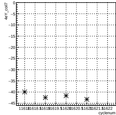
4eY_coil7:cyclenum {run == 8421}
