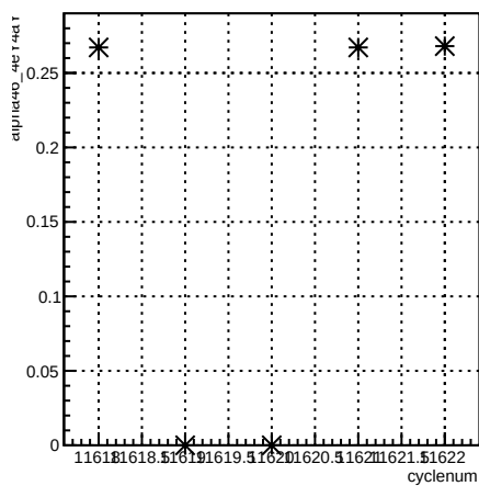
alpha46_4eY4aY:cyclenum {run == 8421}
