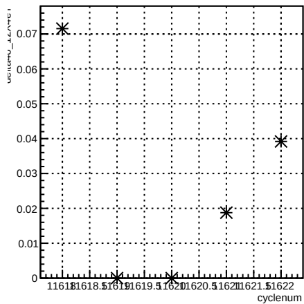
delta46_12X4eY:cyclenum {run == 8421}
