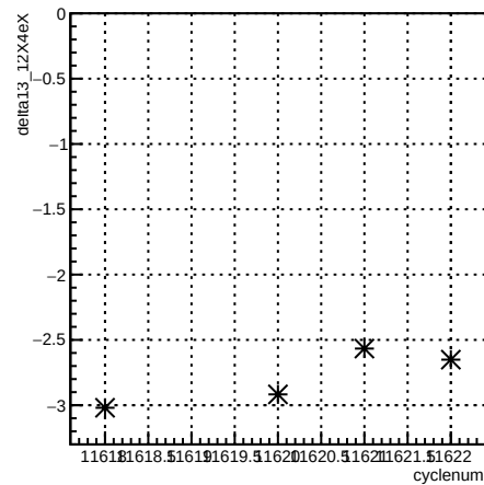
delta13_12X4eX:cyclenum {run == 8421}
