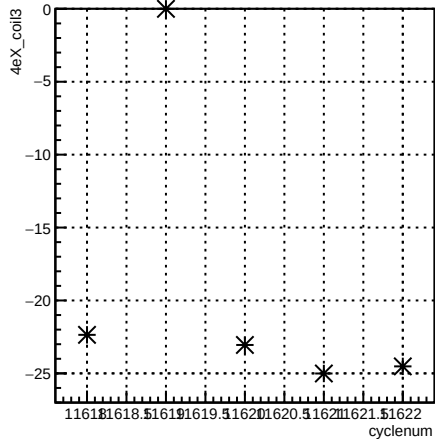
4eX_coil3:cyclenum {run == 8421}
