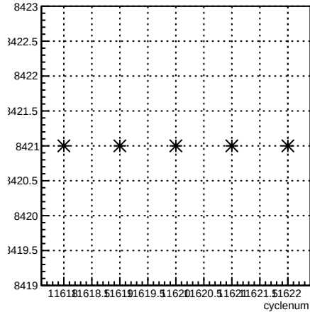
run:cyclenum {run == 8421}
