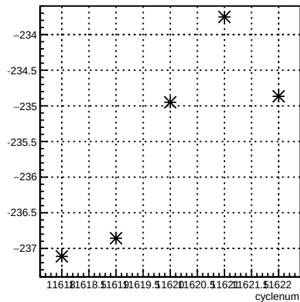
4eX_coil1:cyclenum {run == 8421}
