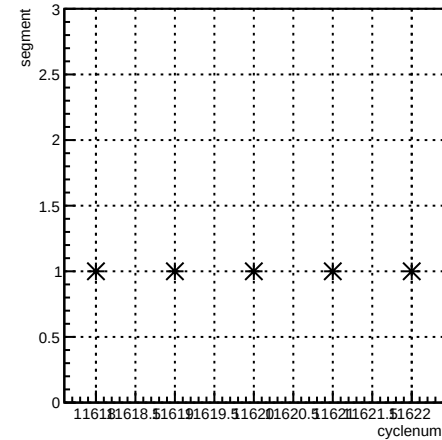
segment:cyclenum {run == 8421}
