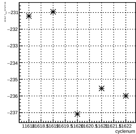
12X_coil1:cyclenum {run == 8421}
