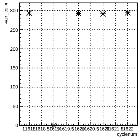
4aY_coil4:cyclenum {run == 8421}
