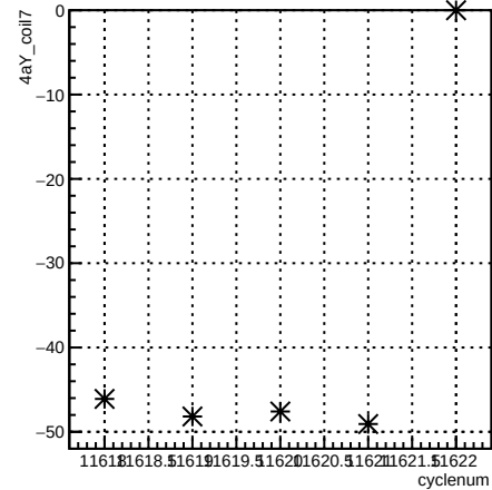
4aY_coil7:cyclenum {run == 8421}
