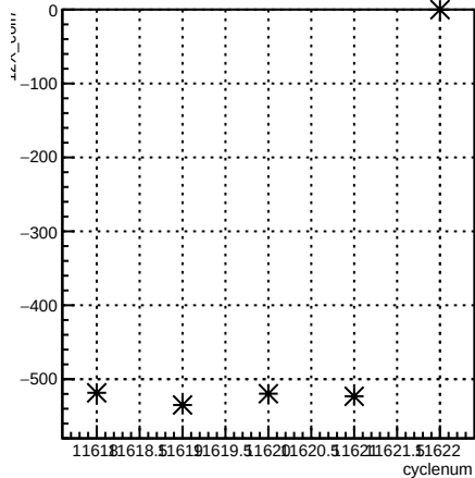
12X_coil7:cyclenum {run == 8421}
