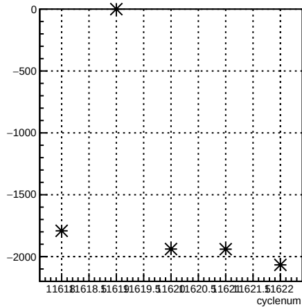
usr_coil3:cyclenum {run == 8421}
