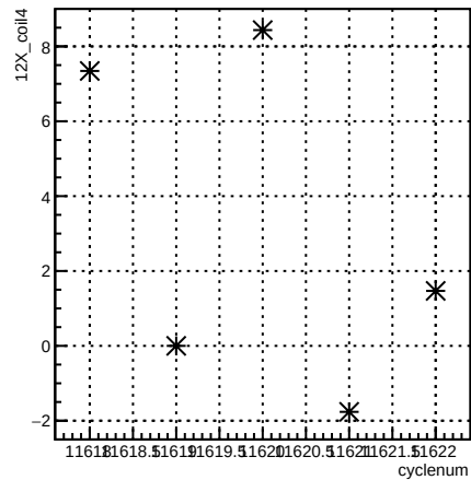
12X_coil4:cyclenum {run == 8421}
