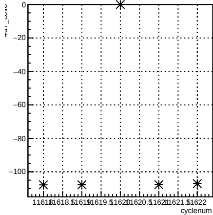
4aY_coil6:cyclenum {run == 8421}
