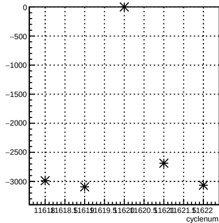
usr_coil6:cyclenum {run == 8421}
