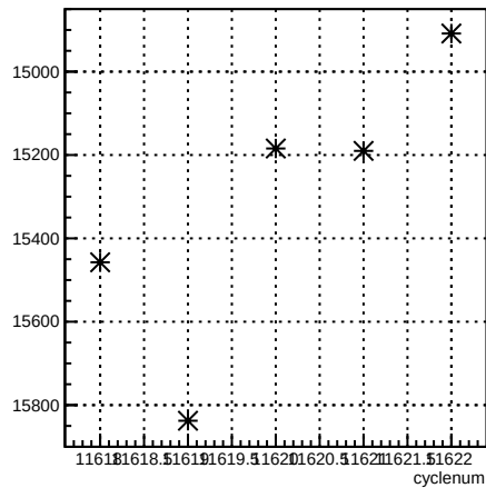
usr_coil6:cyclenum {run == 8421}
