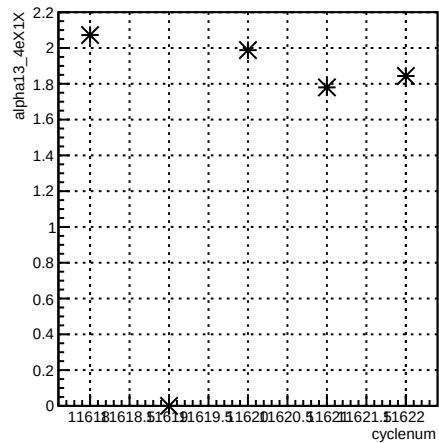
alpha13_4eX1X:cyclenum {run == 8421}
