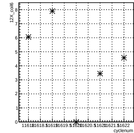
12X_coil6:cyclenum {run == 8421}
