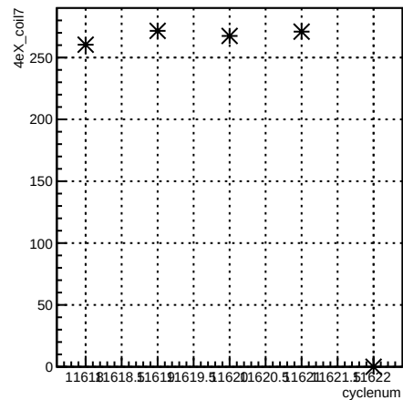
4eX_coil7:cyclenum {run == 8421}
