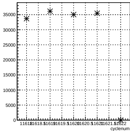
usr_coil7:cyclenum {run == 8421}
