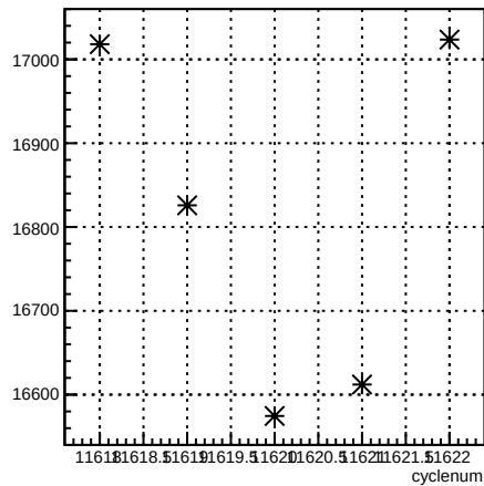
usl_coil6:cyclenum {run == 8421}
