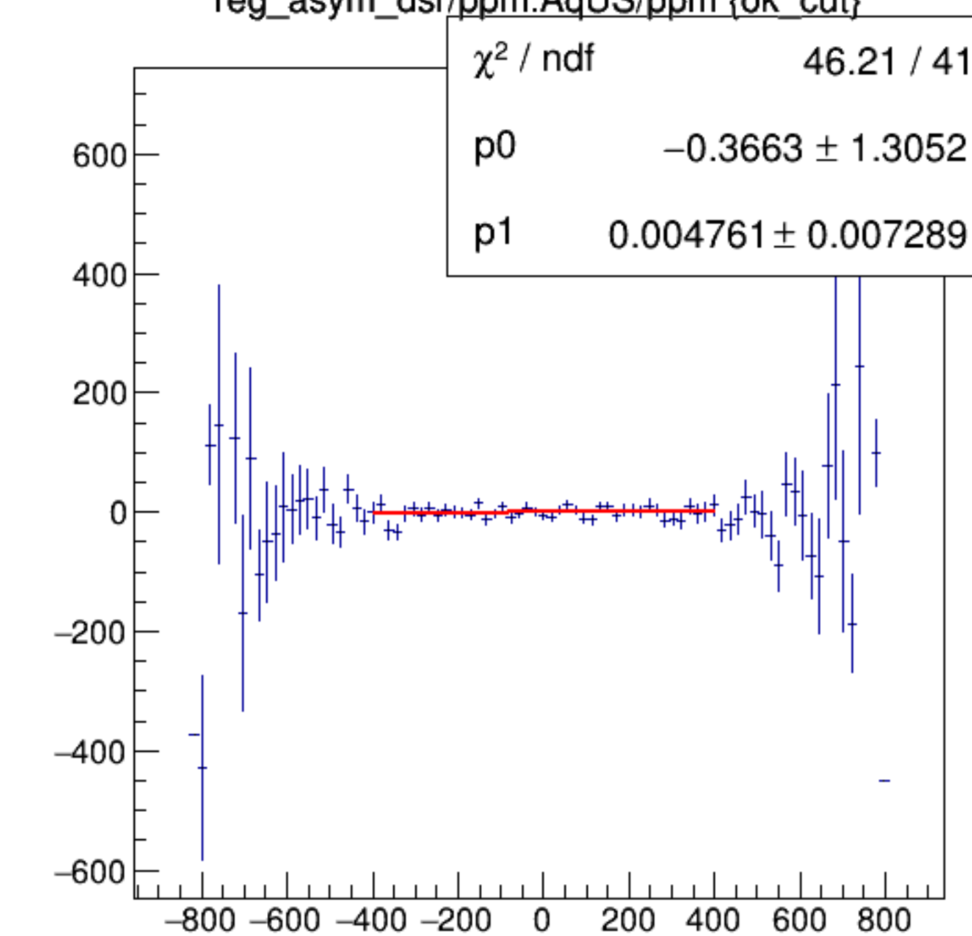
reg_asym_dsr/ppm:AqUS/ppm {ok_cut}
