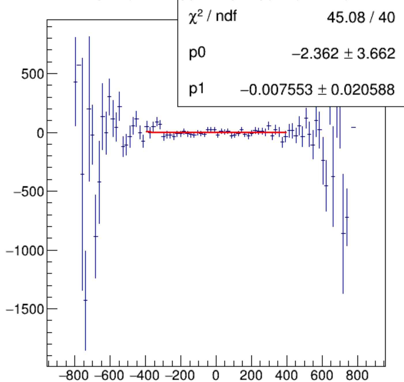
reg_asym_usl/ppm:AqDS/ppm {ok_cut}
