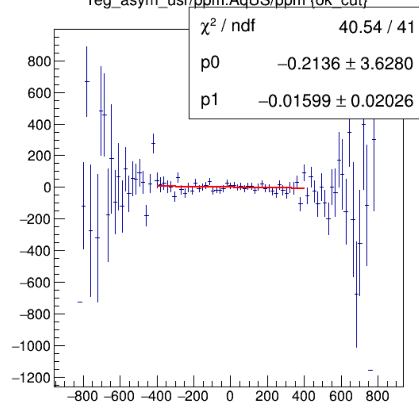
reg_asym_usr/ppm:AqUS/ppm {ok_cut}
