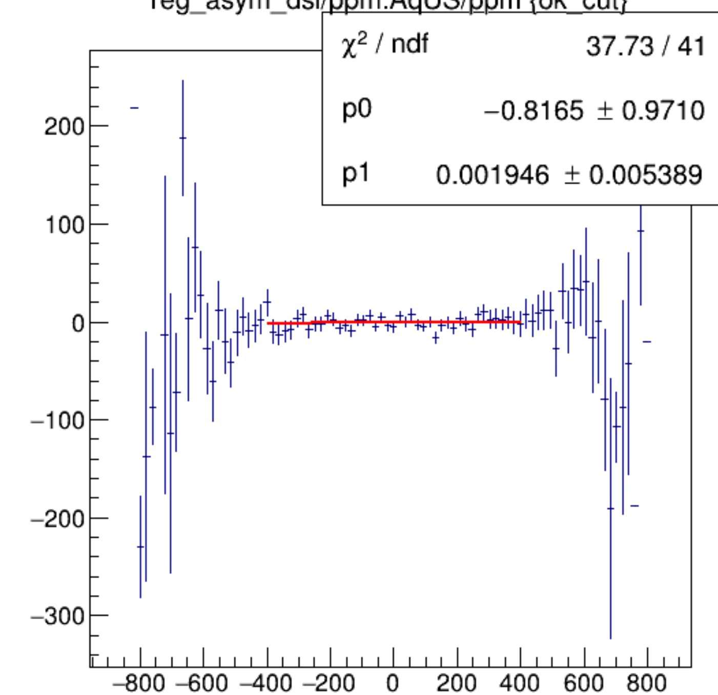
reg_asym_dsl/ppm:AqUS/ppm {ok_cut}
