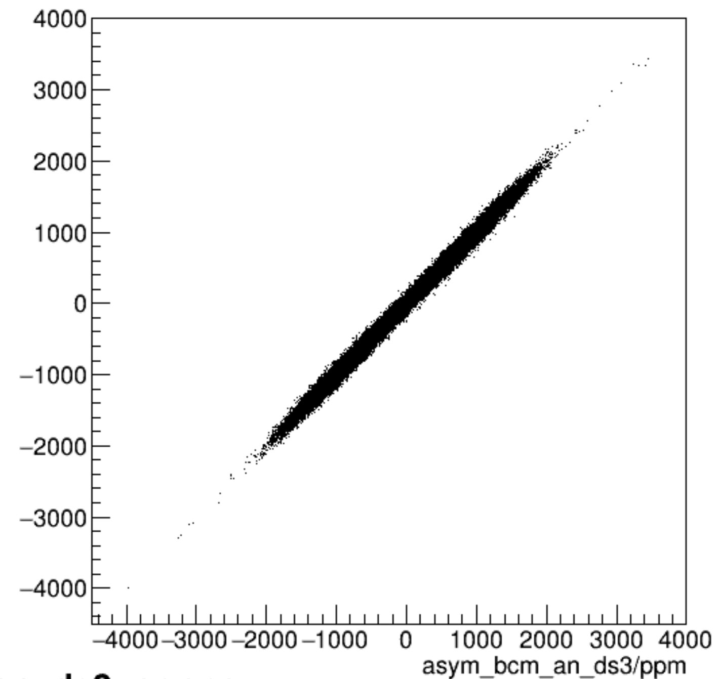
run8398_000_asym_bcm_dg_us_vs_asym_bcm_an_ds3_pr.png
