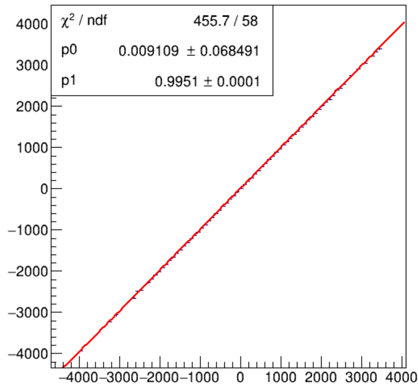
run8398_000_asym_bcm_an_ds_vs_asym_bcm_an_ds3_pr.png
