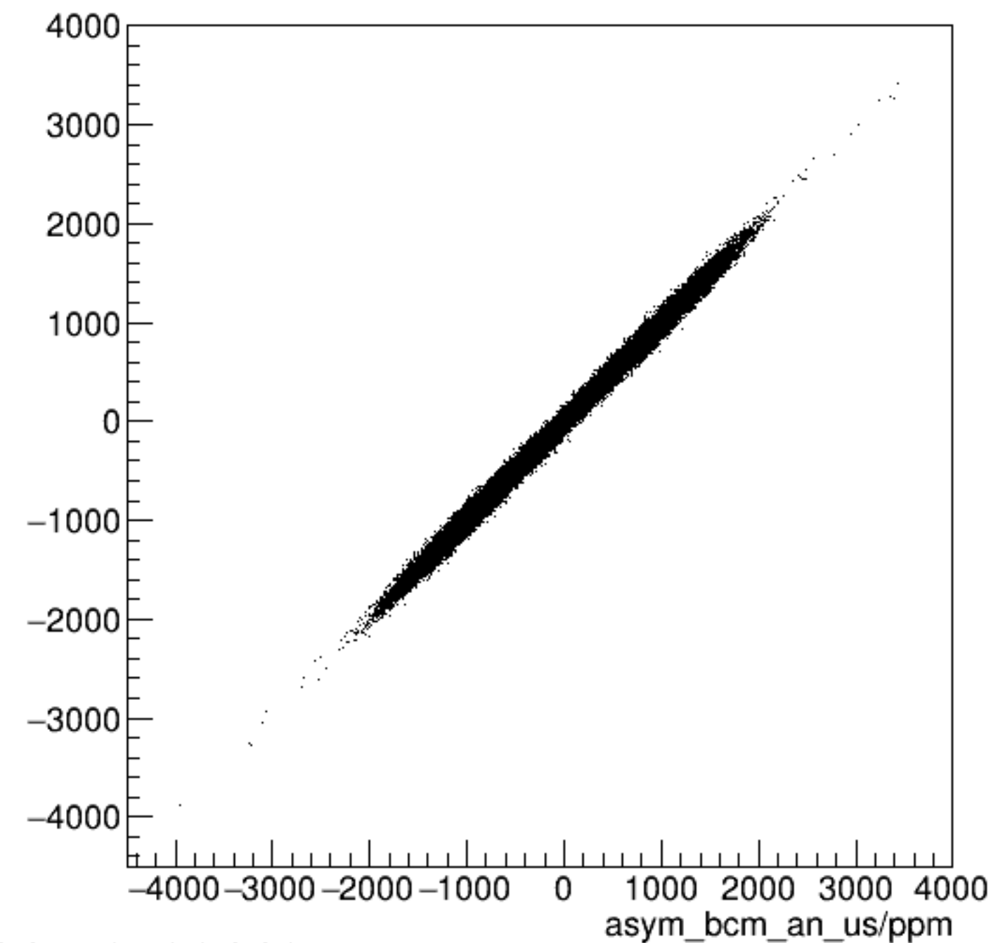
run8398_000_asym_bcm_dg_ds_vs_asym_bcm_an_us_pr.png
