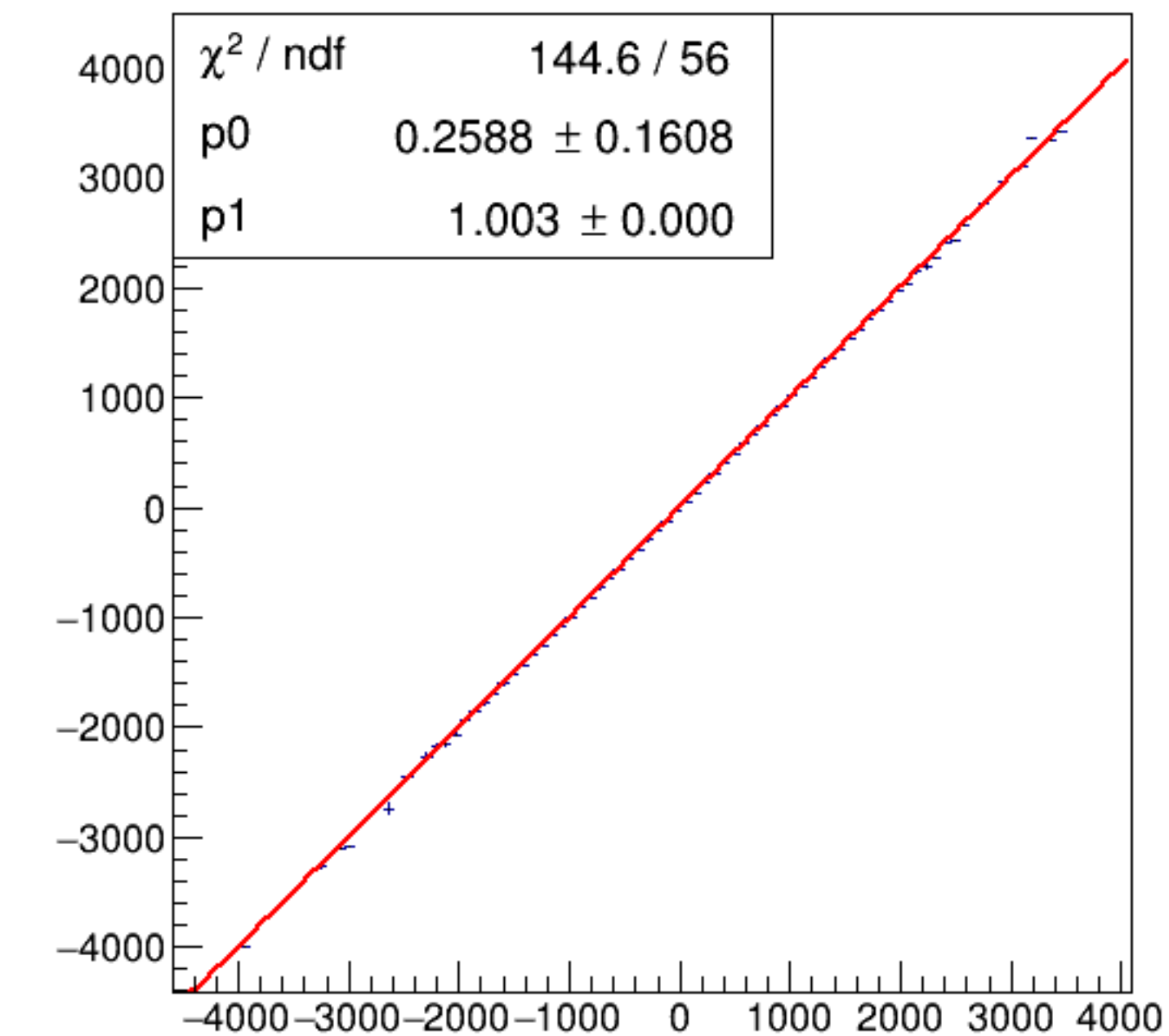
run8398_000_asym_bcm_dg_us_vs_asym_bcm_an_ds_pr.png
