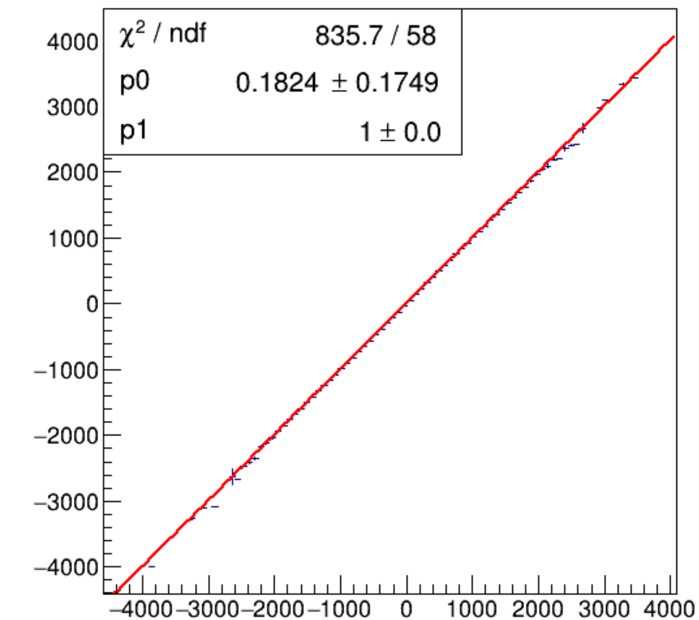
run8398_000_asym_bcm_dg_us_vs_asym_bcm_dg_ds_pr.png
