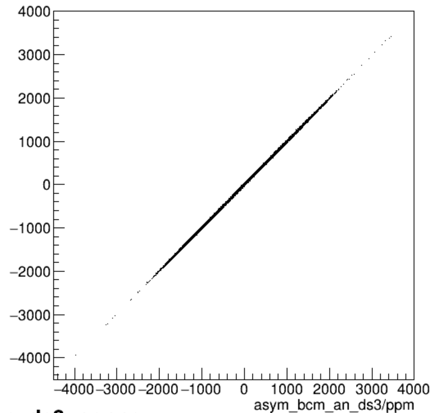
run8398_000_asym_bcm_an_ds_vs_asym_bcm_an_ds3_pr.png
