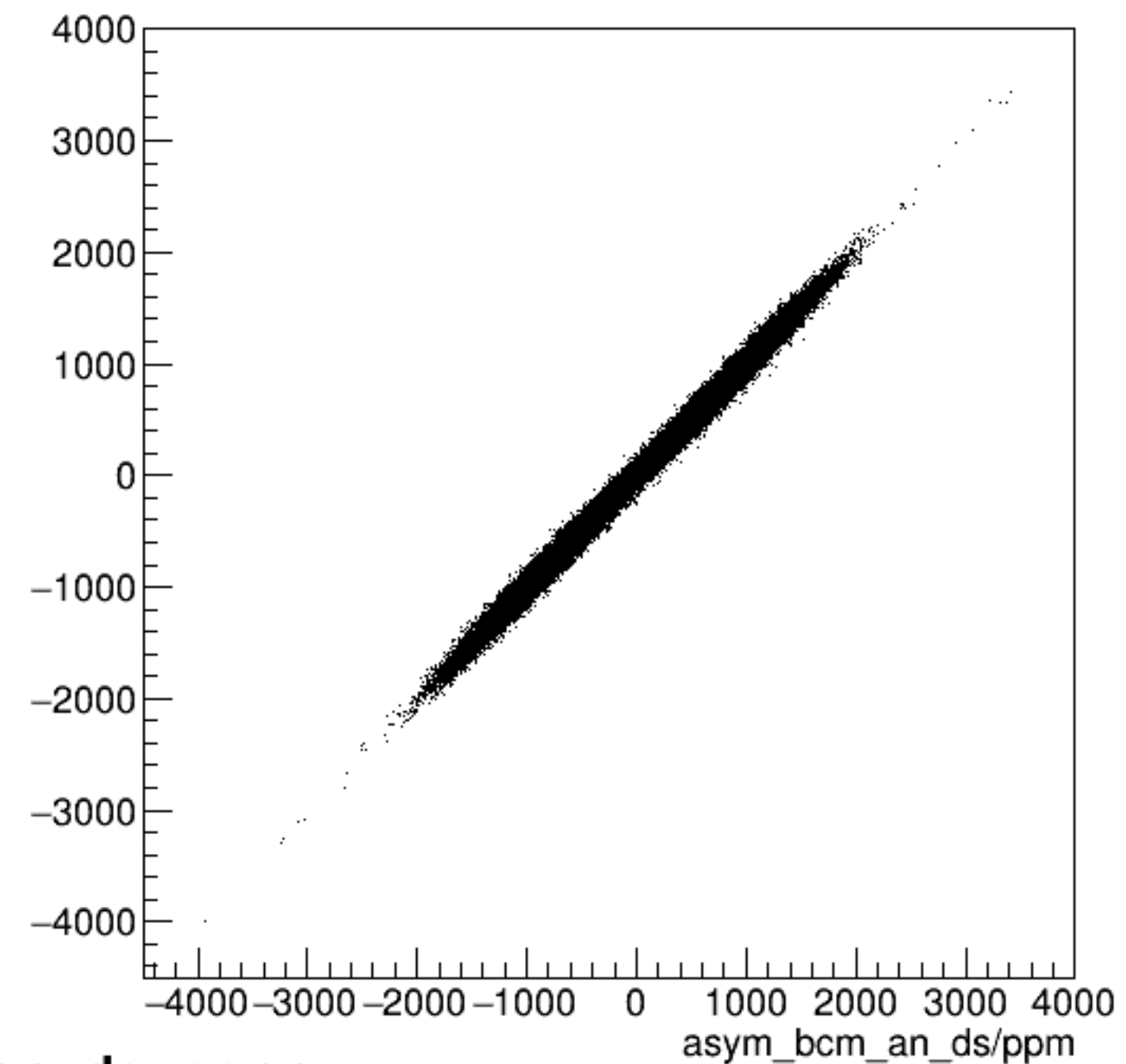
run8398_000_asym_bcm_dg_us_vs_asym_bcm_an_ds_pr.png
