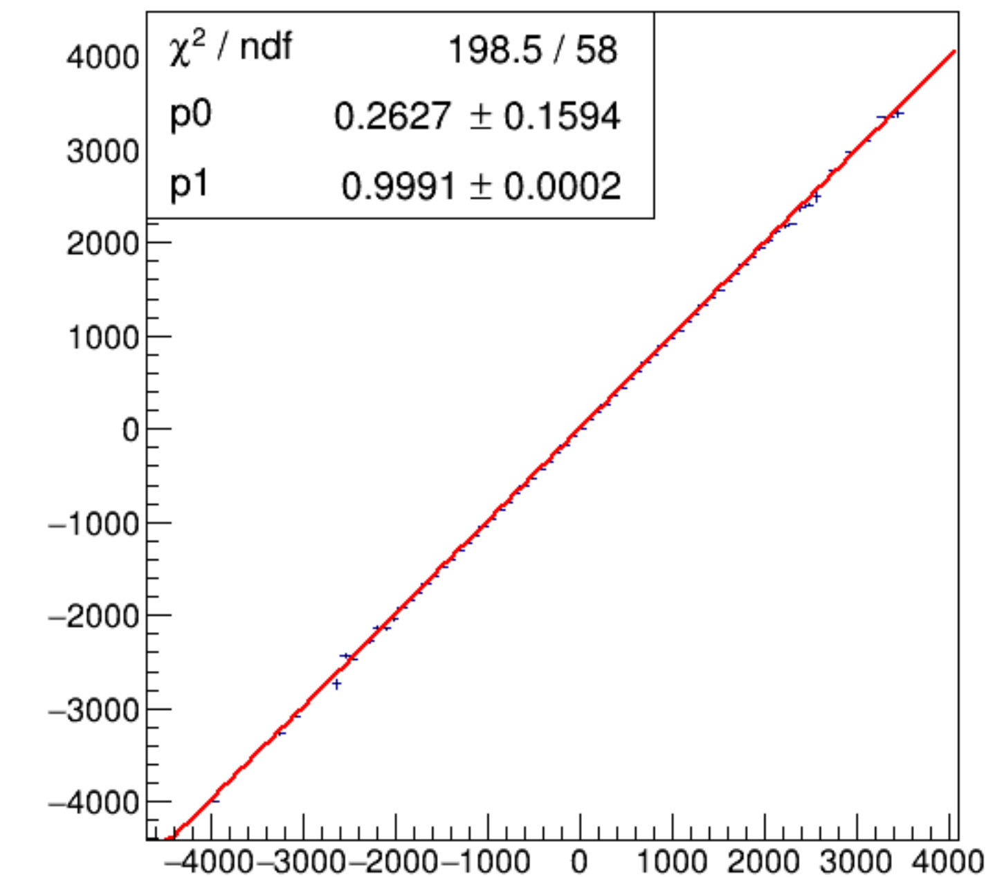
run8398_000_asym_bcm_dg_us_vs_asym_bcm_an_ds3_pr.png
