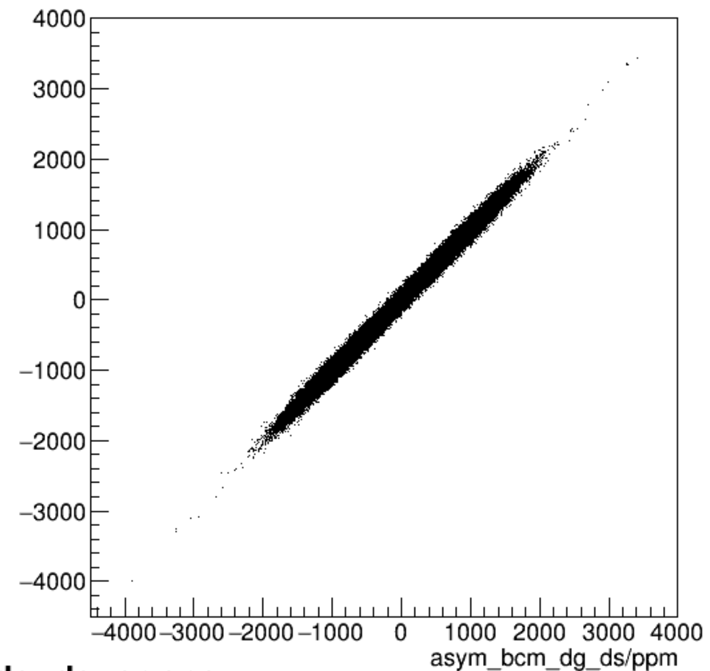
run8398_000_asym_bcm_dg_us_vs_asym_bcm_dg_ds_pr.png
