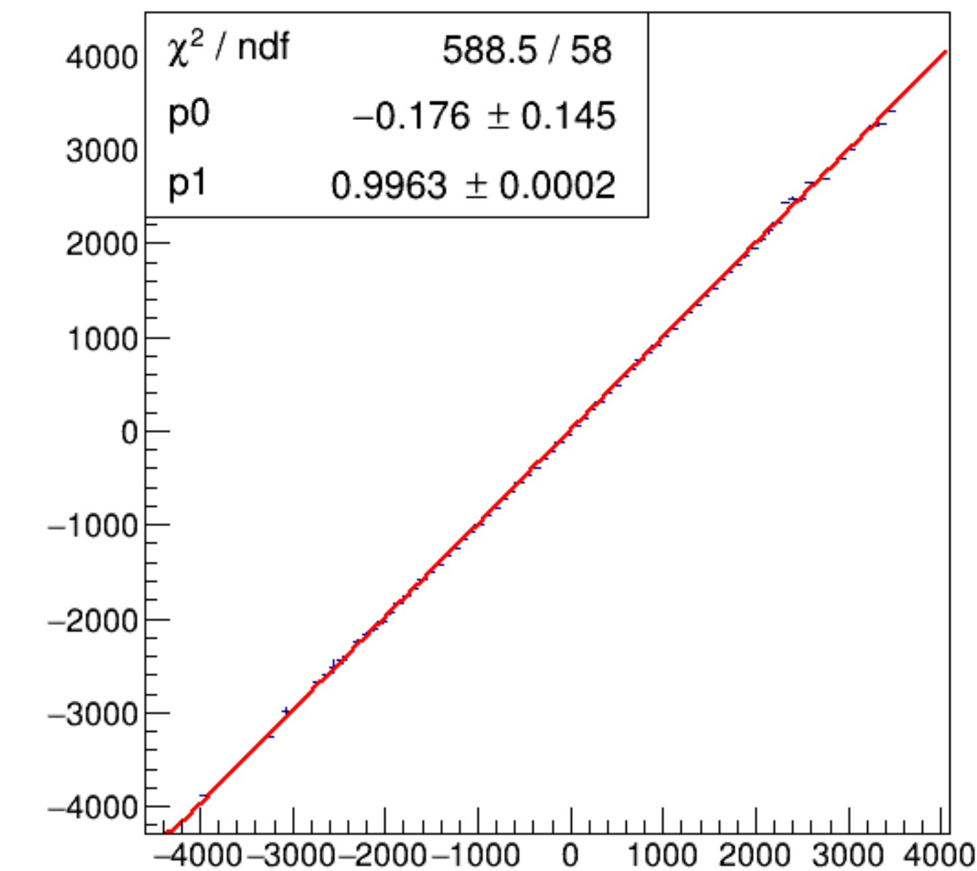
run8398_000_asym_bcm_dg_ds_vs_asym_bcm_an_us_pr.png
