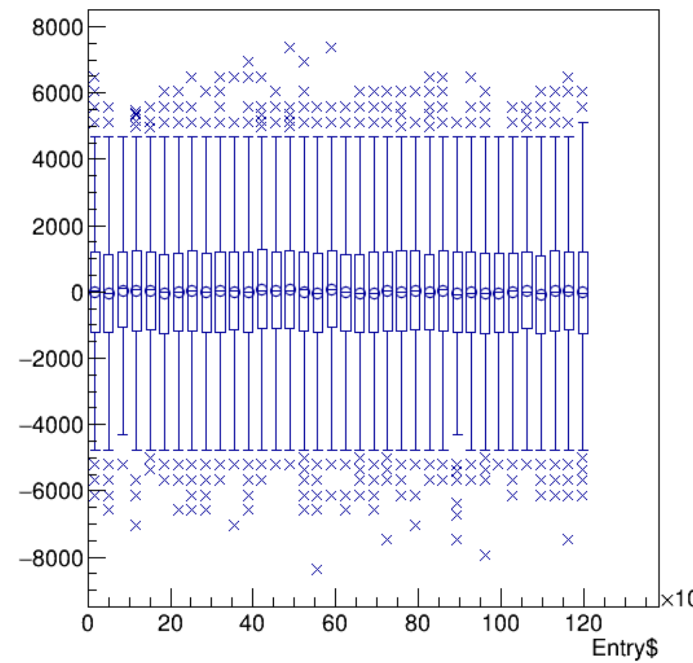
(reg_asym_atl2/ppm-reg_asym_atr2/ppm)/2:Entry$ {ok_cut}
