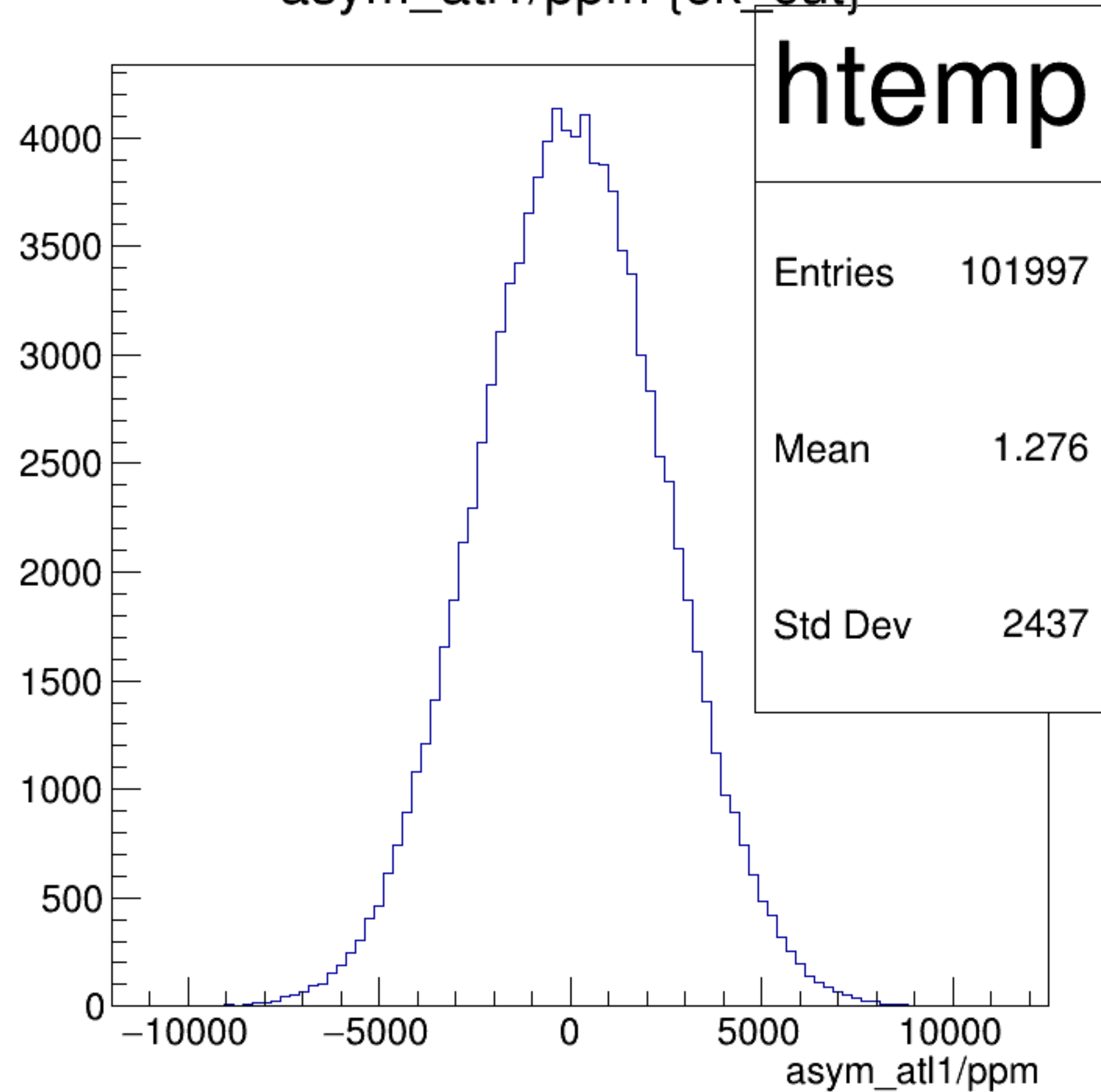
asym_atl1/ppm {ok_cut}
