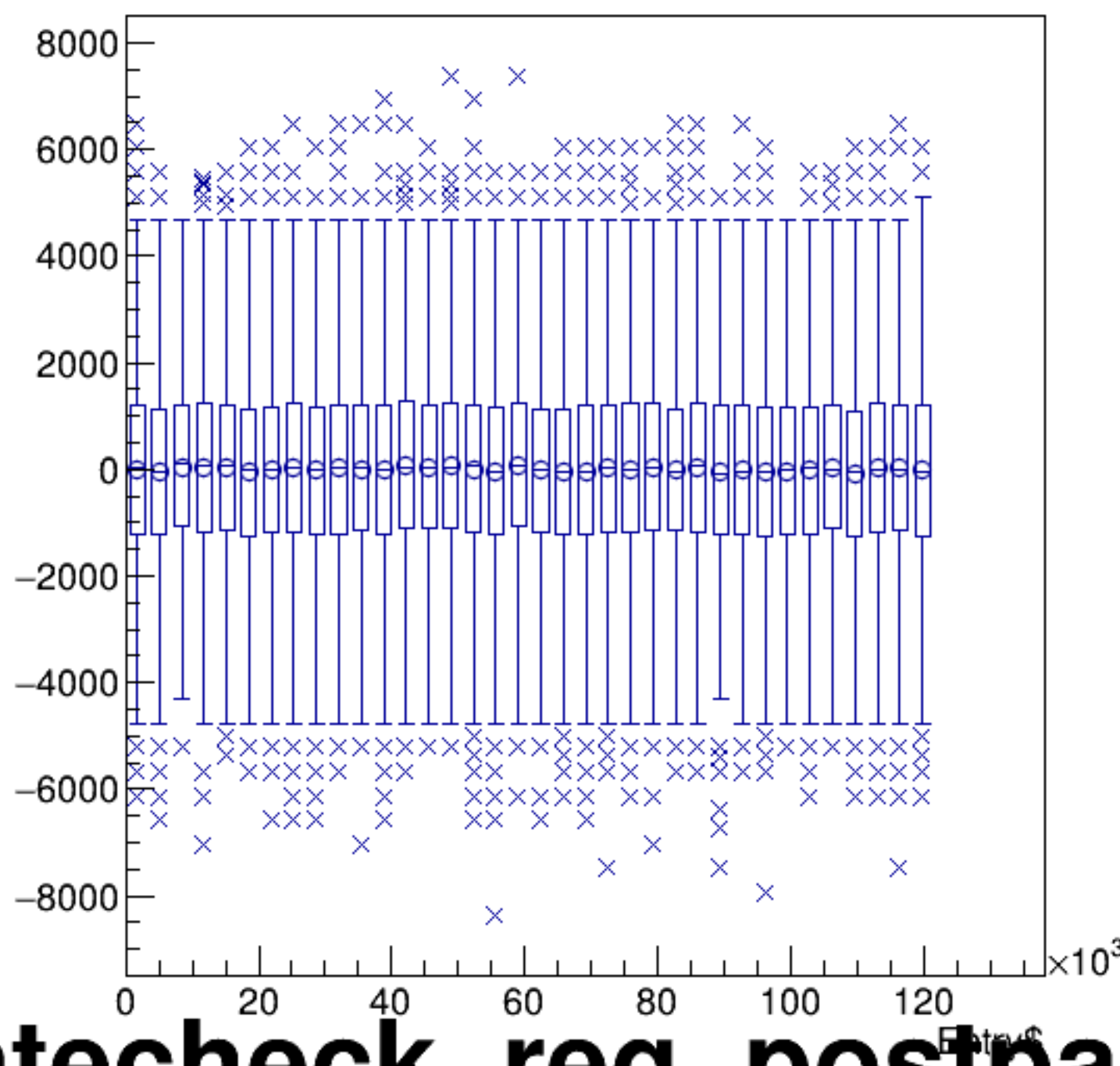
(reg_asym_atl2/ppm-reg_asym_atr2/ppm)/2:Entry$ {ok_cut}
