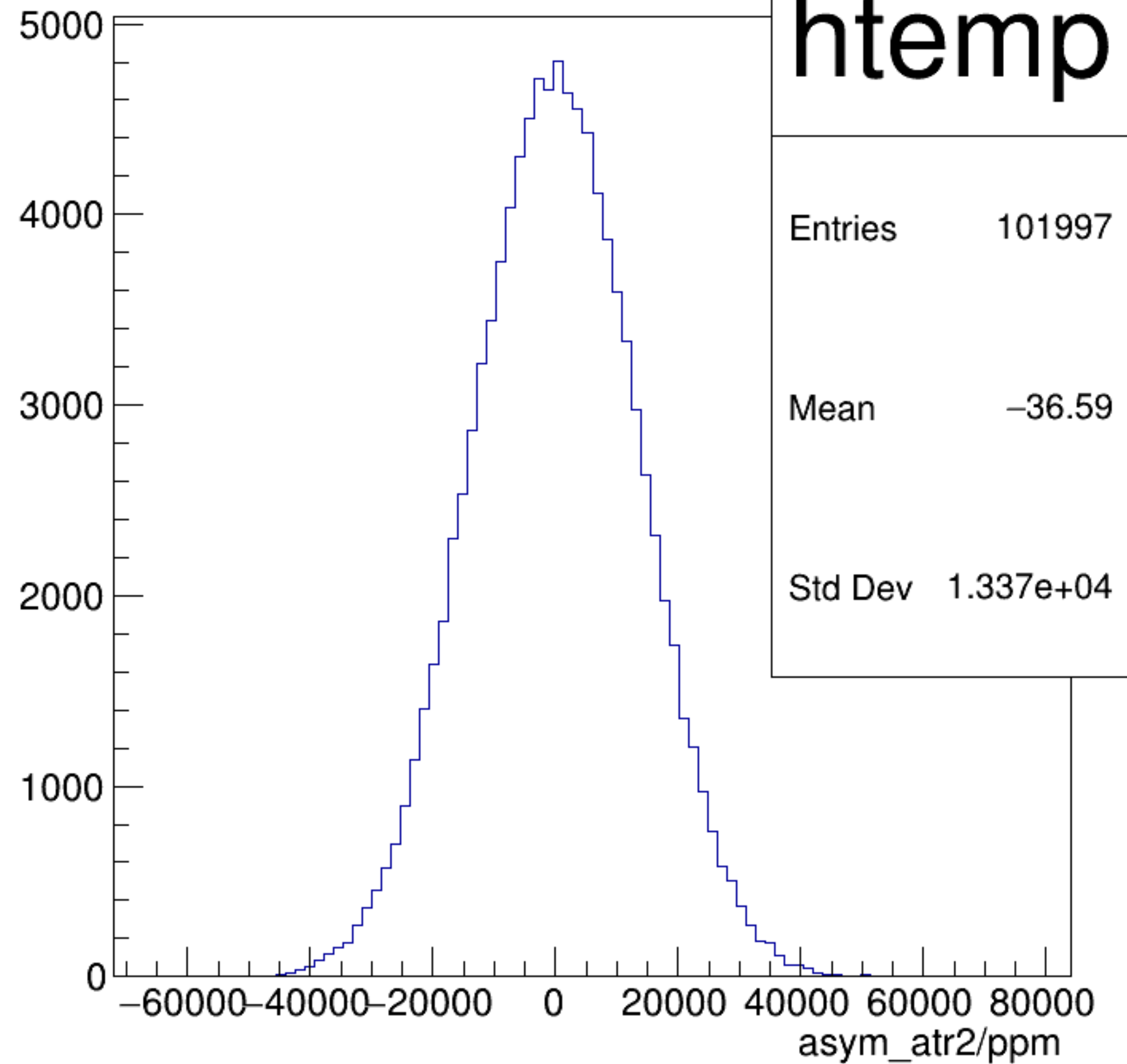
asym_atr2/ppm {ok_cut}
