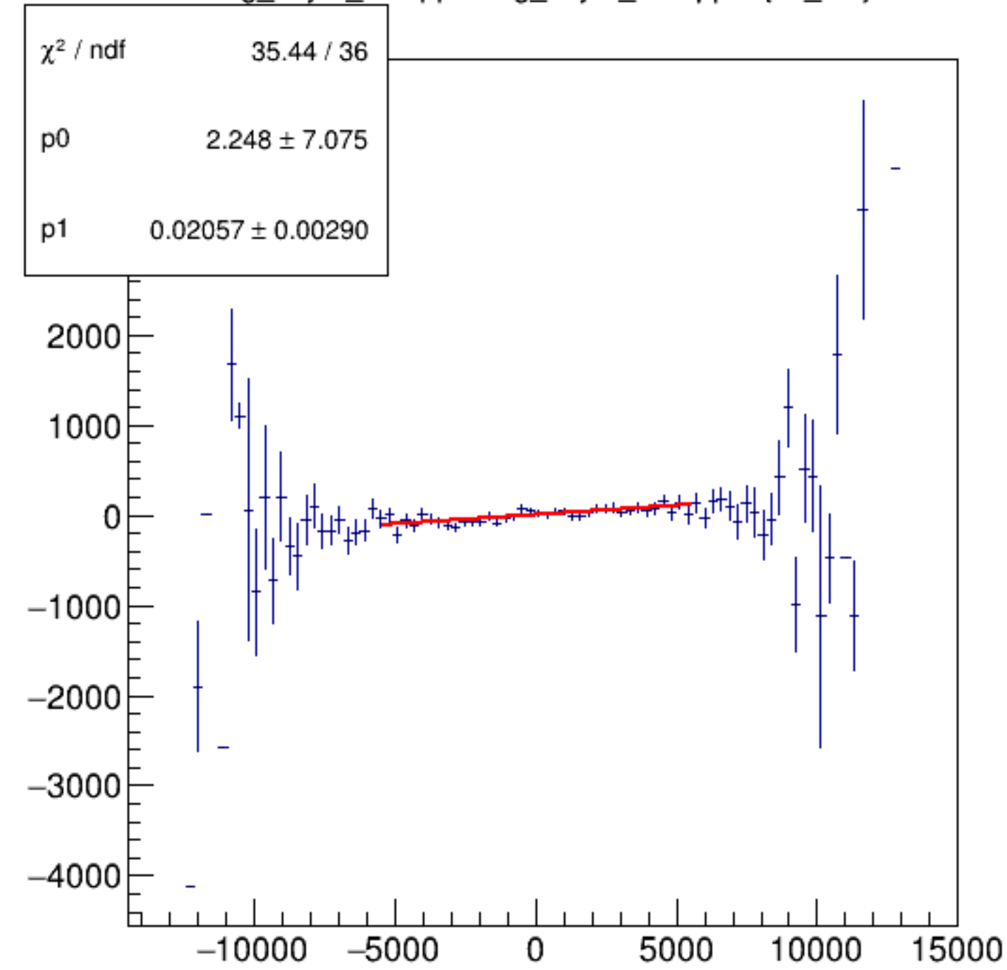
reg_asym_atl2/ppm:reg_asym_atr2/ppm {ok_cut}
