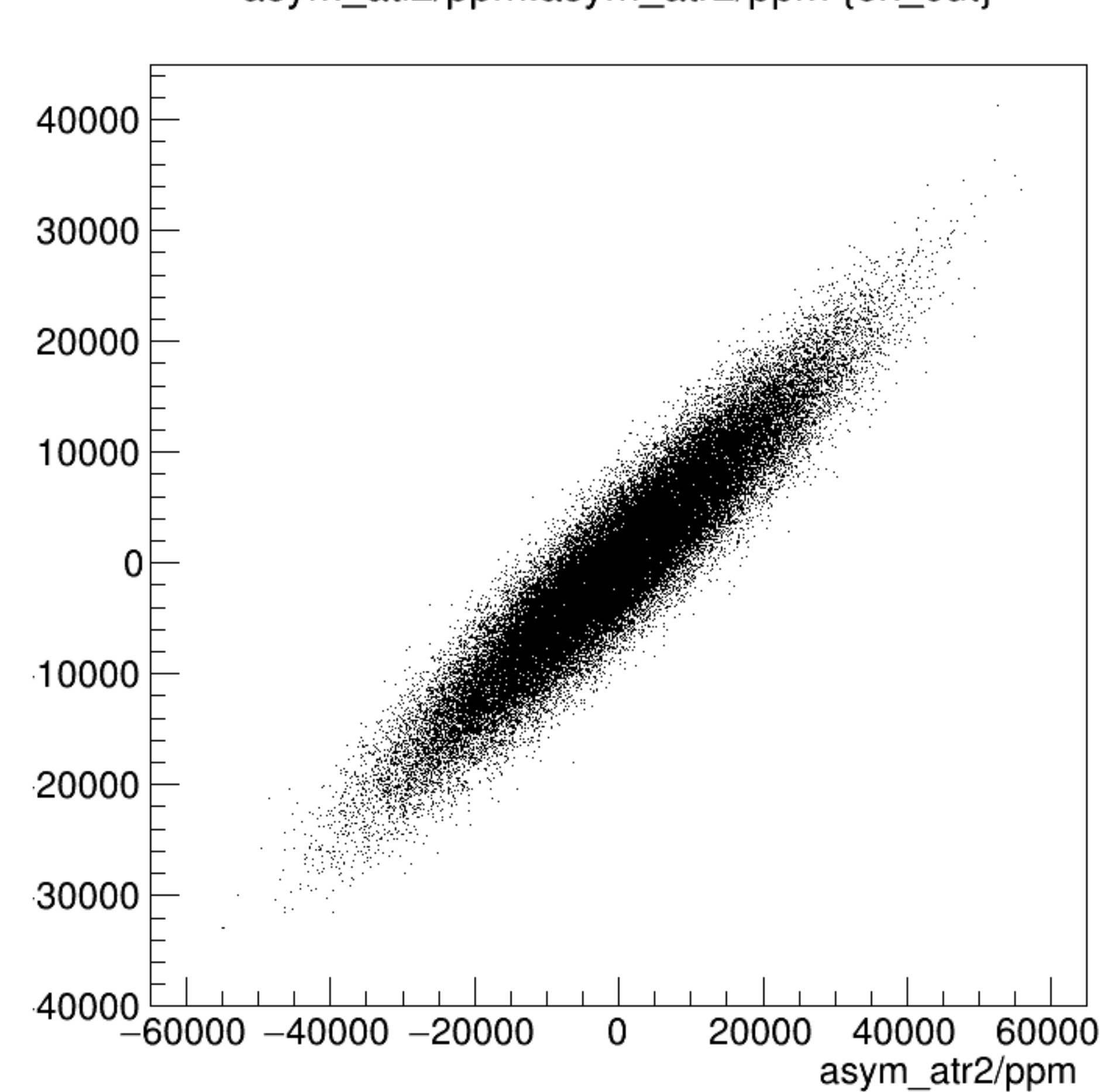
asym_atl2/ppm:asym_atr2/ppm {ok_cut}
