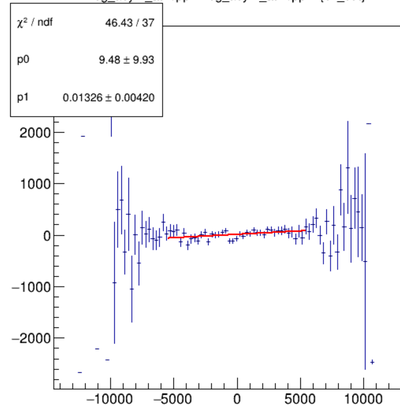
reg_asym_atl1/ppm:reg_asym_atr1/ppm {ok_cut}
