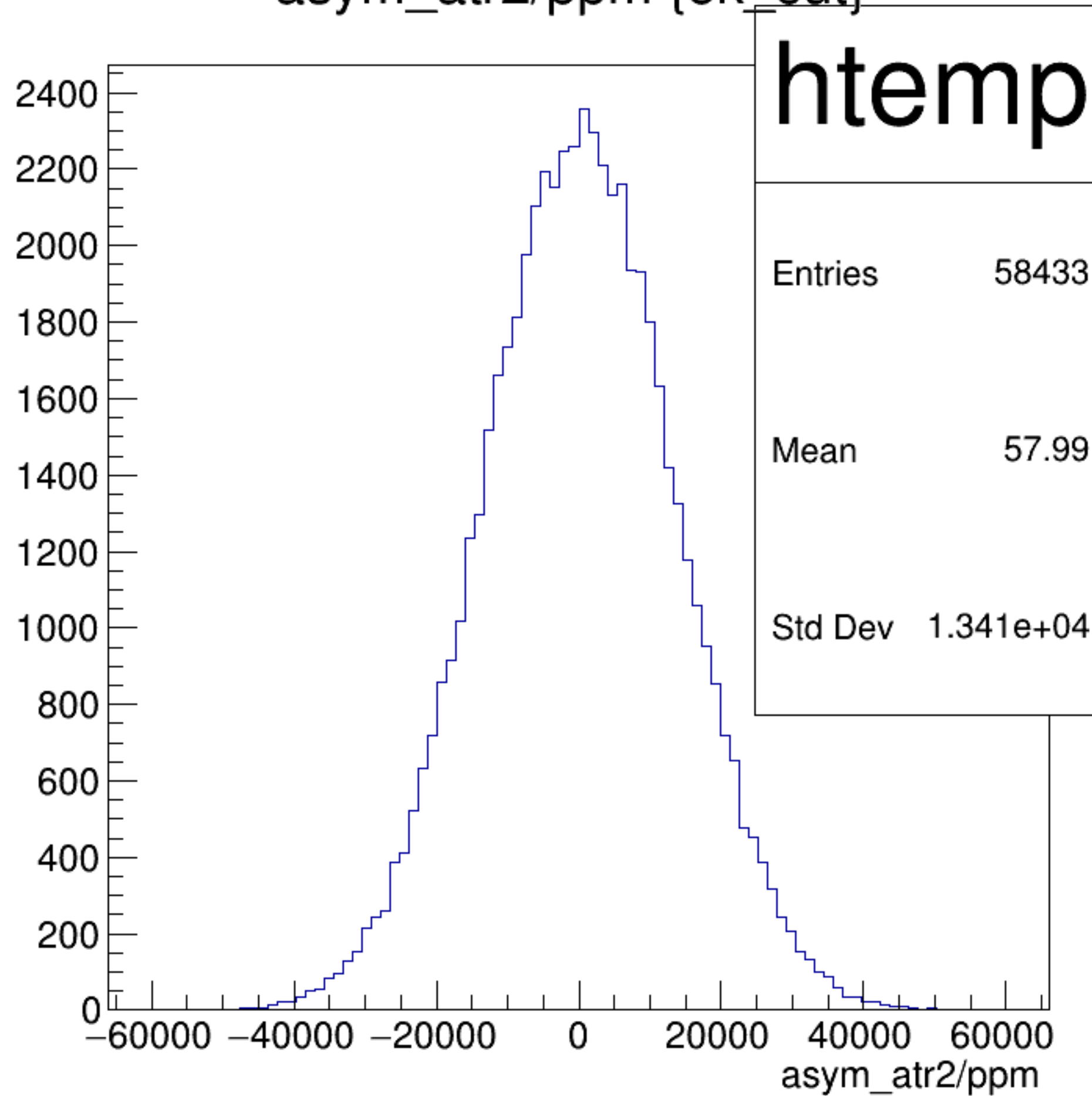
asym_atr2/ppm {ok_cut}
