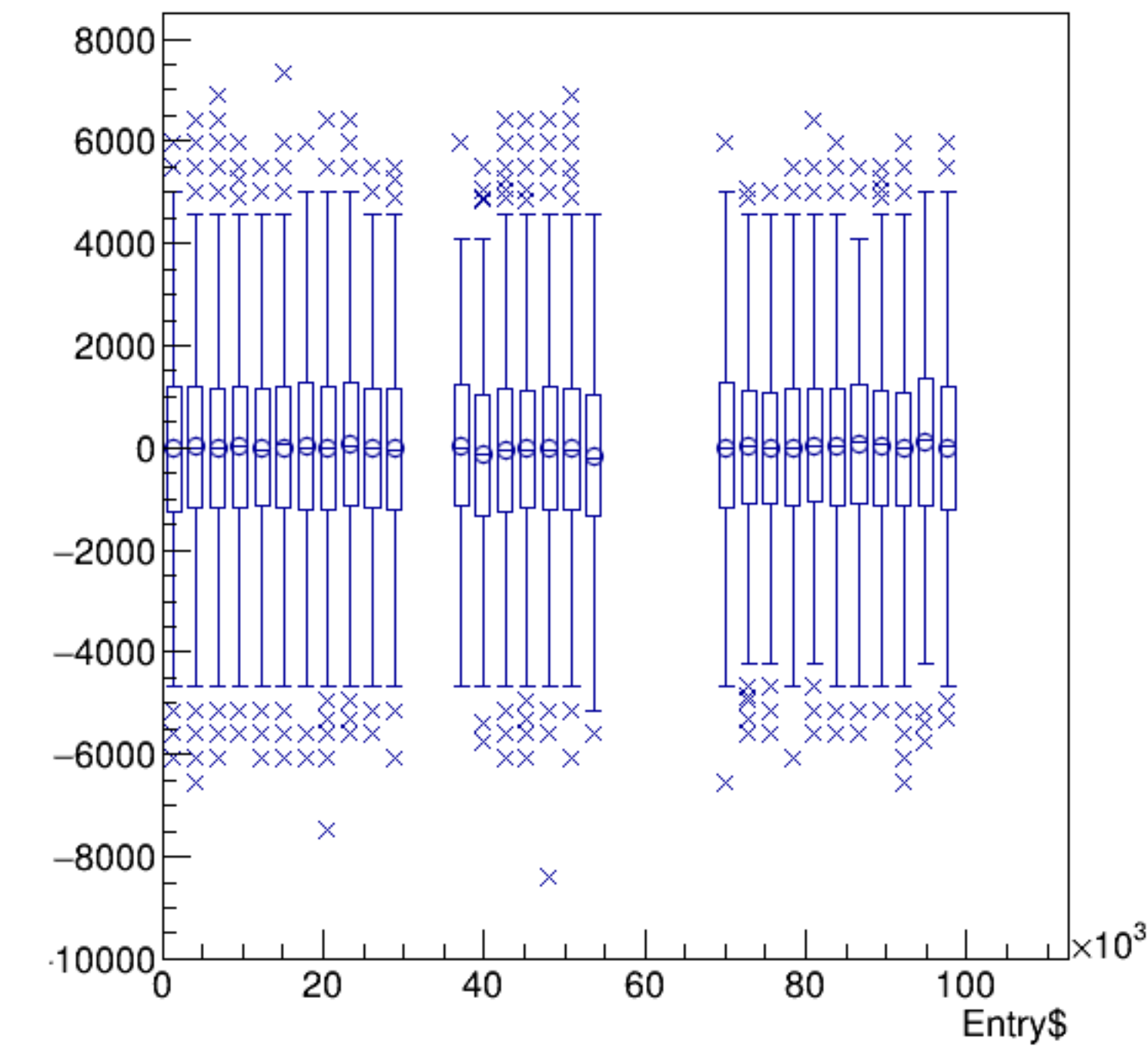
(reg_asym_atl2/ppm-reg_asym_atr2/ppm)/2:Entry$ {ok_cut}
