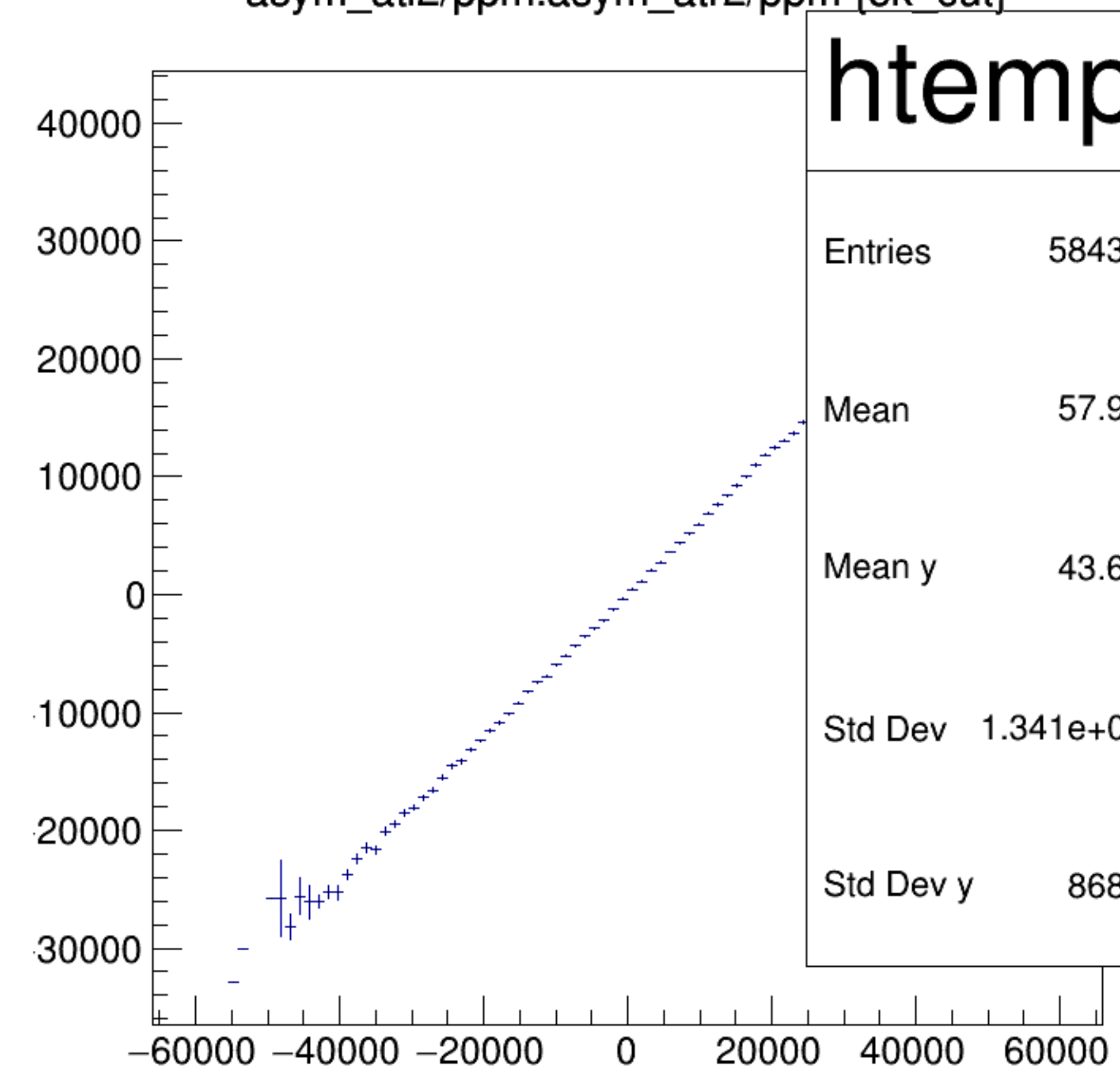
asym_atl2/ppm:asym_atr2/ppm {ok_cut}
