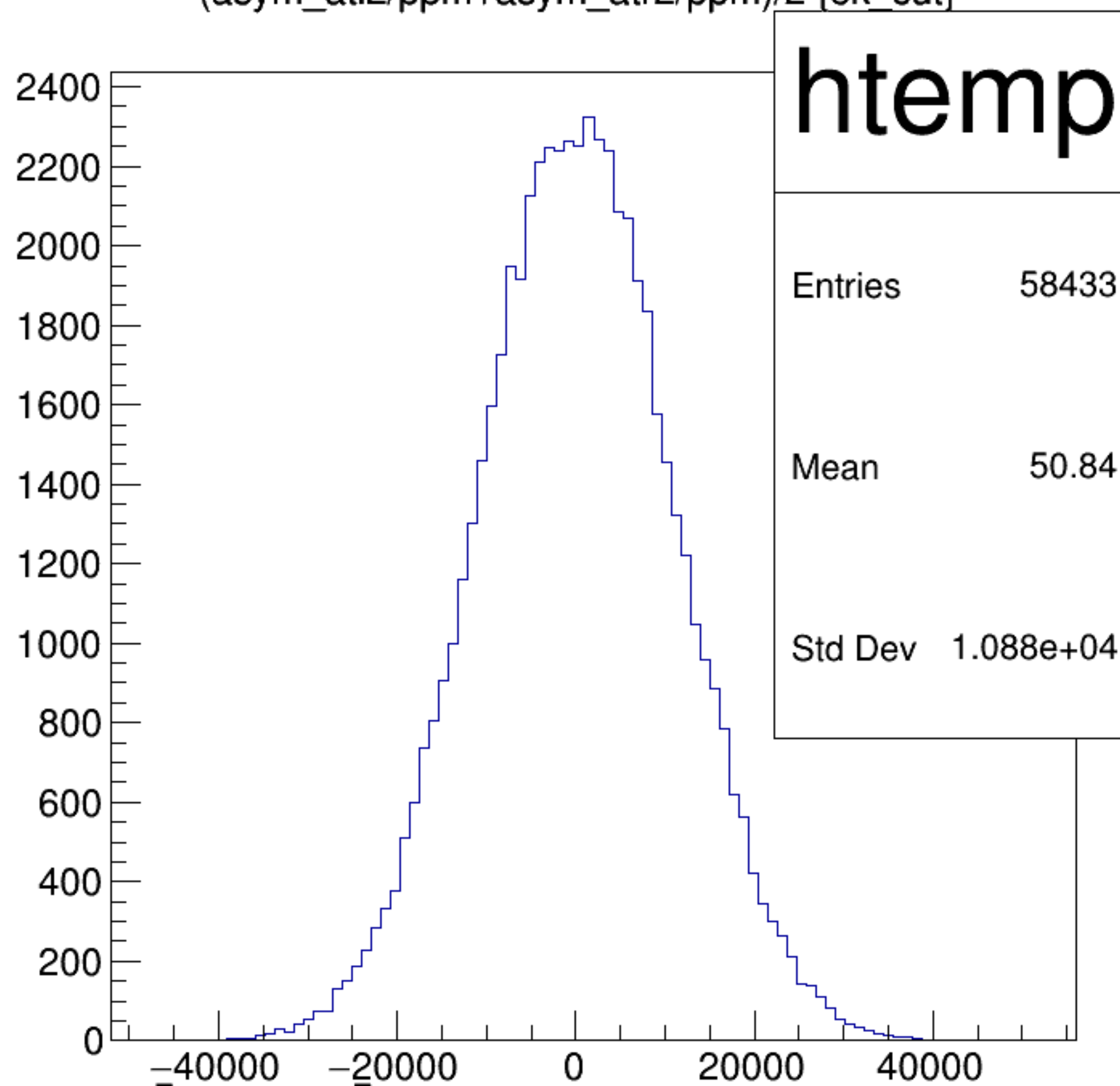
(asym_atl2/ppm+asym_atr2/ppm)/2 {ok_cut}
