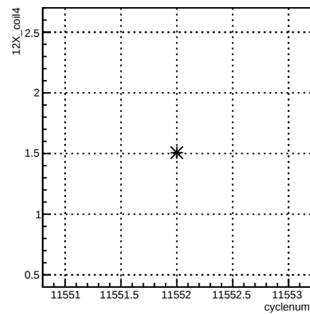
12X_coil4:cyclenum {run == 8407}
