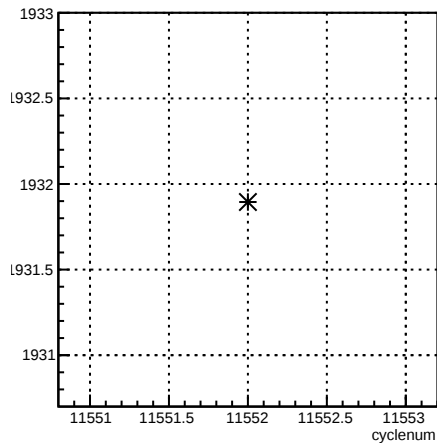
usl_coil7:cyclenum {run == 8407}
