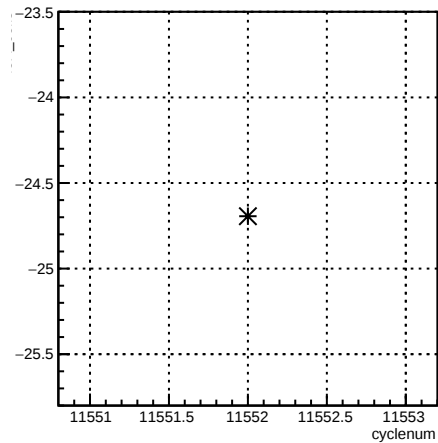
4eX_coil3:cyclenum {run == 8407}
