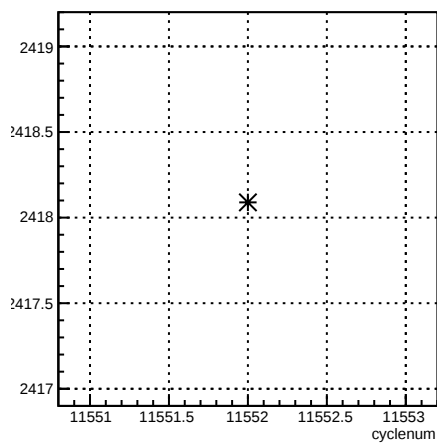
usl_coil3:cyclenum {run == 8407}
