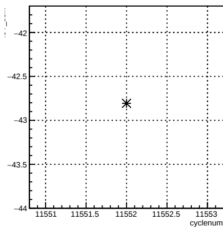
4eY_coil7:cyclenum {run == 8407}
