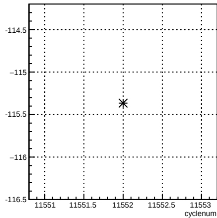
usr_4eY:cyclenum {run == 8407}
