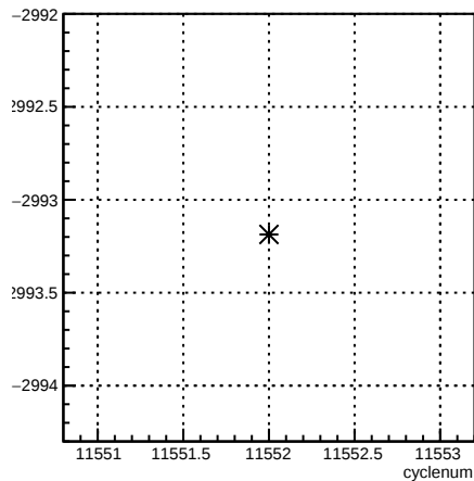
usl_coil6:cyclenum {run == 8407}
