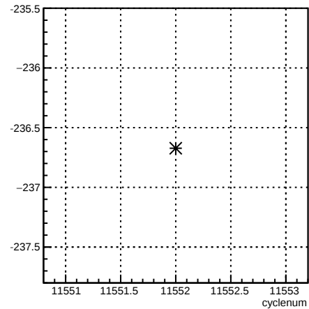
4eX_coil1:cyclenum {run == 8407}
