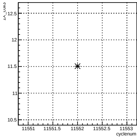
4eX_coil3:cyclenum {run == 8407}
