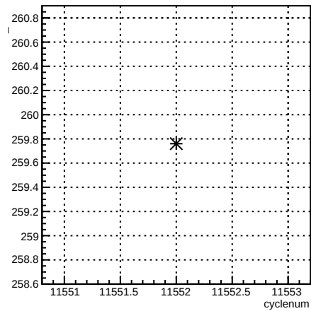
4eX_coil7:cyclenum {run == 8407}
