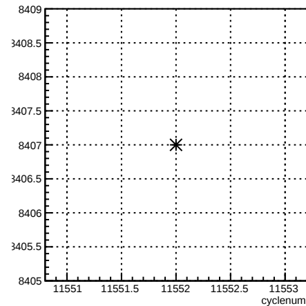
run:cyclenum {run == 8407}
