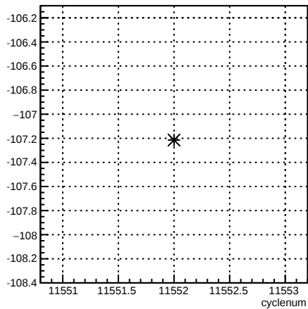
4eY_coil6:cyclenum {run == 8407}
