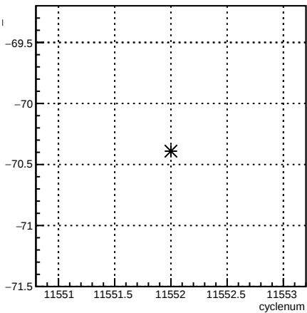
usl_4eY:cyclenum {run == 8407}
