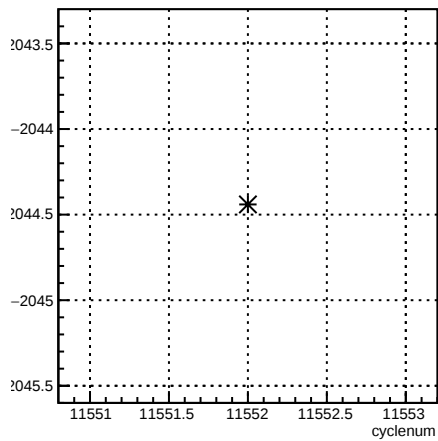
usr_coil3:cyclenum {run == 8407}
