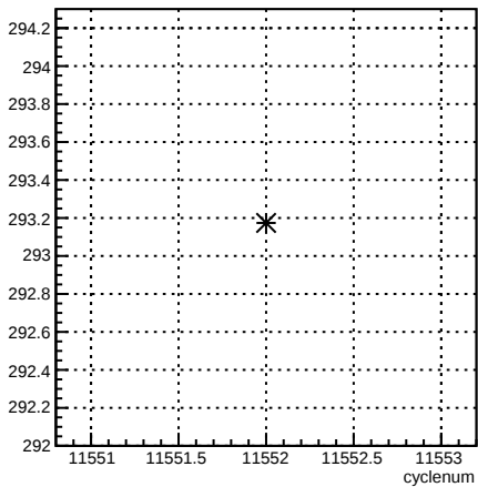
4eY_coil4:cyclenum {run == 8407}
