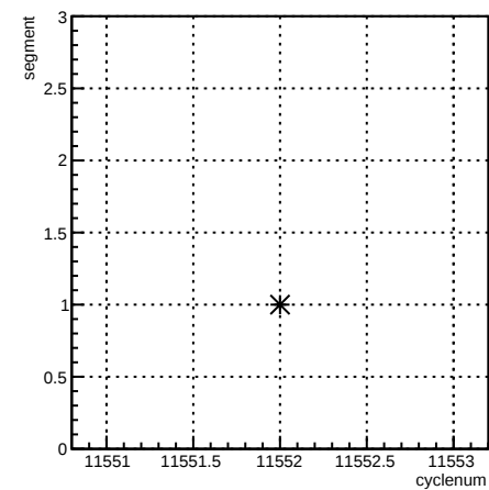
segment:cyclenum {run == 8407}
