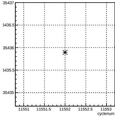
usr_coil7:cyclenum {run == 8407}
