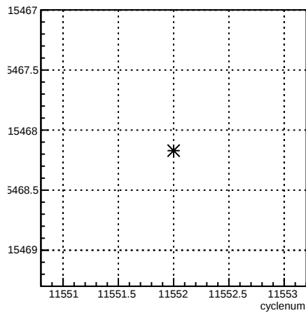
usr_coil1:cyclenum {run == 8407}
