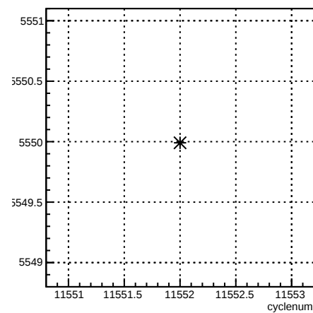
usl_coil4:cyclenum {run == 8407}
