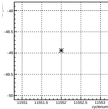
4eY_coil7:cyclenum {run == 8407}
