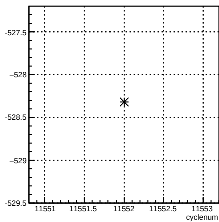
12X_coil7:cyclenum {run == 8407}
