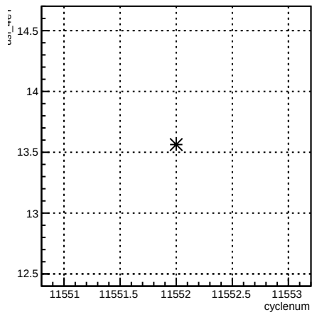
usl_4eY:cyclenum {run == 8407}
