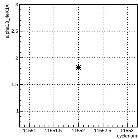
alpha13_4eX1X:cyclenum {run == 8407}
