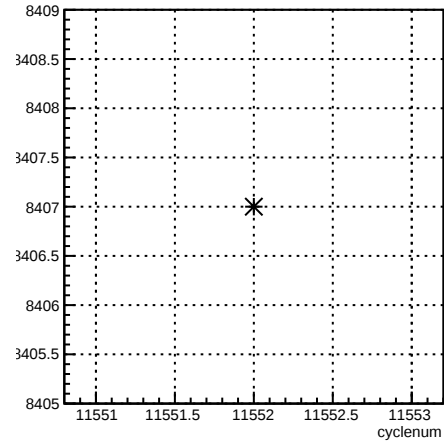
run:cyclenum {run == 8407}
