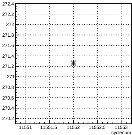
4eY_coil4:cyclenum {run == 8407}
