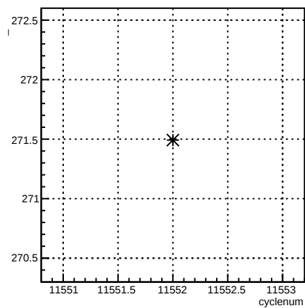
4eX_coil7:cyclenum {run == 8407}
