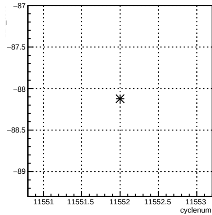
12X_coil3:cyclenum {run == 8407}
