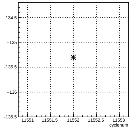
4eX_coil1:cyclenum {run == 8407}
