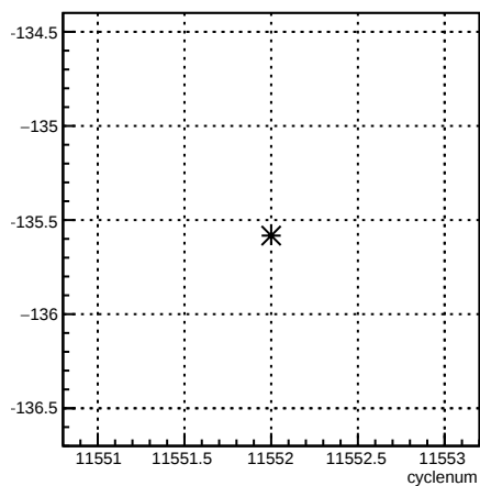
4eY_coil6:cyclenum {run == 8407}
