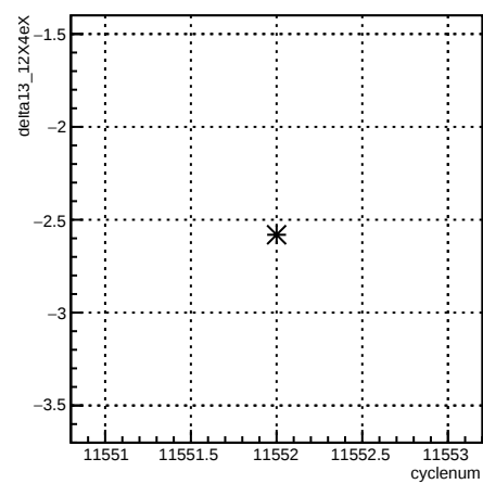
delta13_12X4eX:cyclenum {run == 8407}
