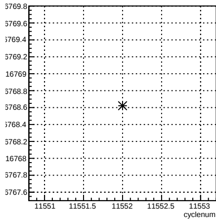
usl_coil1:cyclenum {run == 8407}
