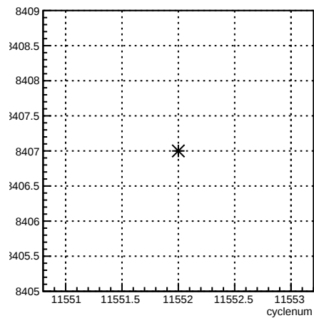
run:cyclenum {run == 8407}
