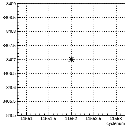
run:cyclenum {run == 8407}
