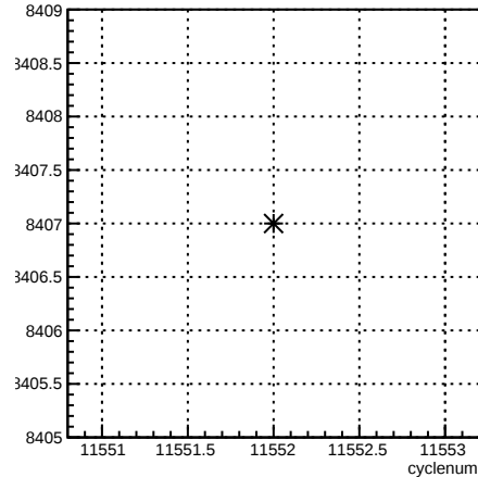
run:cyclenum {run == 8407}
