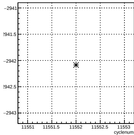
usr_coil6:cyclenum {run == 8407}
