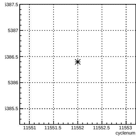
usr_coil4:cyclenum {run == 8407}
