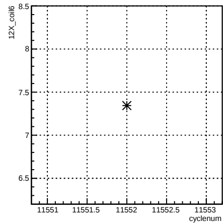
12X_coil6:cyclenum {run == 8407}
