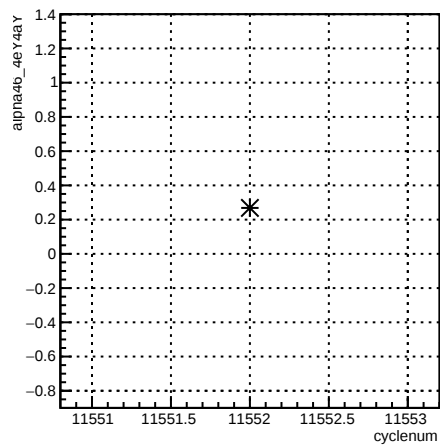
alpha46_4eY4aY:cyclenum {run == 8407}
