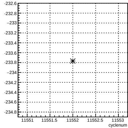
12X_coil1:cyclenum {run == 8407}
