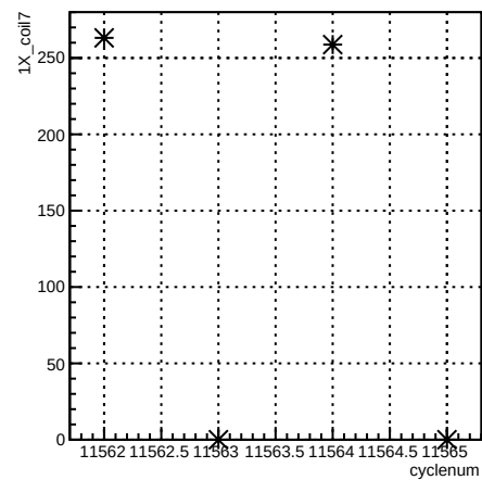
1X_coil7:cyclenum {run == 8409}
