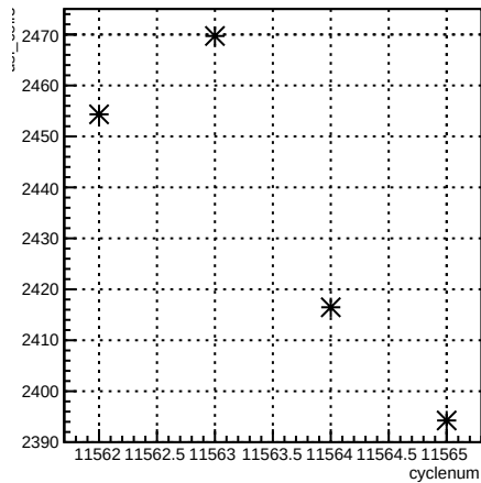
usl_coil7:cyclenum {run == 8409}
