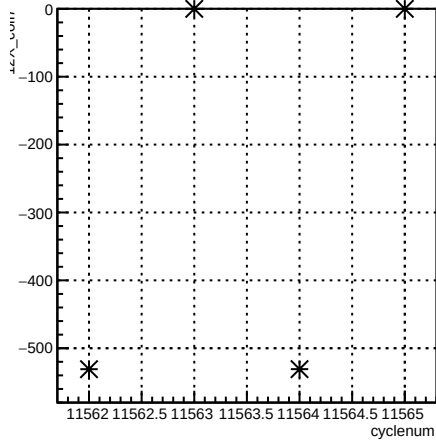
12X_coil7:cyclenum {run == 8409}
