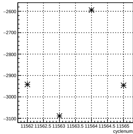
usr_coil6:cyclenum {run == 8409}
