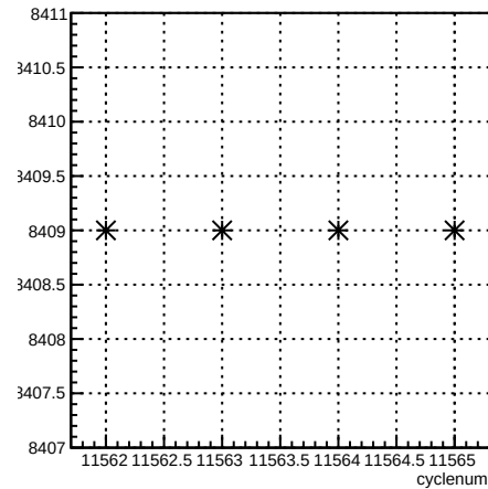
run:cyclenum {run == 8409}
