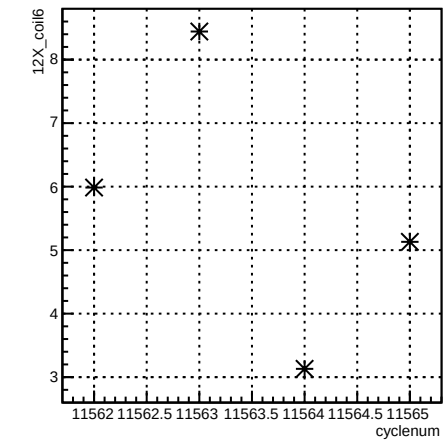
12X_coil6:cyclenum {run == 8409}
