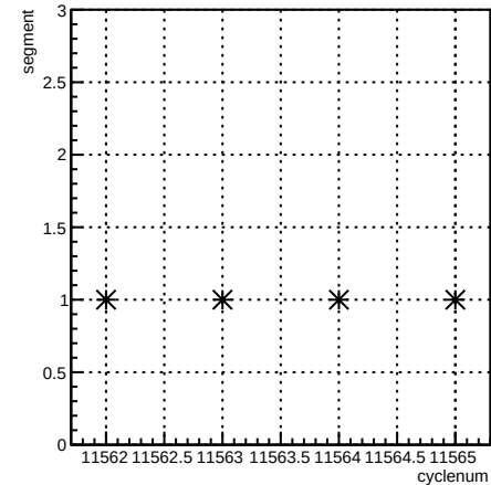
segment:cyclenum {run == 8409}
