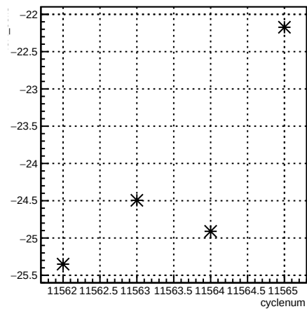
4eX_coil3:cyclenum {run == 8409}
