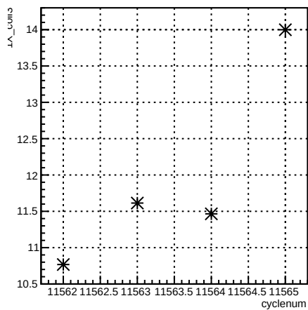
1X_coil3:cyclenum {run == 8409}
