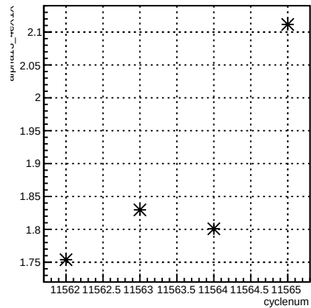
alpha13_4eX1X:cyclenum {run == 8409}
