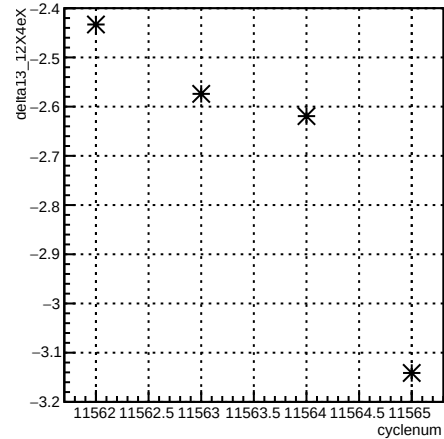
delta13_12X4eX:cyclenum {run == 8409}
