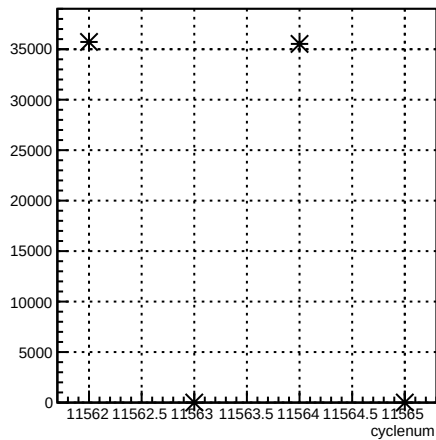
usr_coil7:cyclenum {run == 8409}
