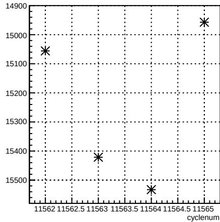
usr_coil1:cyclenum {run == 8409}
