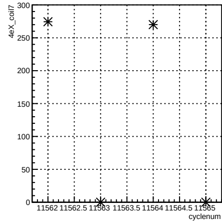
4eX_coil7:cyclenum {run == 8409}
