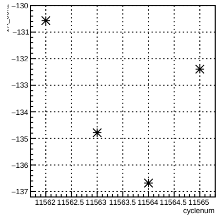
1X_coil1:cyclenum {run == 8409}
