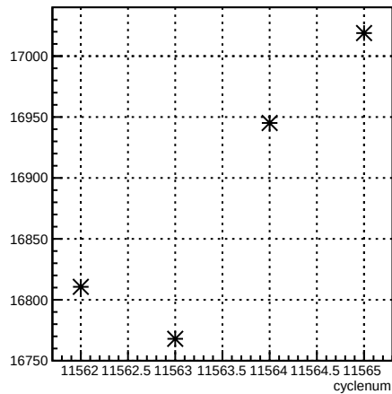
usl_coil6:cyclenum {run == 8409}
