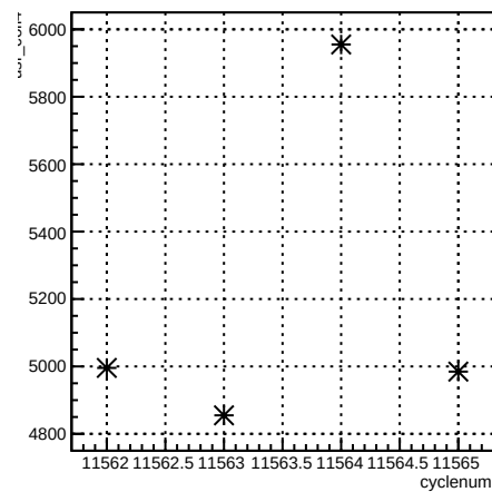
usr_coil4:cyclenum {run == 8409}
