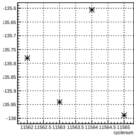
4eY_coil6:cyclenum {run == 8409}
