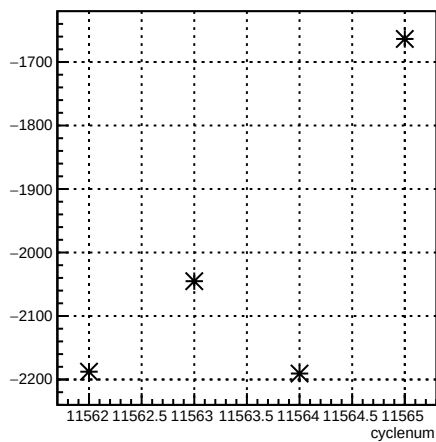
usr_coil3:cyclenum {run == 8409}
