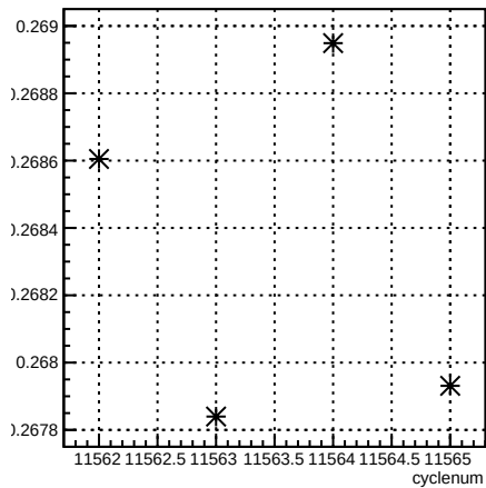
alpha46_4eY4aY:cyclenum {run == 8409}
