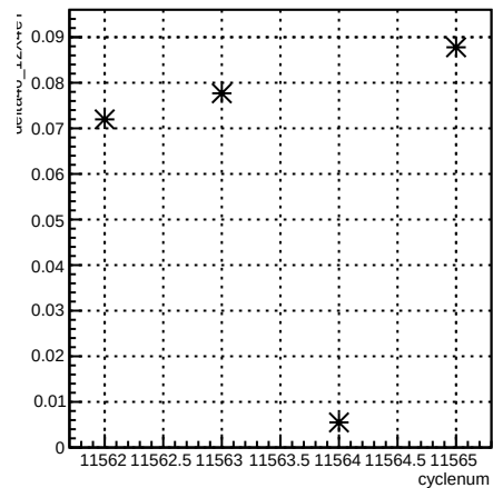
delta46_12X4eY:cyclenum {run == 8409}
