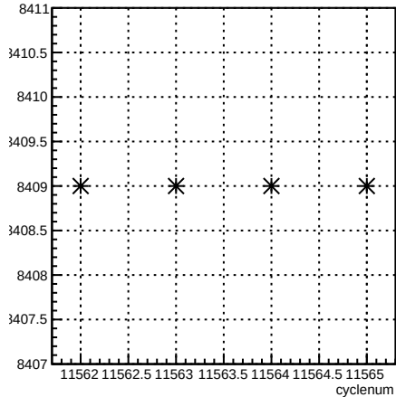
run:cyclenum {run == 8409}
