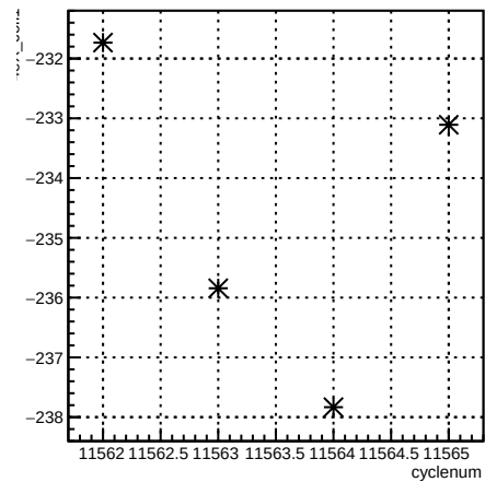
4eX_coil1:cyclenum {run == 8409}
