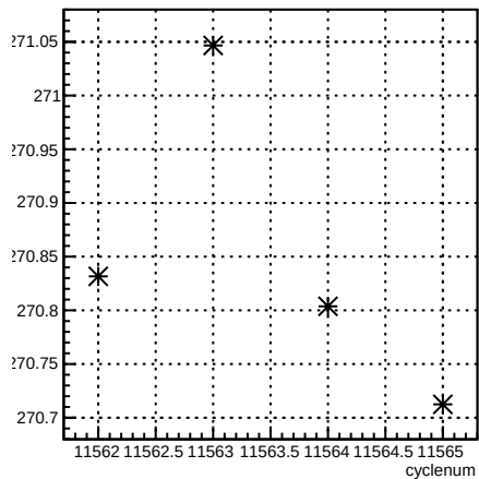
4eY_coil4:cyclenum {run == 8409}
