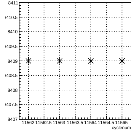
run:cyclenum {run == 8409}
