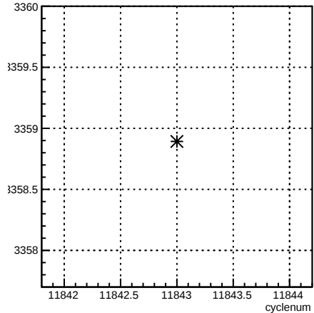
usl_coil7:cyclenum {run == 8531}
