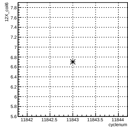
12X_coil6:cyclenum {run == 8531}
