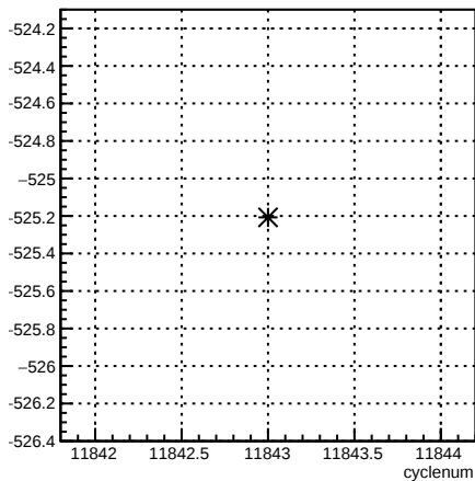
12X_coil7:cyclenum {run == 8531}
