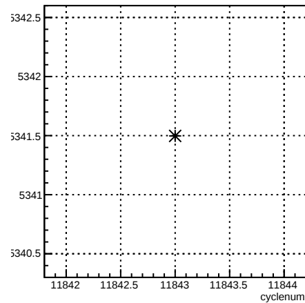
usr_coil4:cyclenum {run == 8531}
