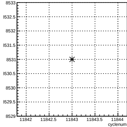
run:cyclenum {run == 8531}
