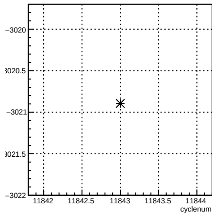
usr_coil6:cyclenum {run == 8531}
