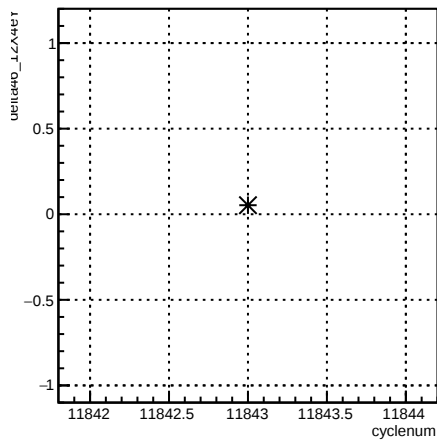
delta46_12X4eY:cyclenum {run == 8531}
