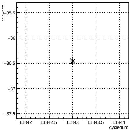
4eY_coil7:cyclenum {run == 8531}
