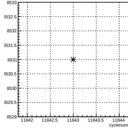
run:cyclenum {run == 8531}
