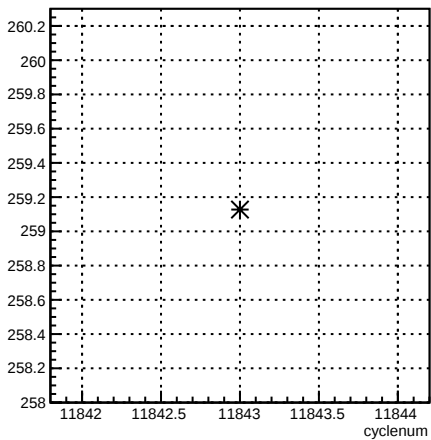
4eY_coil4:cyclenum {run == 8531}
