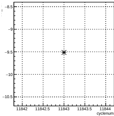
usl_12X:cyclenum {run == 8531}
