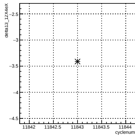
delta13_12X4eX:cyclenum {run == 8531}
