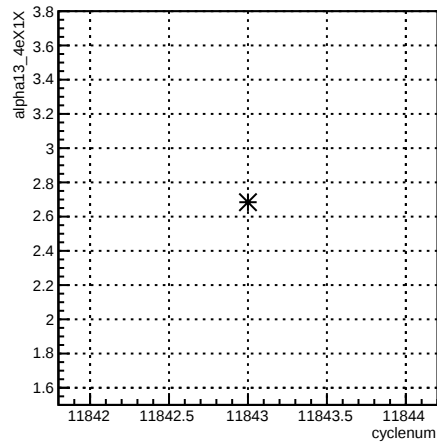
alpha13_4eX1X:cyclenum {run == 8531}
