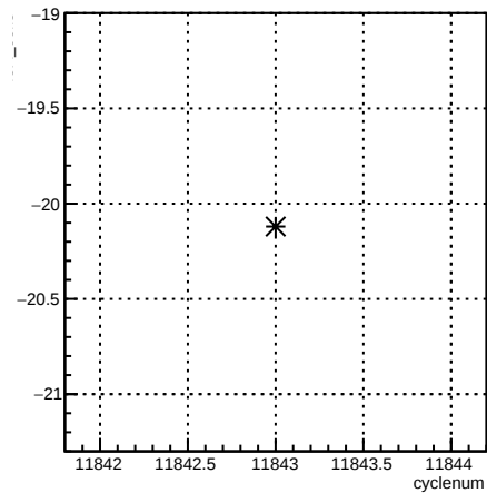
4eX_coil3:cyclenum {run == 8531}
