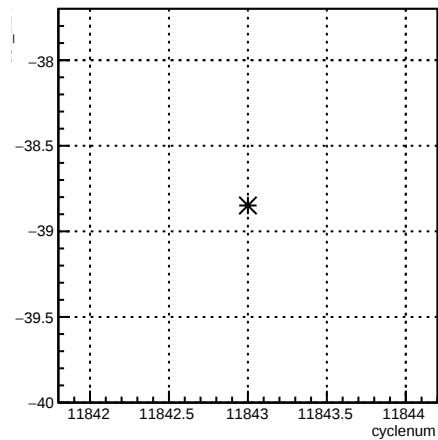
usr_12X:cyclenum {run == 8531}
