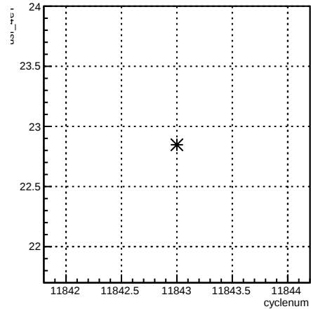
usr_4eY:cyclenum {run == 8531}
