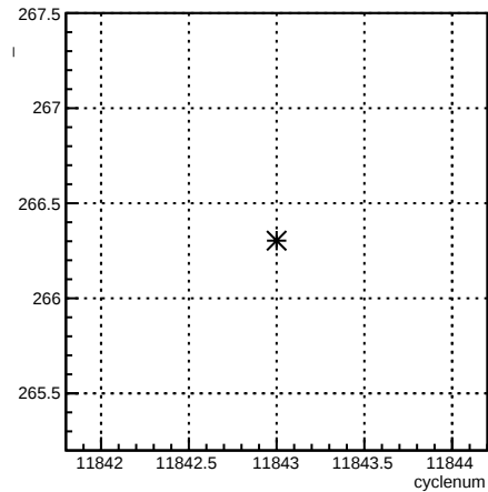
4eX_coil7:cyclenum {run == 8531}
