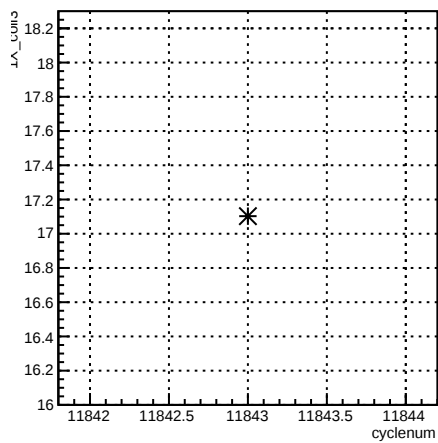
1X_coil3:cyclenum {run == 8531}
