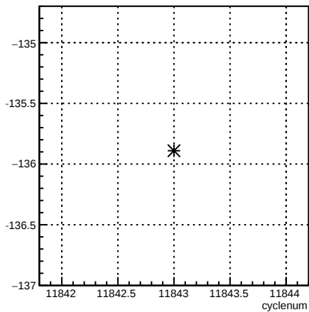
4eY_coil6:cyclenum {run == 8531}
