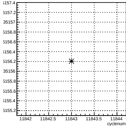
usr_coil7:cyclenum {run == 8531}
