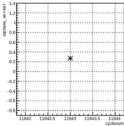
alpha46_4eY4aY:cyclenum {run == 8531}
