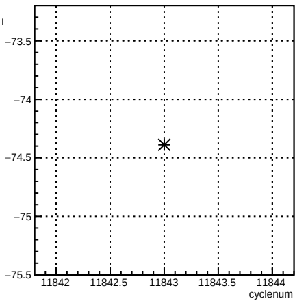
usl_4eY:cyclenum {run == 8531}
