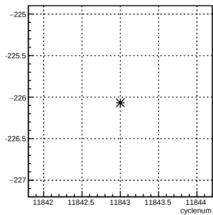
4eX_coil1:cyclenum {run == 8531}
