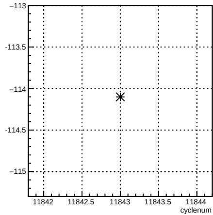
1X_coil1:cyclenum {run == 8531}
