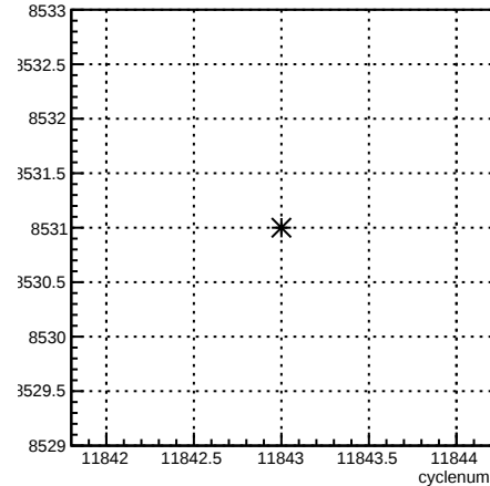
run:cyclenum {run == 8531}
