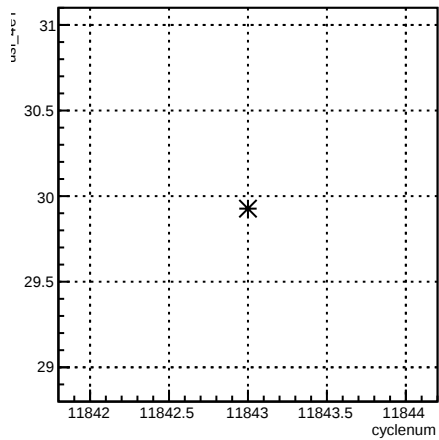
usl_4eY:cyclenum {run == 8531}
