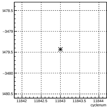
usl_coil6:cyclenum {run == 8531}
