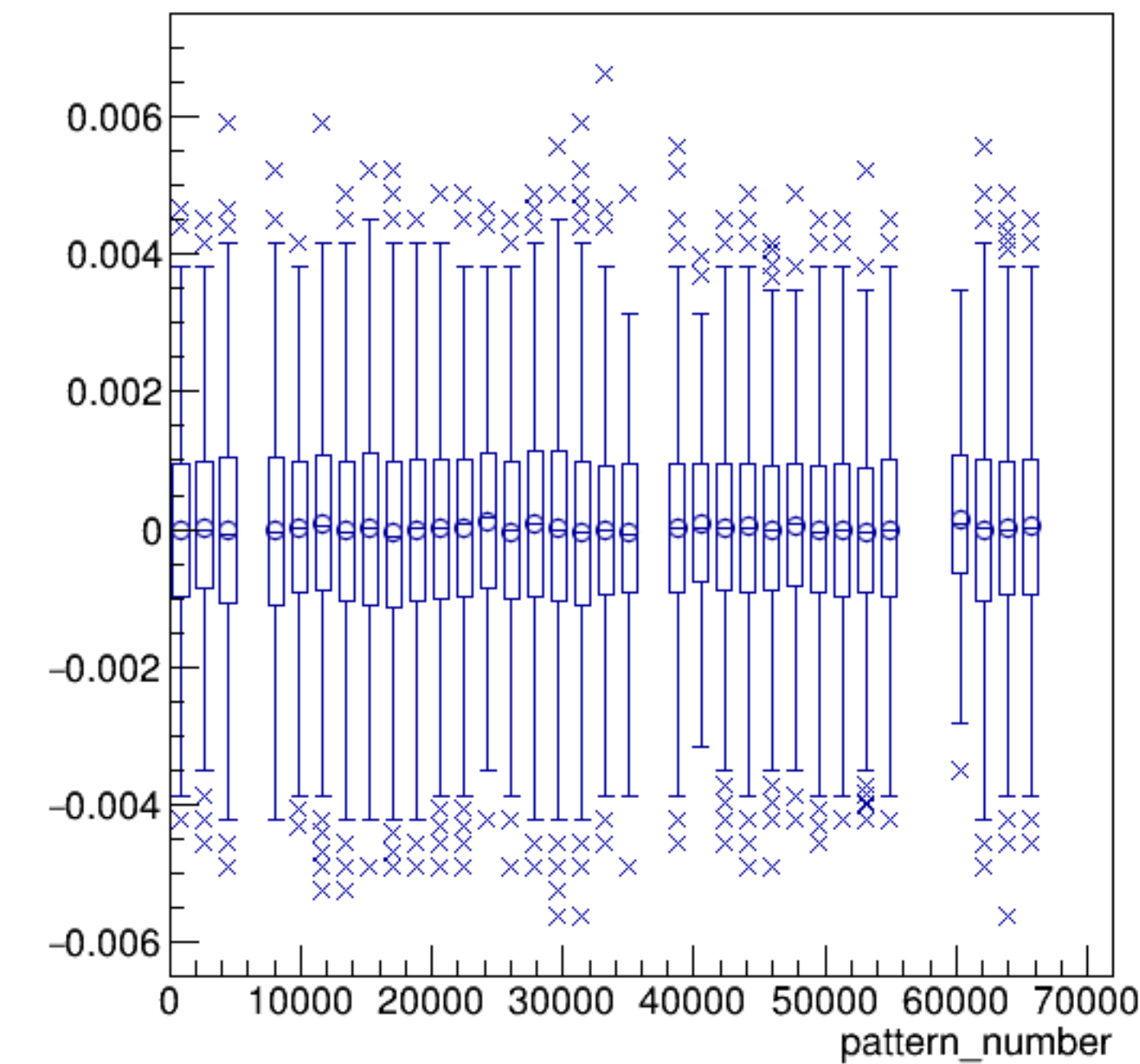
asym_bcm_an_diff*yield_bcm_an_diff:pattern_number {ErrorFlag==0}
