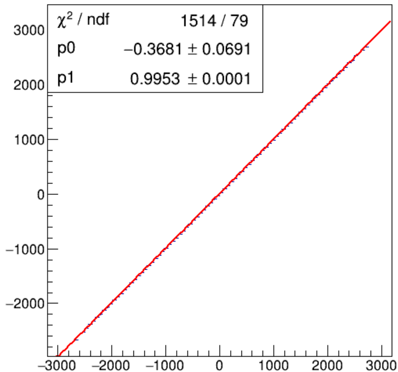
run8531_000_asym_bcm_an_ds_vs_asym_bcm_an_ds3_pr.png
