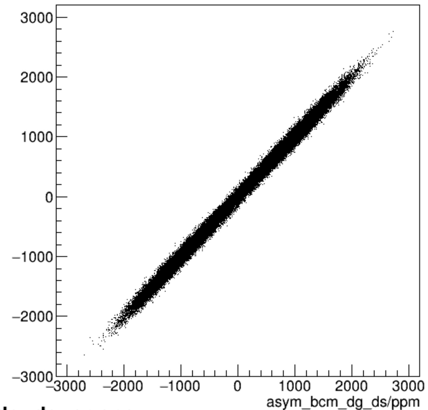
run8531_000_asym_bcm_dg_us_vs_asym_bcm_dg_ds_pr.png
