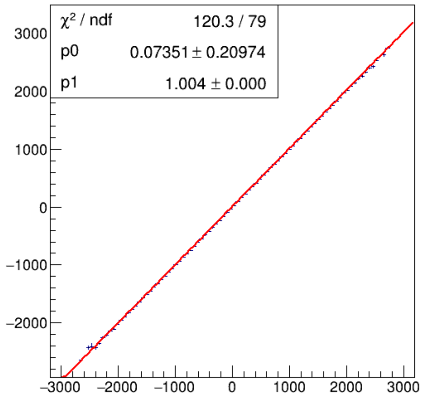
run8531_000_asym_bcm_dg_us_vs_asym_bcm_an_ds_pr.png
