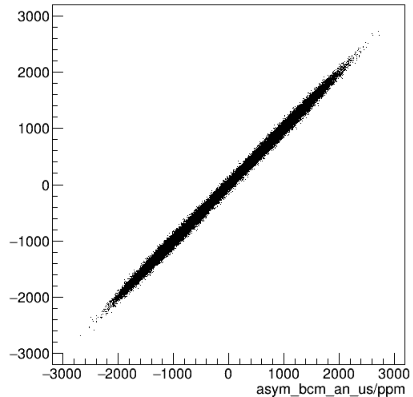
run8531_000_asym_bcm_dg_ds_vs_asym_bcm_an_us_pr.png
