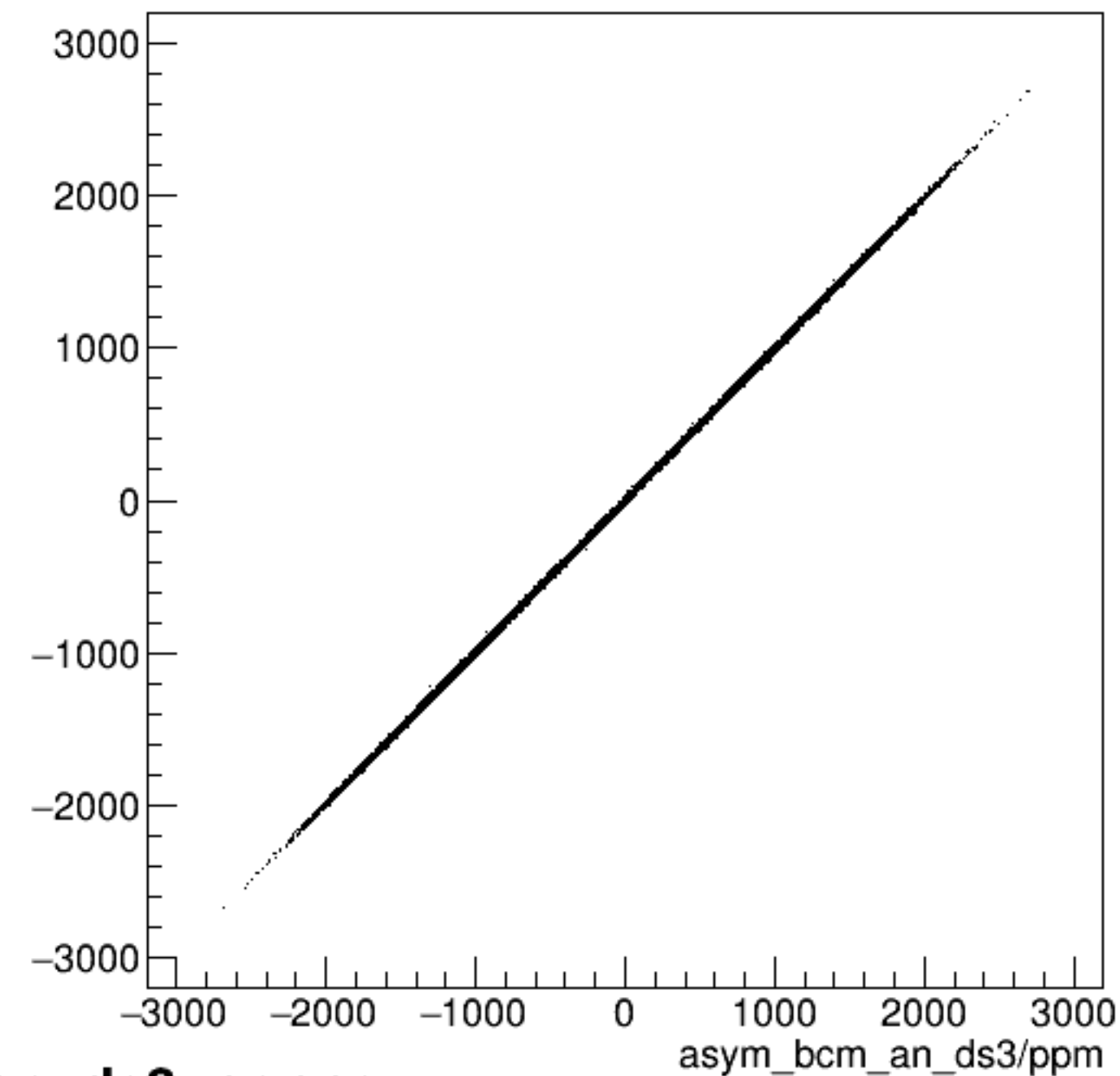
run8531_000_asym_bcm_an_ds_vs_asym_bcm_an_ds3_pr.png
