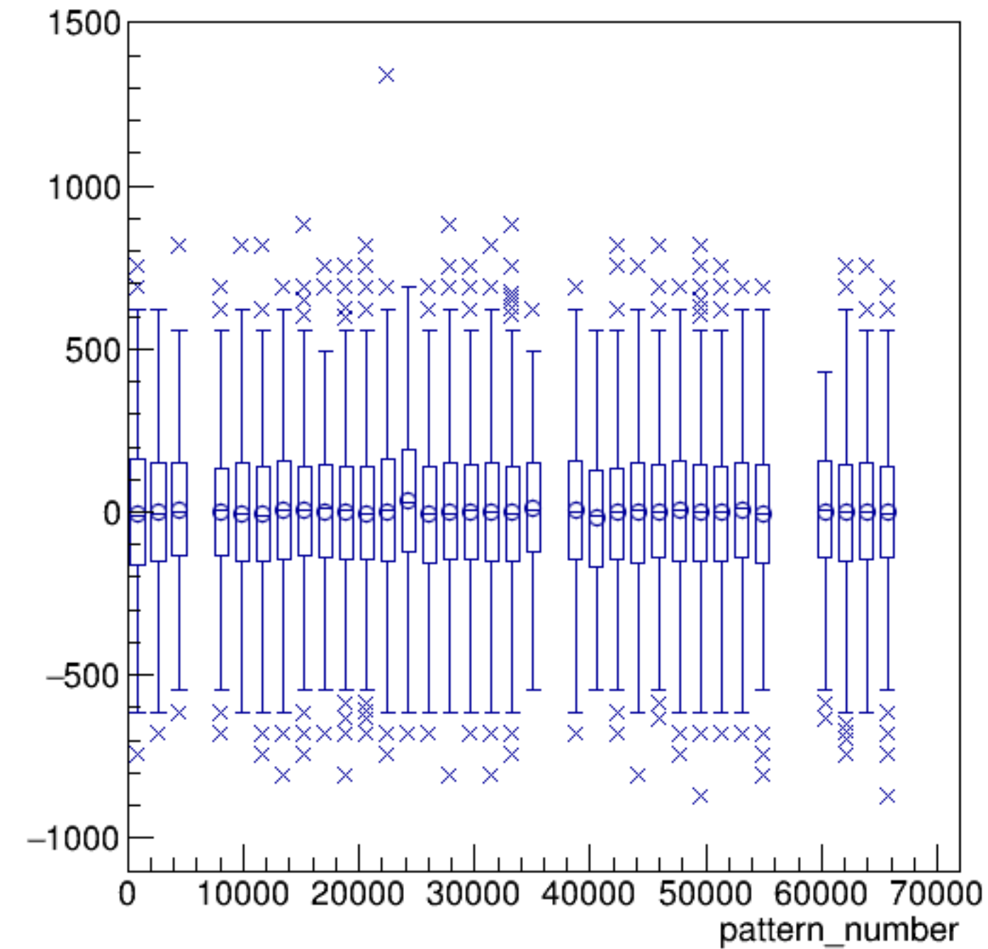
asym_bcm_dg_us/ppm:pattern_number {ErrorFlag==0}
