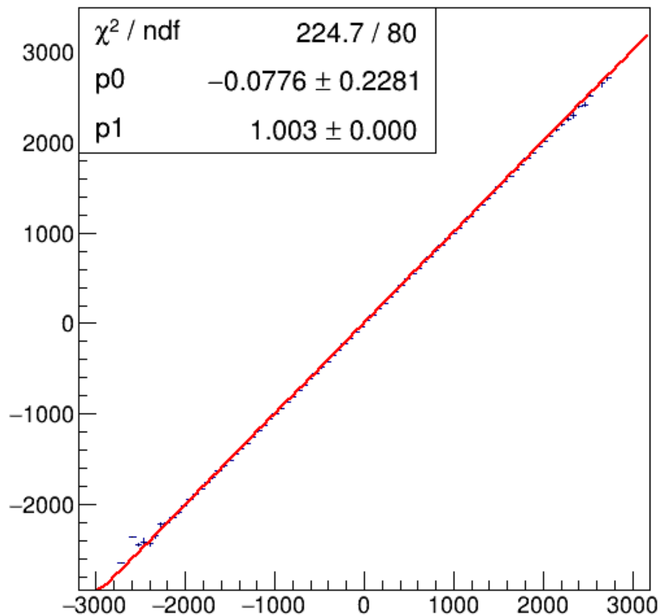
run8531_000_asym_bcm_dg_us_vs_asym_bcm_dg_ds_pr.png
