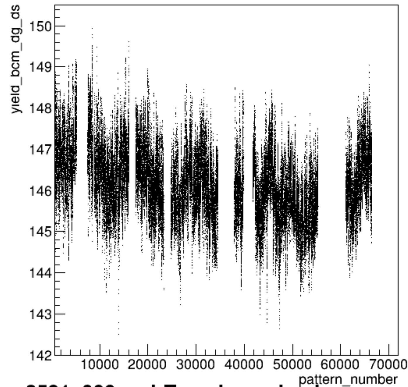
yield_bcm_dg_ds:pattern_number {ErrorFlag==0}
