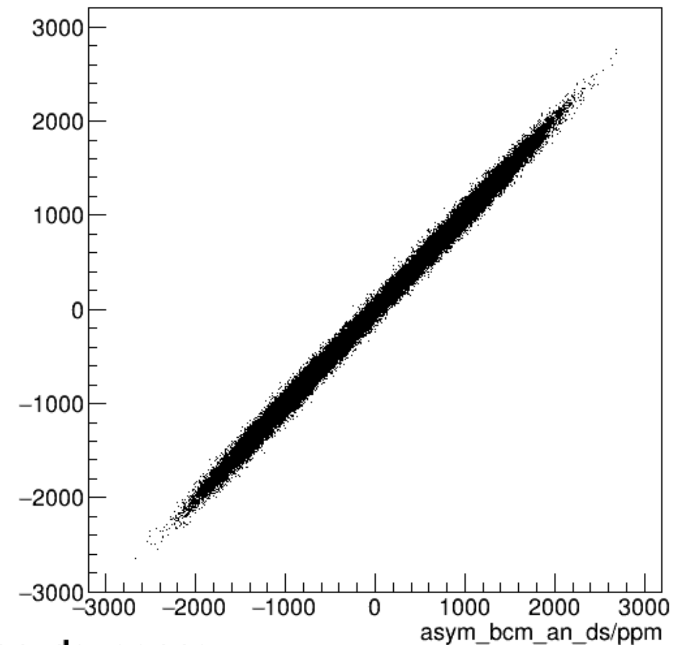
run8531_000_asym_bcm_dg_us_vs_asym_bcm_an_ds_pr.png
