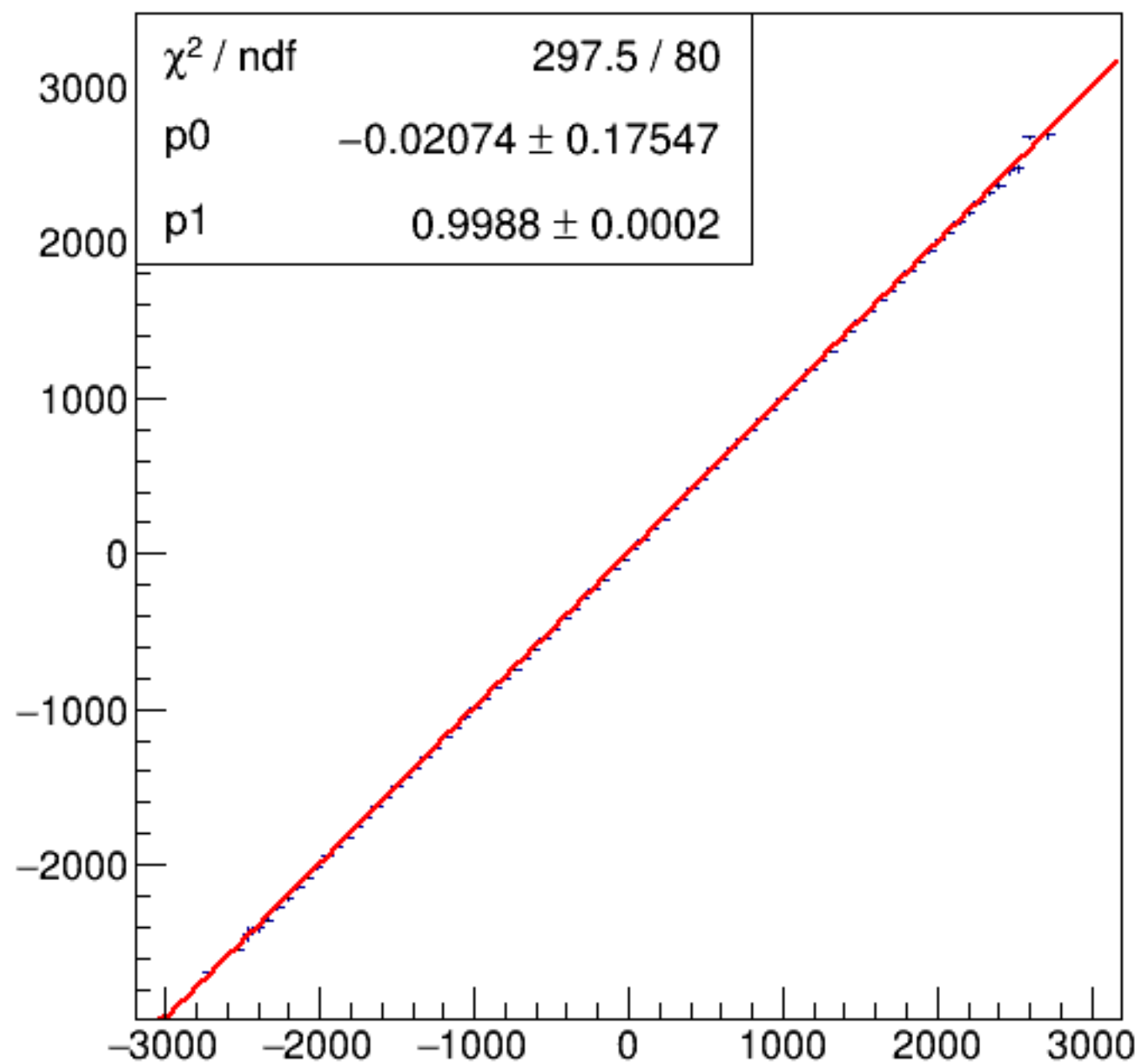
run8531_000_asym_bcm_dg_ds_vs_asym_bcm_an_us_pr.png
