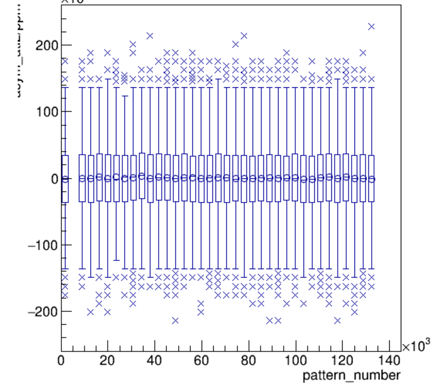
asym_atl2/ppm:pattern_number {ErrorFlag==0}
