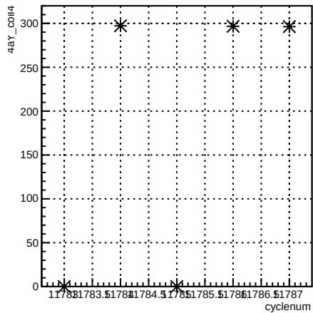
4eY_coil4:cyclenum {run == 8488}
