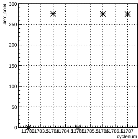
4eY_coil4:cyclenum {run == 8488}
