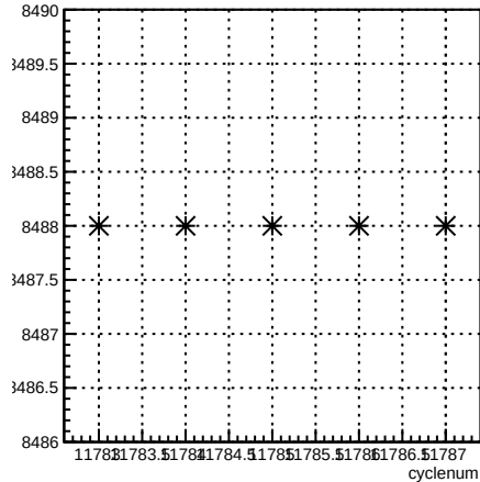
run:cyclenum {run == 8488}
