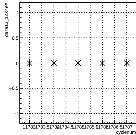
delta13_12X4eX:cyclenum {run == 8488}
