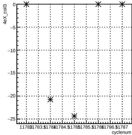
4eX_coil3:cyclenum {run == 8488}
