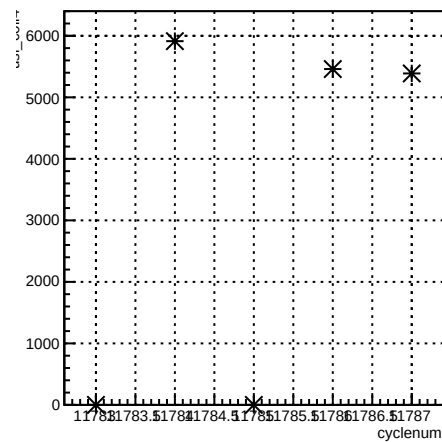
usl_coil4:cyclenum {run == 8488}
