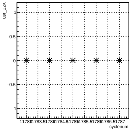
usr_12X:cyclenum {run == 8488}
