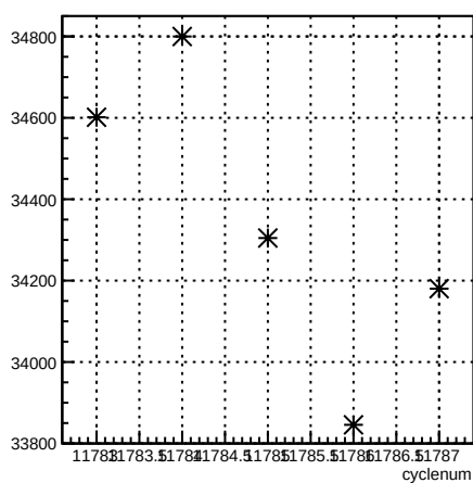
usr_coil7:cyclenum {run == 8488}
