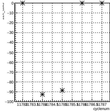
12X_coil3:cyclenum {run == 8488}
