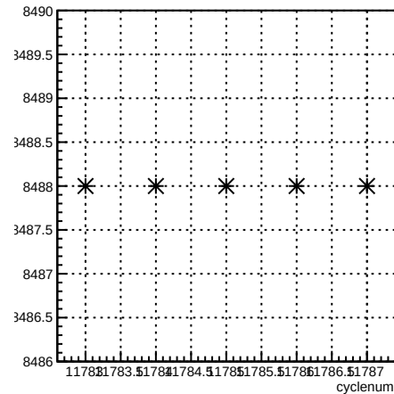
run:cyclenum {run == 8488}
