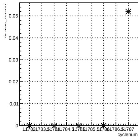
delta46_12X4eY:cyclenum {run == 8488}
