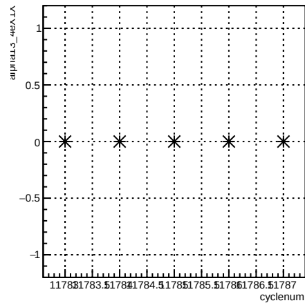
alpha13_4eX1X:cyclenum {run == 8488}
