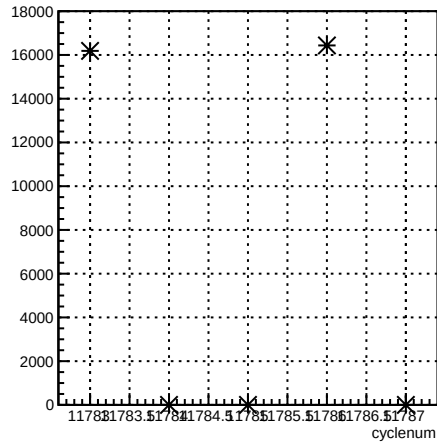
usl_coil1:cyclenum {run == 8488}
