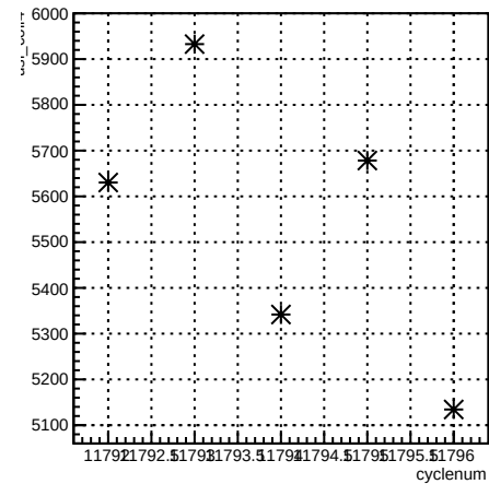
usl_coil4:cyclenum {run == 8490}
