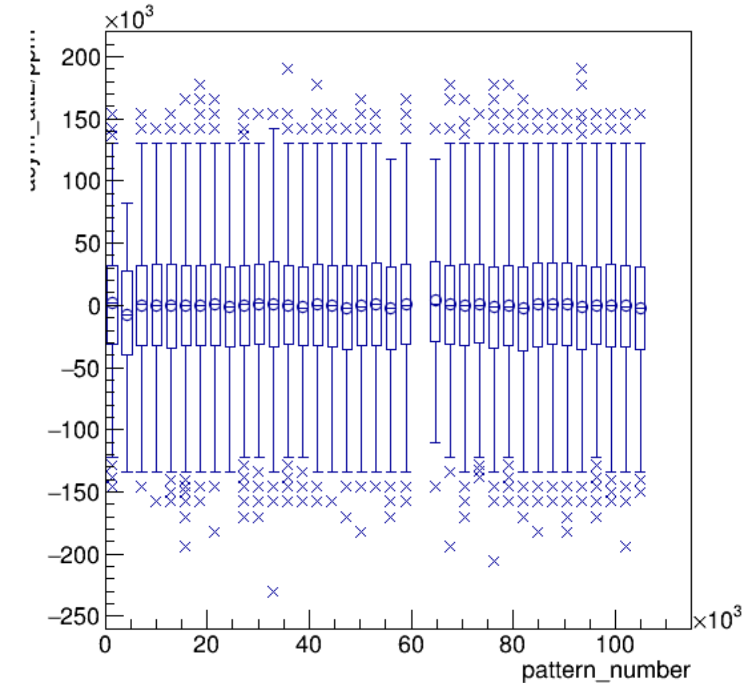
asym_atl2/ppm:pattern_number {ErrorFlag==0}
