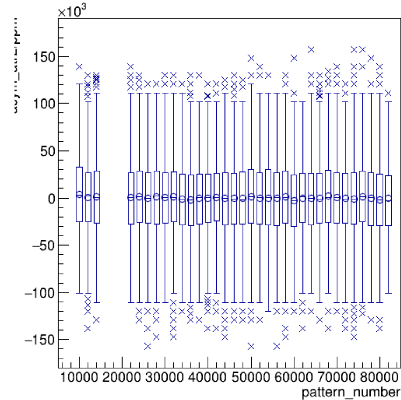
asym_atr2/ppm:pattern_number {ErrorFlag==0}
