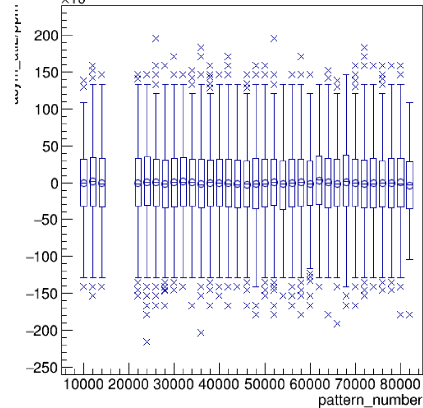
asym_atl2/ppm:pattern_number {ErrorFlag==0}
