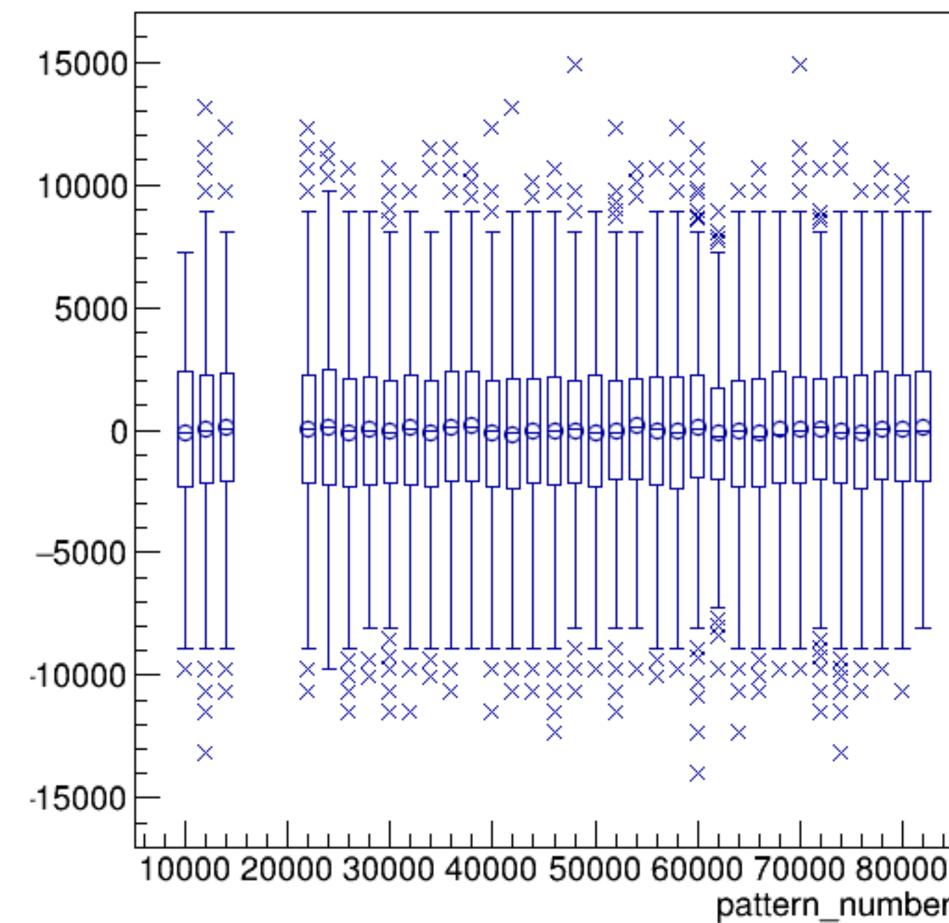
asym_atr1/ppm:pattern_number {ErrorFlag==0}
