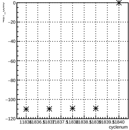
4eY_coil6:cyclenum {run == 8529}
