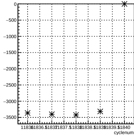
usl_coil6:cyclenum {run == 8529}
