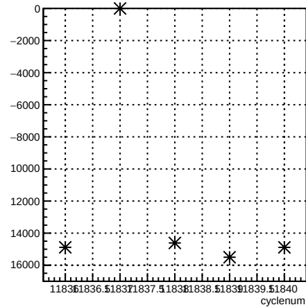
usr_coil1:cyclenum {run == 8529}
