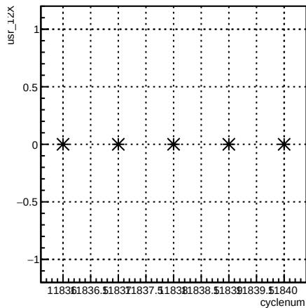
usr_12X:cyclenum {run == 8529}
