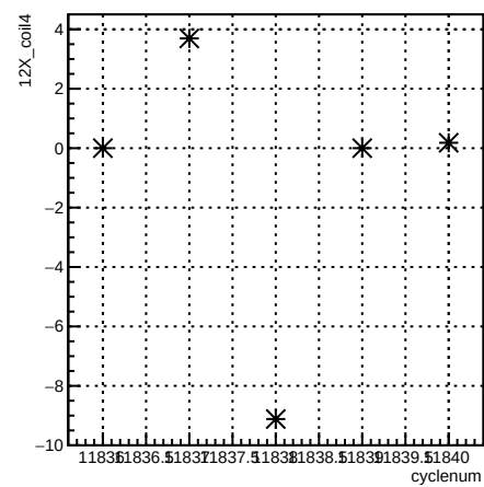
12X_coil4:cyclenum {run == 8529}
