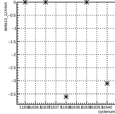
delta13_12X4eX:cyclenum {run == 8529}
