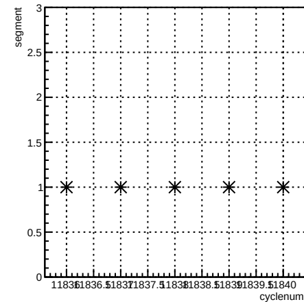
segment:cyclenum {run == 8529}
