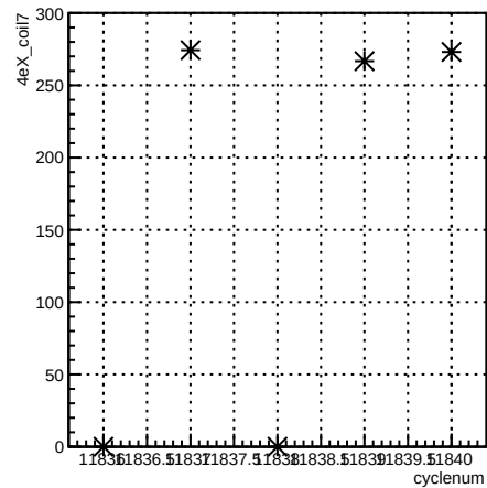
4eX_coil7:cyclenum {run == 8529}
