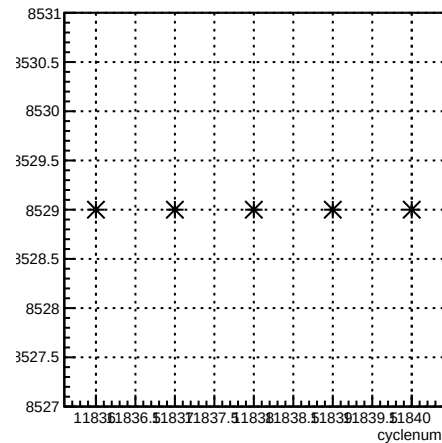
run:cyclenum {run == 8529}
