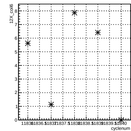
12X_coil6:cyclenum {run == 8529}
