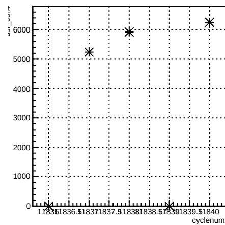
usr_coil4:cyclenum {run == 8529}
