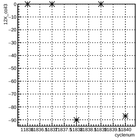
12X_coil3:cyclenum {run == 8529}
