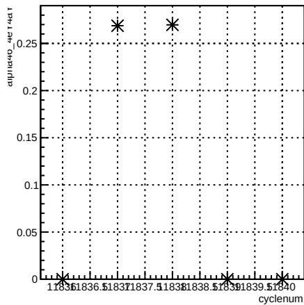
alpha46_4eY4aY:cyclenum {run == 8529}
