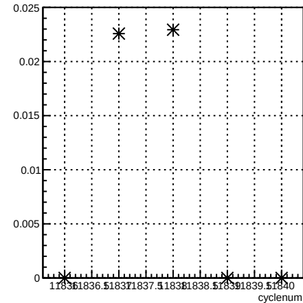
delta46_12X4eY:cyclenum {run == 8529}
