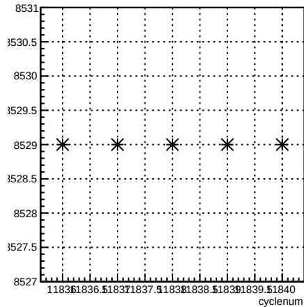
run:cyclenum {run == 8529}
