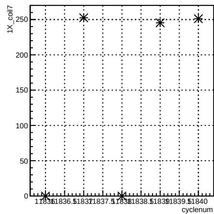
1X_coil7:cyclenum {run == 8529}
