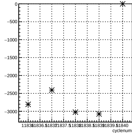
usr_coil6:cyclenum {run == 8529}
