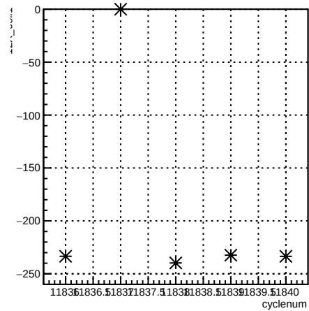
12X_coil1:cyclenum {run == 8529}
