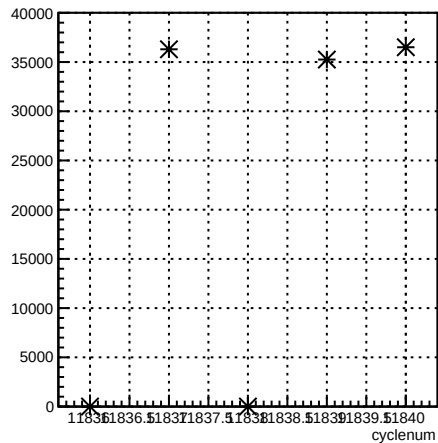
usr_coil7:cyclenum {run == 8529}
