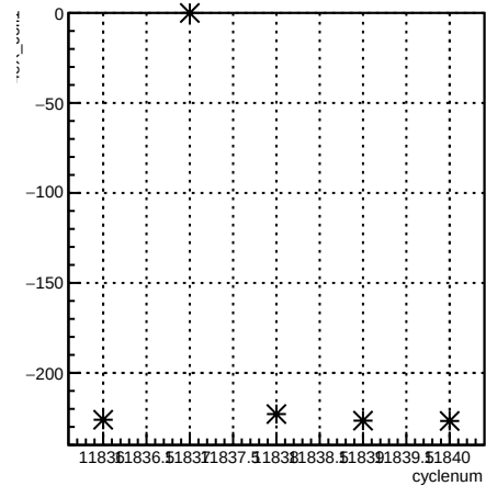
4eX_coil1:cyclenum {run == 8529}
