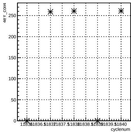
4eY_coil4:cyclenum {run == 8529}
