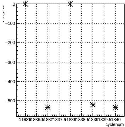
12X_coil7:cyclenum {run == 8529}
