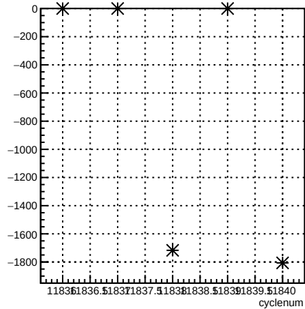
usr_coil3:cyclenum {run == 8529}
