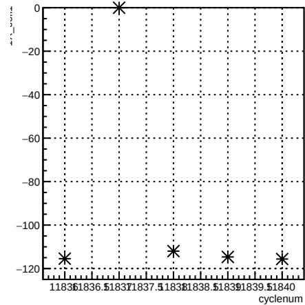
1X_coil1:cyclenum {run == 8529}
