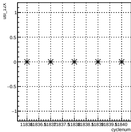
usl_12X:cyclenum {run == 8529}
