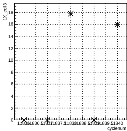
1X_coil3:cyclenum {run == 8529}
