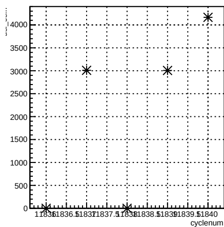
usl_coil7:cyclenum {run == 8529}
