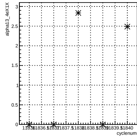
alpha13_4eX1X:cyclenum {run == 8529}
