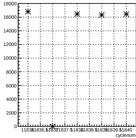
usl_coil1:cyclenum {run == 8529}
