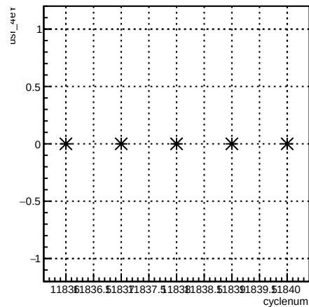
usr_4eY:cyclenum {run == 8529}
