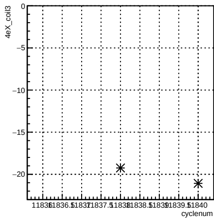
4eX_coil3:cyclenum {run == 8529}
