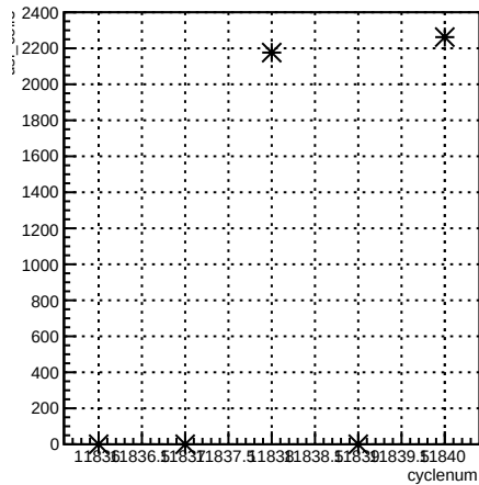
usl_coil3:cyclenum {run == 8529}
