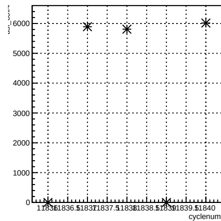
usl_coil4:cyclenum {run == 8529}
