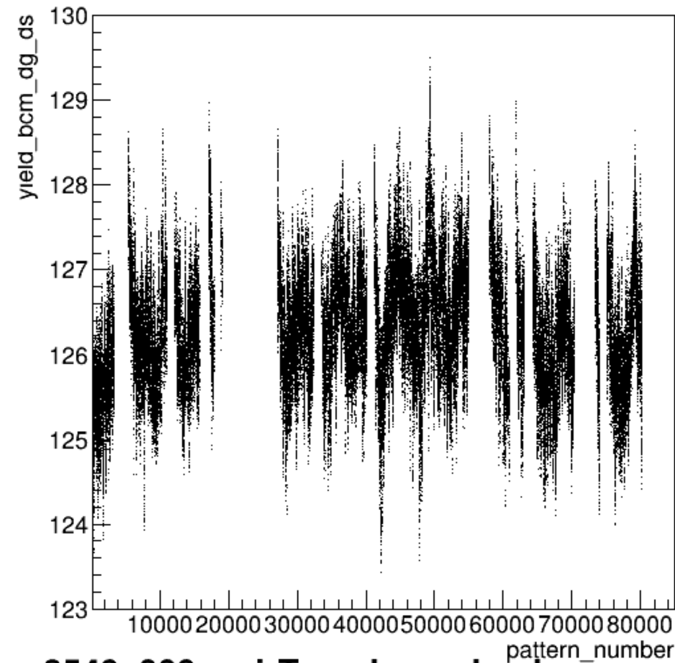
yield_bcm_dg_ds:pattern_number {ErrorFlag==0}
