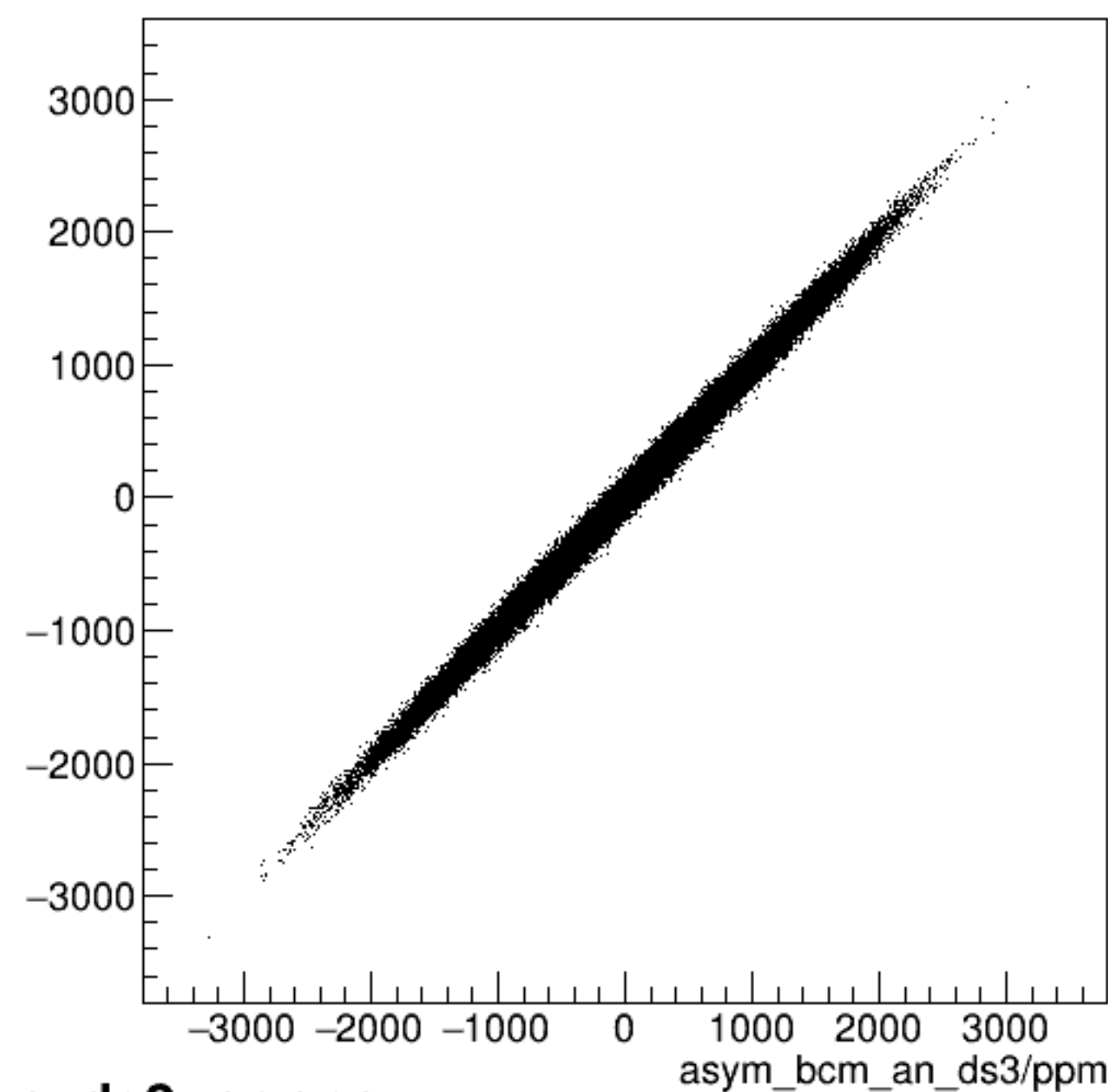
run8549_000_asym_bcm_dg_us_vs_asym_bcm_an_ds3_pr.png
