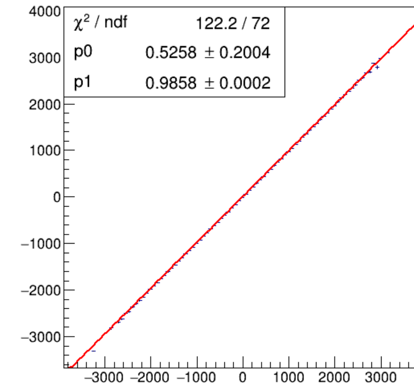
run8549_000_asym_bcm_dg_us_vs_asym_bcm_an_ds3_pr.png
