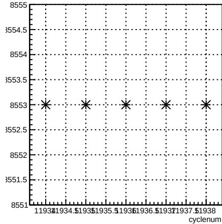
run:cyclenum {run == 8553}
