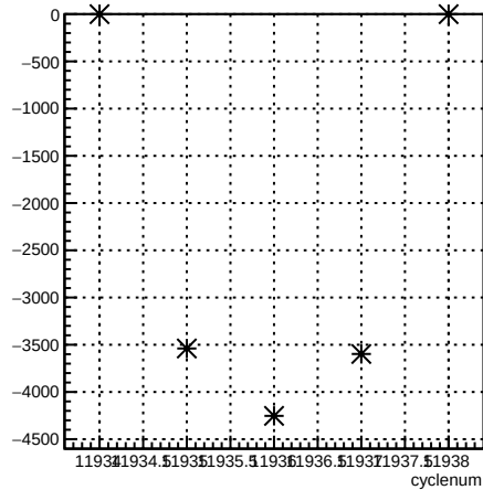
usl_coil6:cyclenum {run == 8553}
