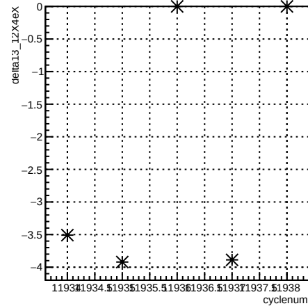
delta13_12X4eX:cyclenum {run == 8553}
