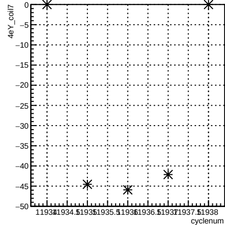
4eY_coil7:cyclenum {run == 8553}
