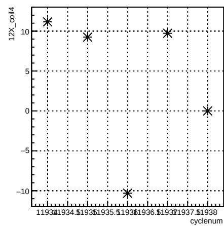
12X_coil4:cyclenum {run == 8553}
