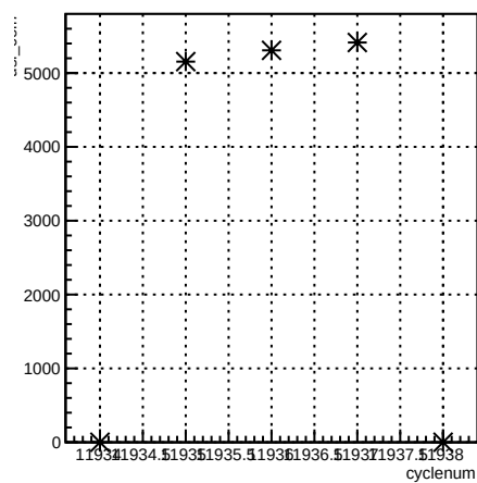
usl_coil7:cyclenum {run == 8553}
