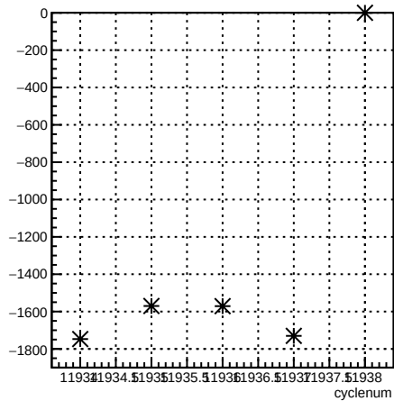
usr_coil3:cyclenum {run == 8553}
