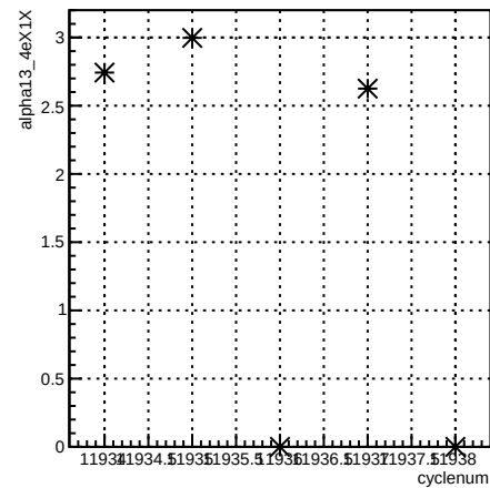
alpha13_4eX1X:cyclenum {run == 8553}
