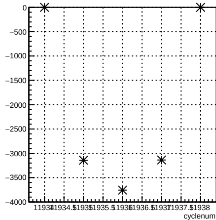
usr_coil6:cyclenum {run == 8553}
