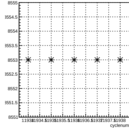
run:cyclenum {run == 8553}
