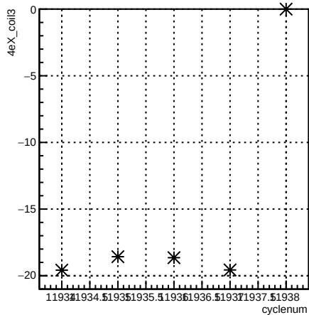
4eX_coil3:cyclenum {run == 8553}
