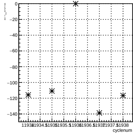
1X_coil1:cyclenum {run == 8553}
