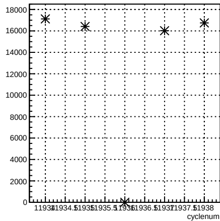
usl_coil6:cyclenum {run == 8553}
