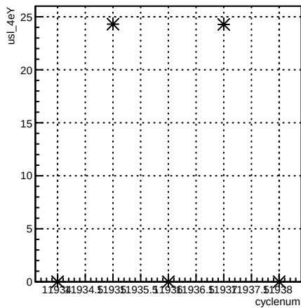
usl_4eY:cyclenum {run == 8553}
