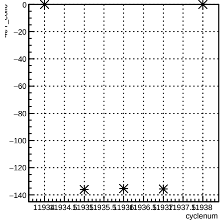
4eY_coil6:cyclenum {run == 8553}
