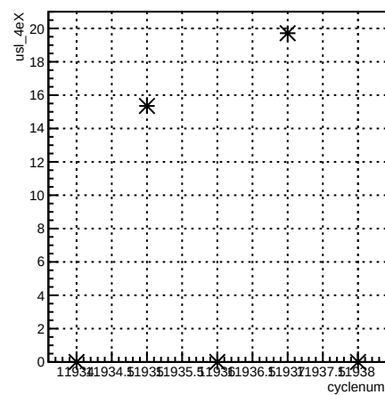
usl_4eX:cyclenum {run == 8553}
