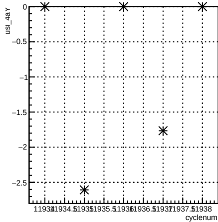
usl_4aY:cyclenum {run == 8553}
