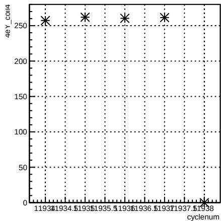
4eY_coil4:cyclenum {run == 8553}
