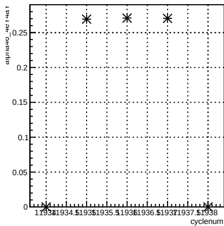
alpha46_4eY4aY:cyclenum {run == 8553}
