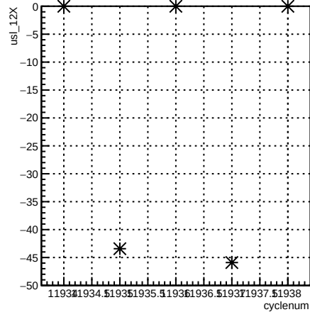
usl_12X:cyclenum {run == 8553}
