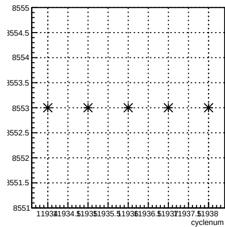
run:cyclenum {run == 8553}
