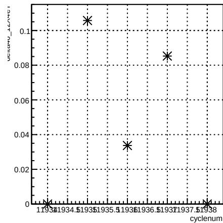
delta46_12X4eY:cyclenum {run == 8553}
