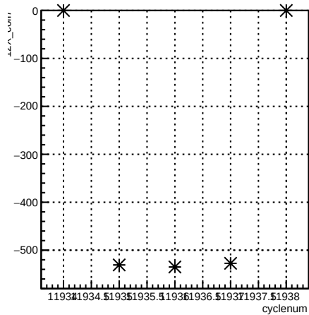
12X_coil7:cyclenum {run == 8553}
