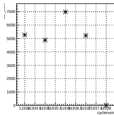
usr_coil4:cyclenum {run == 8553}
