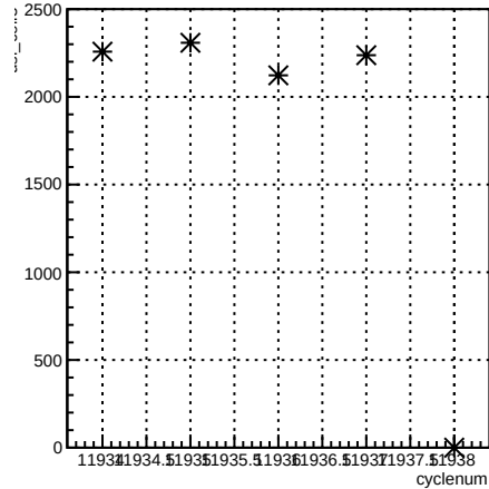
usl_coil7:cyclenum {run == 8553}
