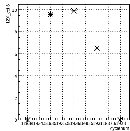
12X_coil6:cyclenum {run == 8553}
