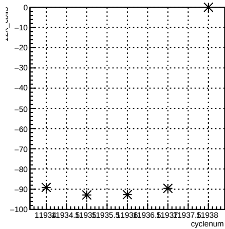
12X_coil3:cyclenum {run == 8553}
