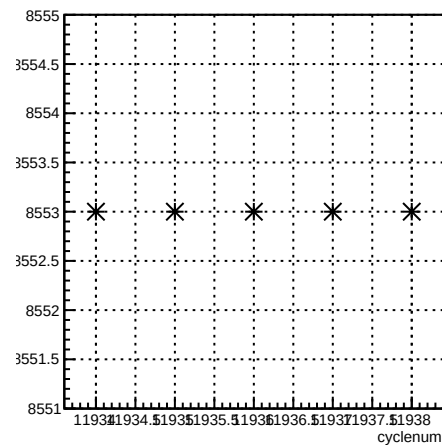
run:cyclenum {run == 8553}
