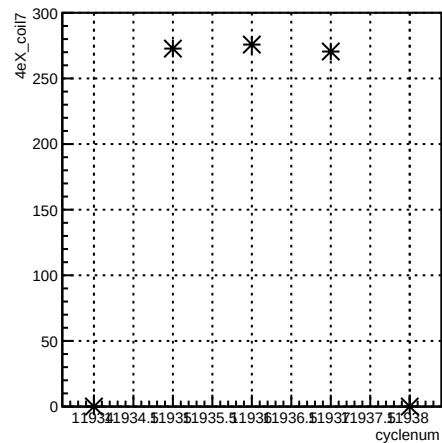
4eX_coil7:cyclenum {run == 8553}
