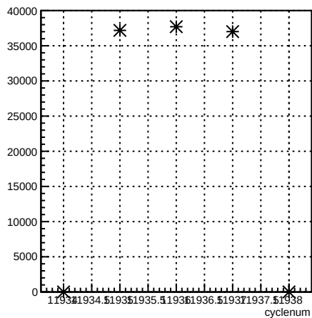
usr_coil7:cyclenum {run == 8553}
