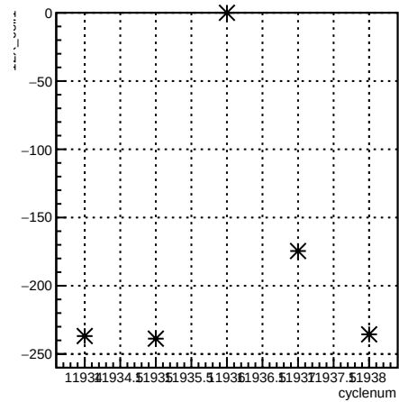
12X_coil1:cyclenum {run == 8553}
