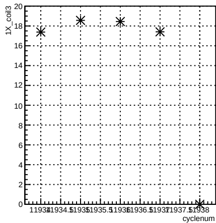
1X_coil3:cyclenum {run == 8553}
