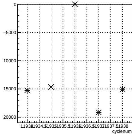
usr_coil1:cyclenum {run == 8553}
