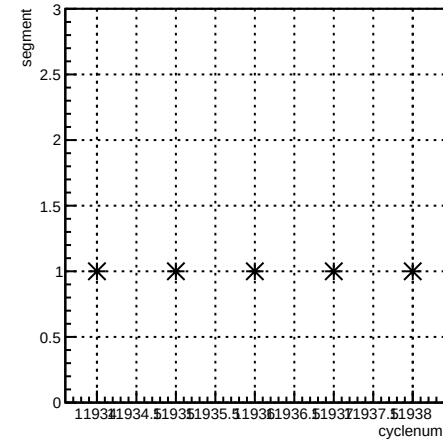
segment:cyclenum {run == 8553}
