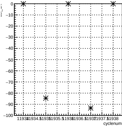
usl_1X:cyclenum {run == 8553}
