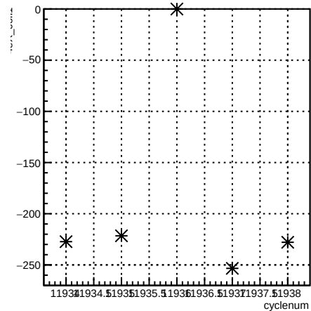
4eX_coil1:cyclenum {run == 8553}
