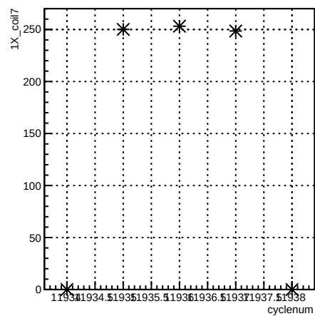
1X_coil7:cyclenum {run == 8553}
