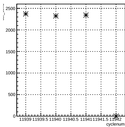
usl_coil3:cyclenum {run == 8554}
