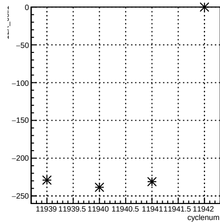
12X_coil1:cyclenum {run == 8554}
