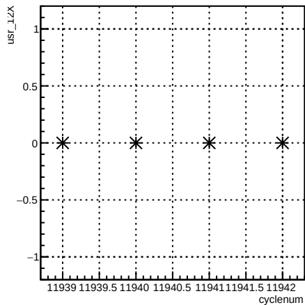
usr_12X:cyclenum {run == 8554}
