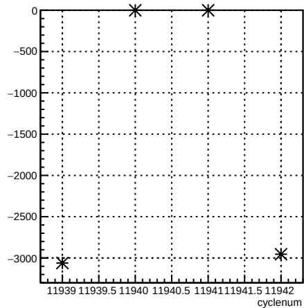
usr_coil6:cyclenum {run == 8554}
