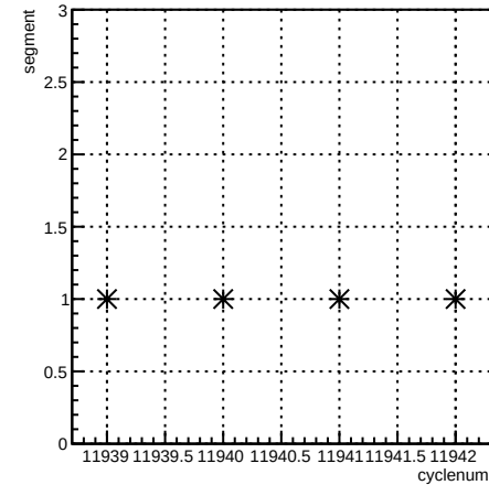
segment:cyclenum {run == 8554}
