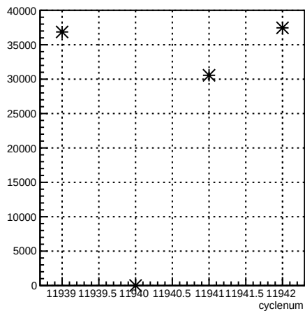
usr_coil7:cyclenum {run == 8554}
