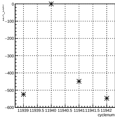
12X_coil7:cyclenum {run == 8554}
