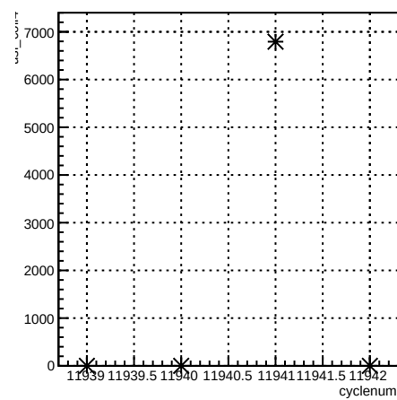
usl_coil4:cyclenum {run == 8554}
