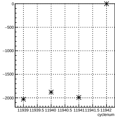
usr_coil3:cyclenum {run == 8554}
