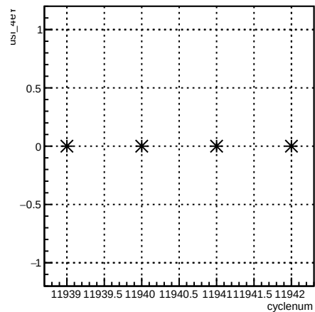
usl_4eY:cyclenum {run == 8554}
