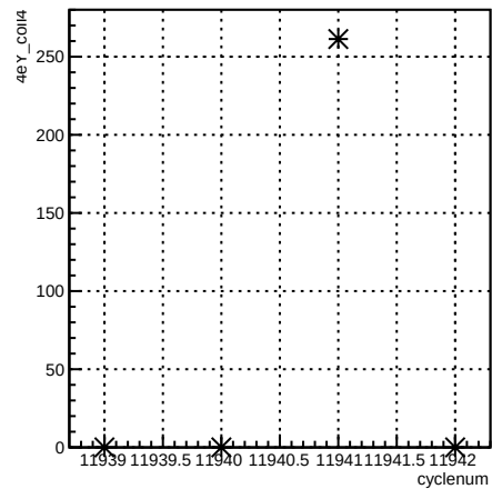
4eY_coil4:cyclenum {run == 8554}
