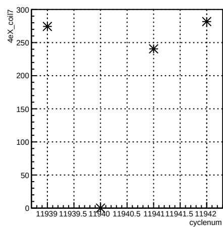
4eX_coil7:cyclenum {run == 8554}
