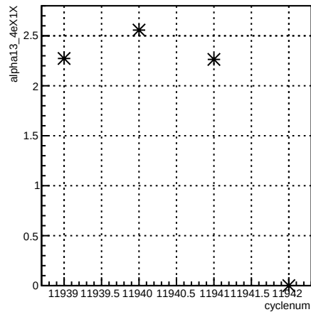
alpha13_4eX1X:cyclenum {run == 8554}
