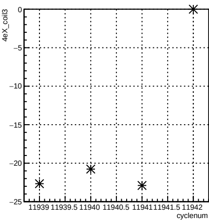
4eX_coil3:cyclenum {run == 8554}
