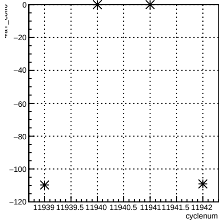
4eY_coil6:cyclenum {run == 8554}
