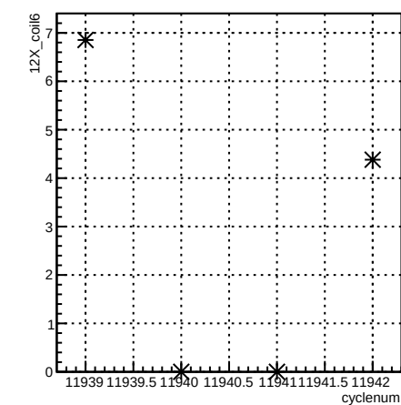
12X_coil6:cyclenum {run == 8554}
