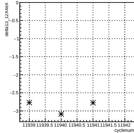
delta13_12X4eX:cyclenum {run == 8554}
