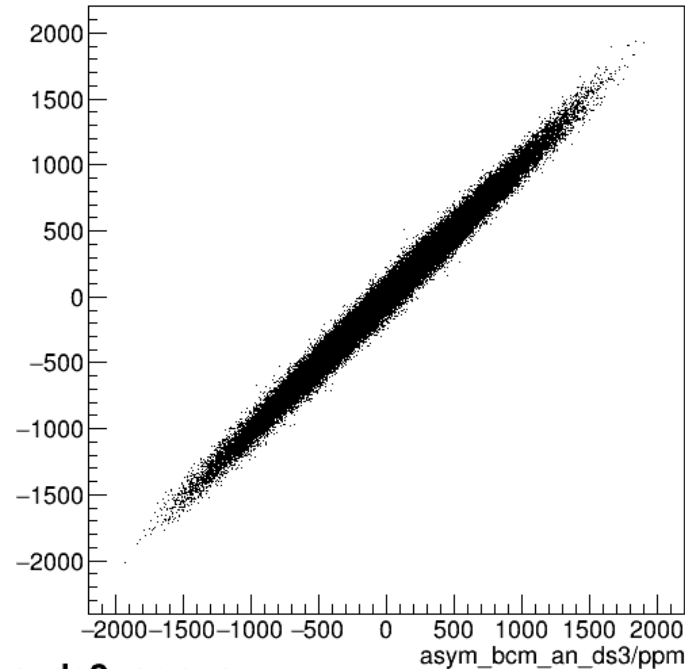
run6344_000_asym_bcm_dg_us_vs_asym_bcm_an_ds3_pr.png
