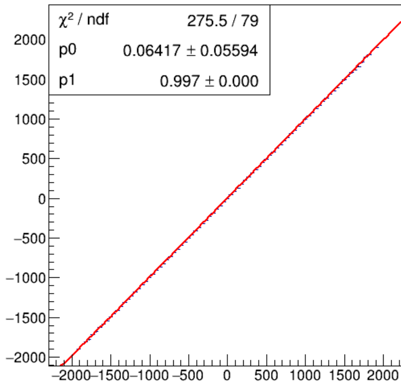
run6344_000_asym_bcm_an_ds_vs_asym_bcm_an_ds3_pr.png
