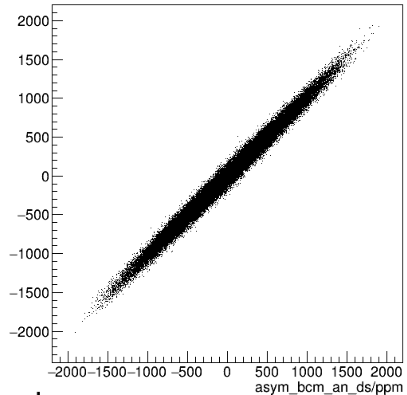
run6344_000_asym_bcm_dg_us_vs_asym_bcm_an_ds_pr.png
