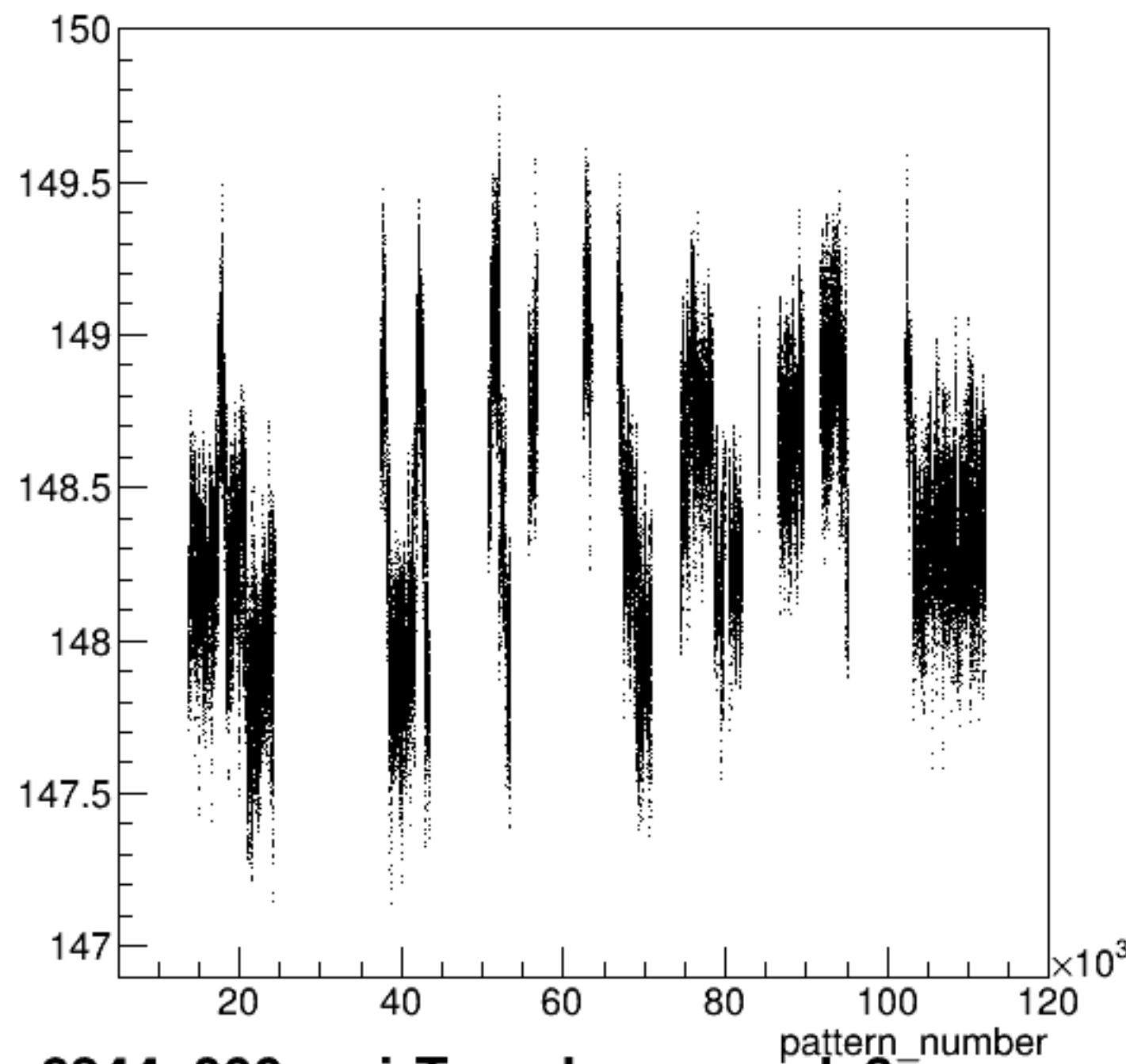
yield_bcm_an_ds3:pattern_number {ErrorFlag==0}
