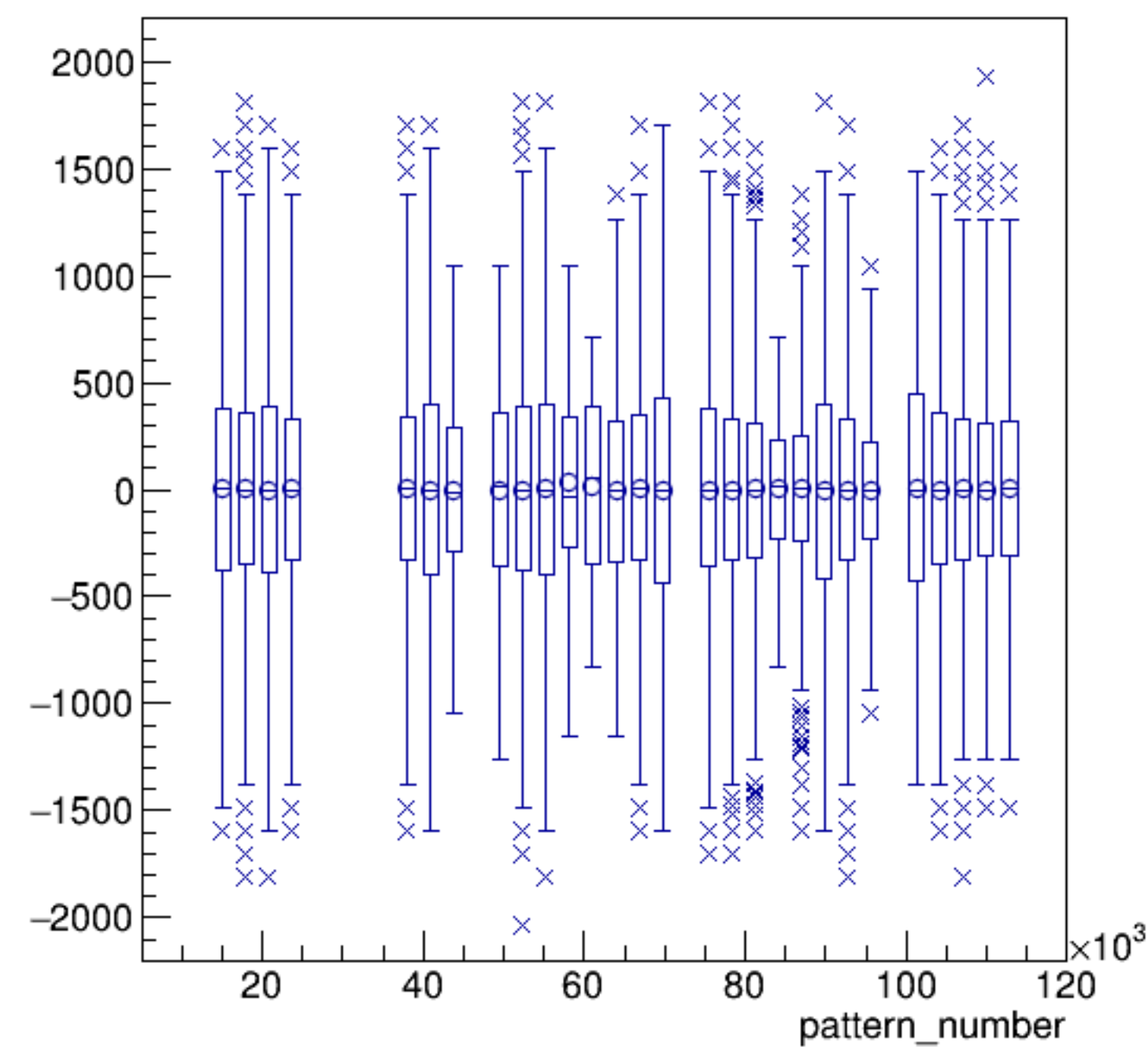
asym_bcm_an_us/ppm:pattern_number {ErrorFlag==0}
