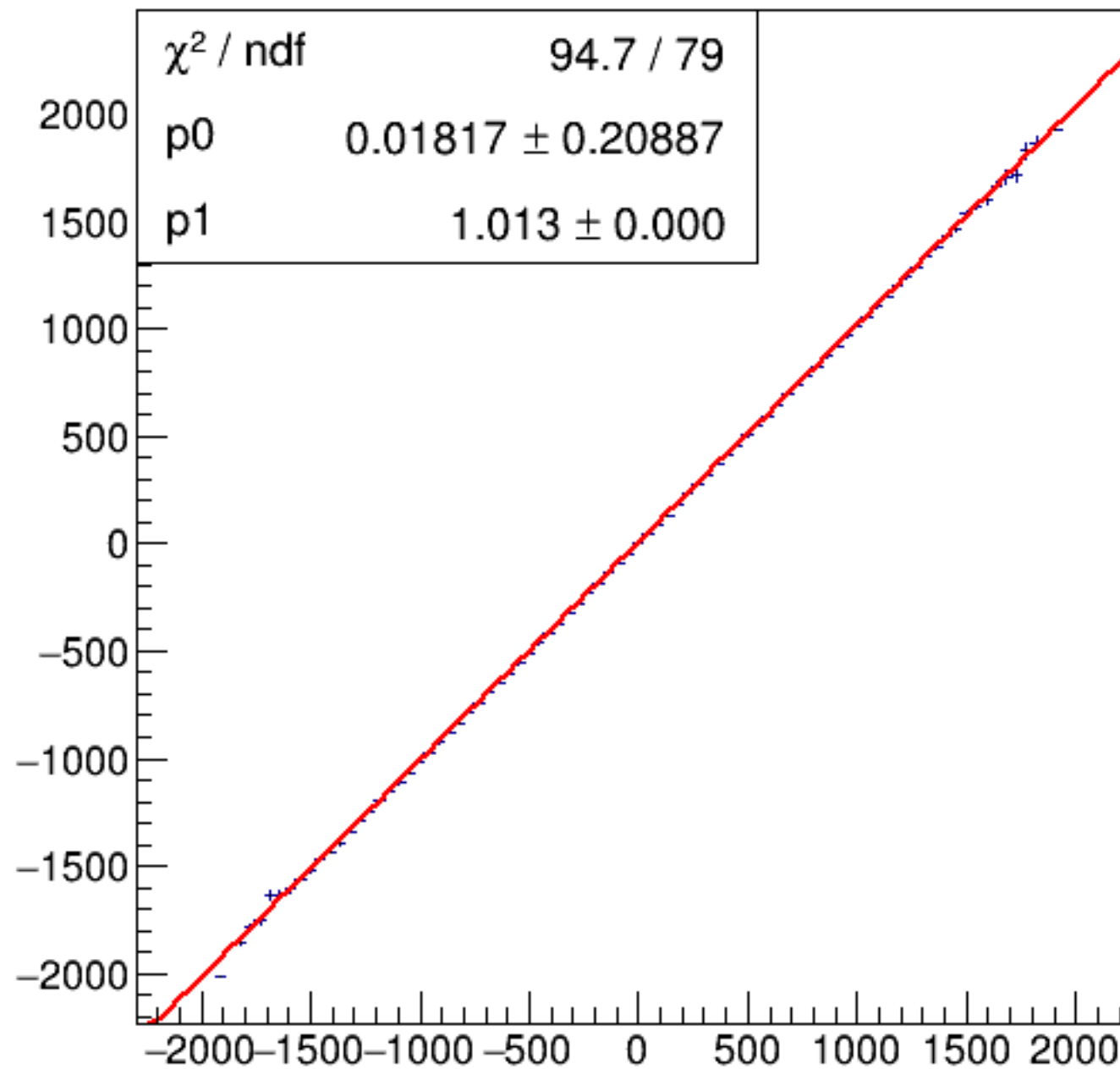
run6344_000_asym_bcm_dg_us_vs_asym_bcm_an_ds3_pr.png
