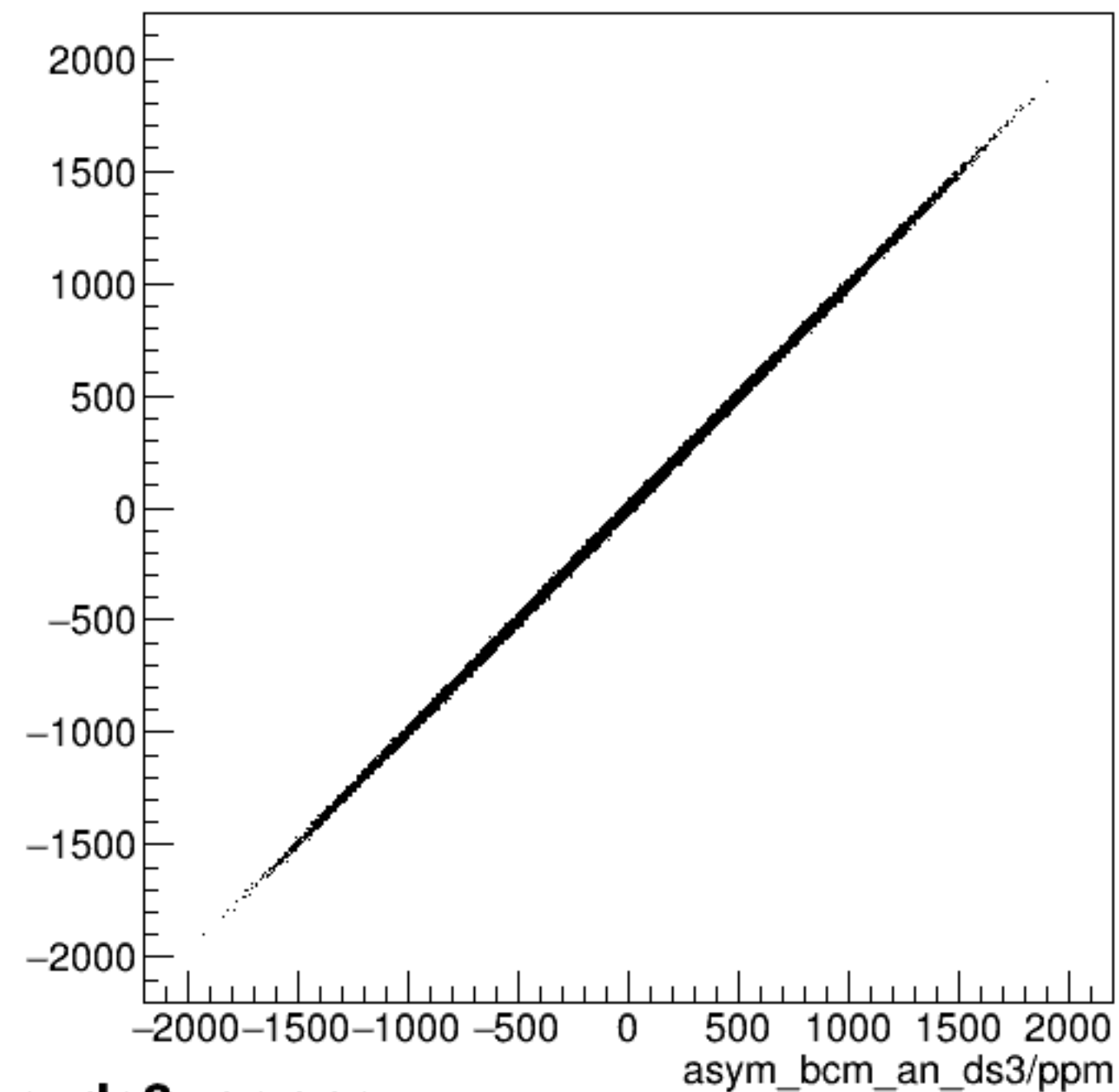
run6344_000_asym_bcm_an_ds_vs_asym_bcm_an_ds3_pr.png
