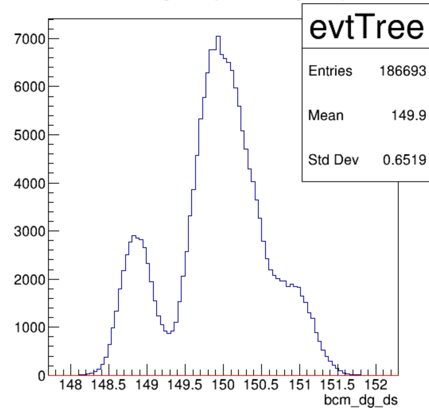
bcm_dg_ds {ErrorFlag==0}
