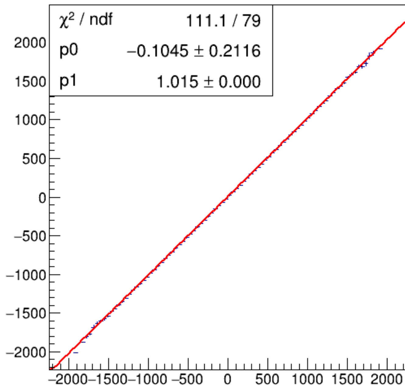
run6344_000_asym_bcm_dg_us_vs_asym_bcm_an_ds_pr.png
