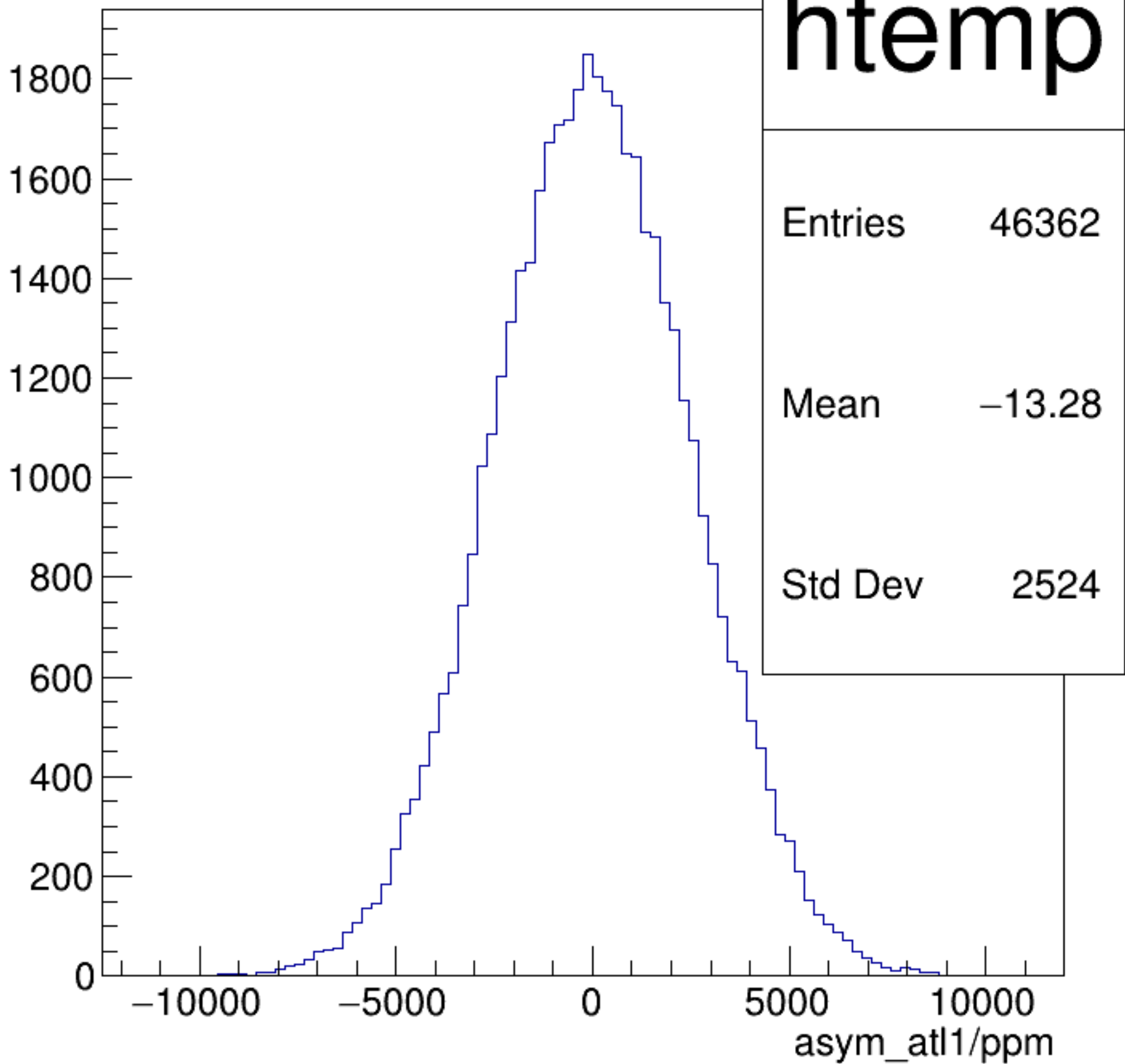
asym_atl1/ppm {ok_cut}
