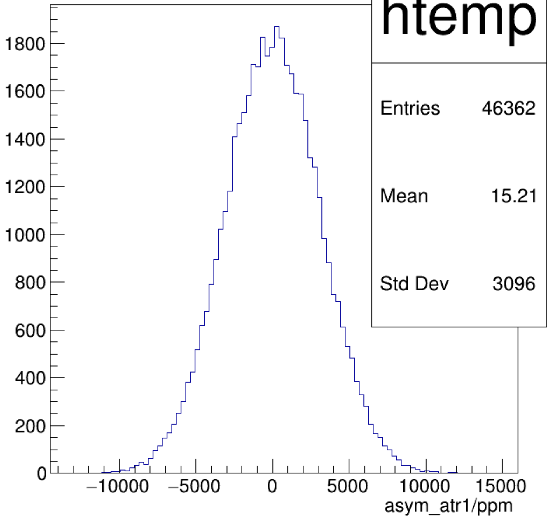
asym_atr1/ppm {ok_cut}
