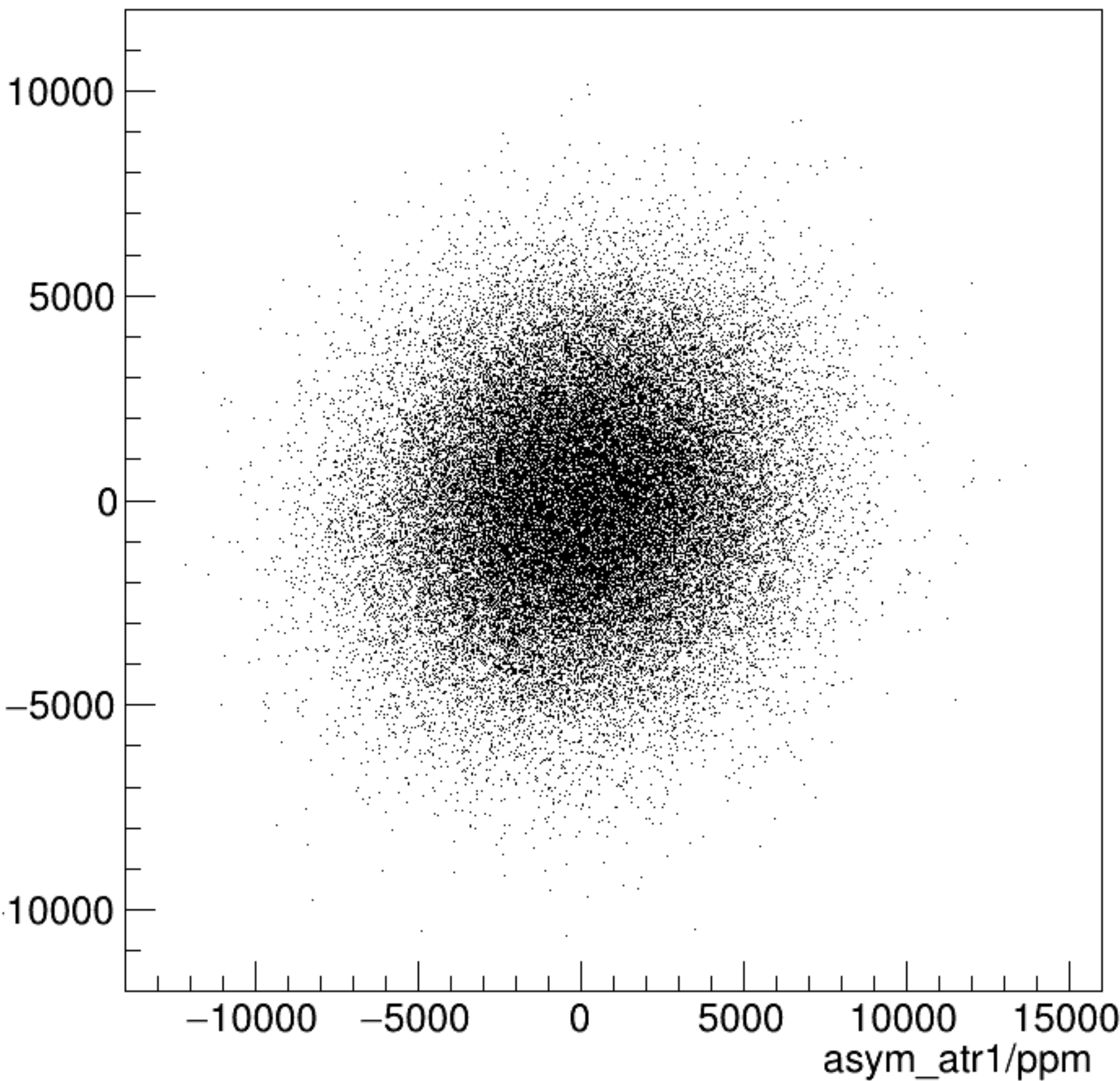
asym_atl1/ppm:asym_atr1/ppm {ok_cut}
