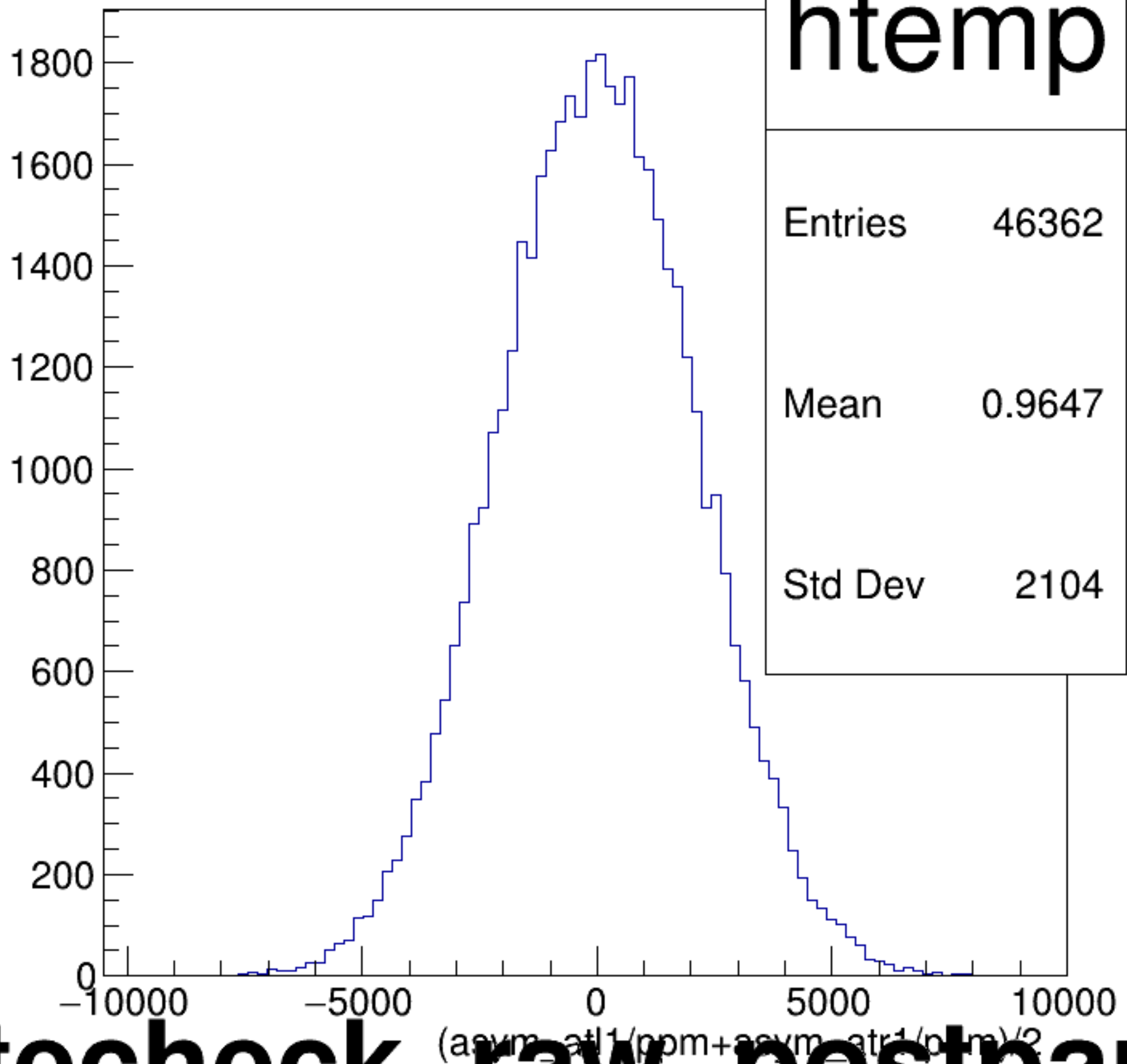
(asym_atl1/ppm+asym_atr1/ppm)/2 {ok_cut}
