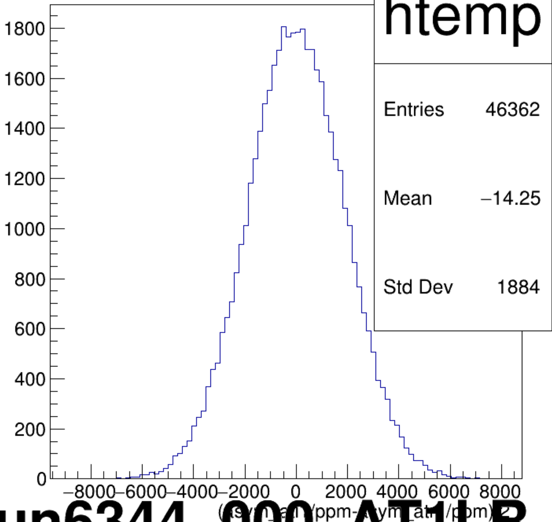
(asym_atl1/ppm-asym_atr1/ppm)/2 {ok_cut}
