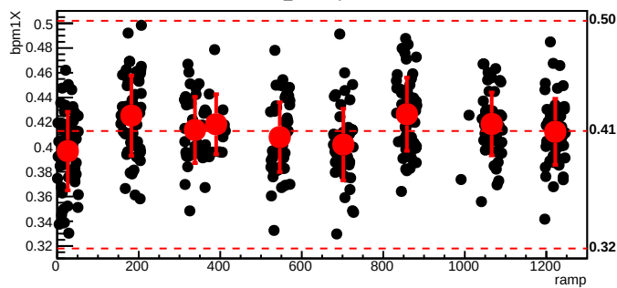
bmod_trim4,cyc=6010
