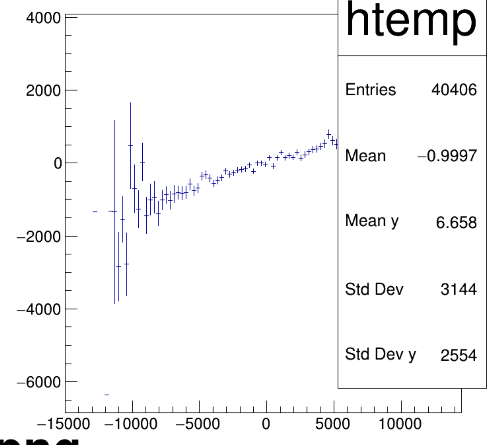
asym_atl1/ppm:asym_atr1/ppm {ok_cut}
